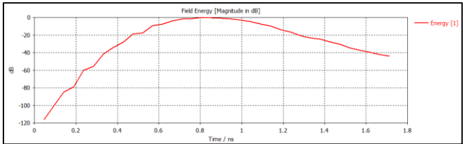
Figure 13 Field Energy for Monopole Antenna
