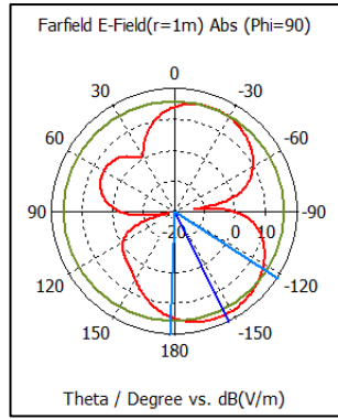
Figure 14 E-Field of Monopole with AMC
