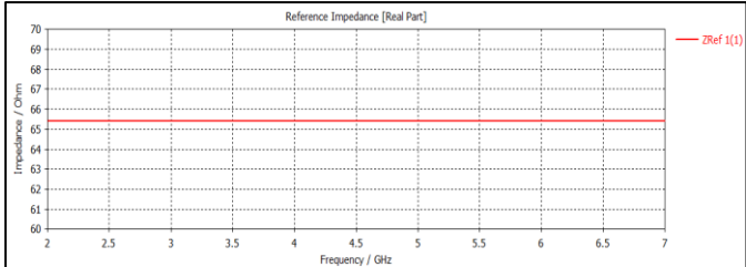
Figure 10 Ref Impdace of monopole with AMC
