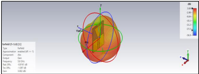
Figure 9 Gain of Monopole Antenna
