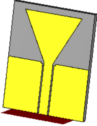
Figure 1: Coplanar Waveguide fed monopole
