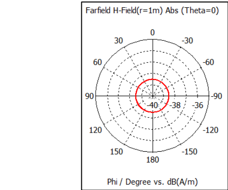
Figure 10: H field of Monopole Antenna
