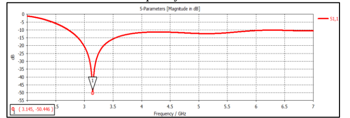
Figure 5: S (1,1) parameter of Monopole Antenna with AMC
