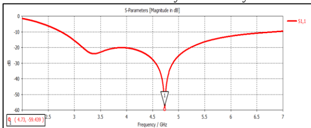
Figure 4: S (1,1) parameter of Monopole Antenna
