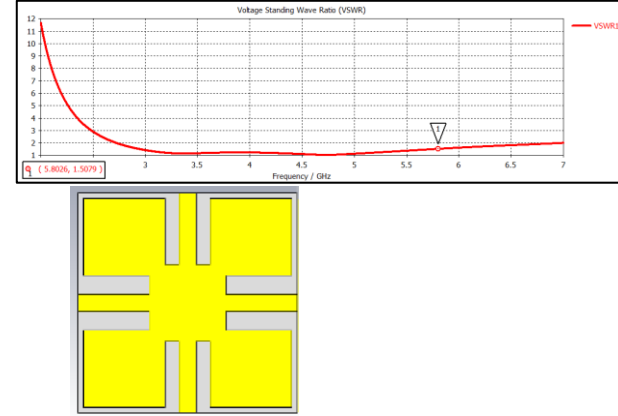
Figure 2: AMC Design
