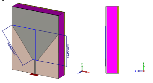
Figure 2: Antenna-2 Structure
