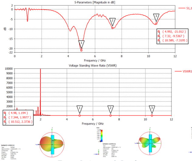
Figure 5: Antenna 2, Results
