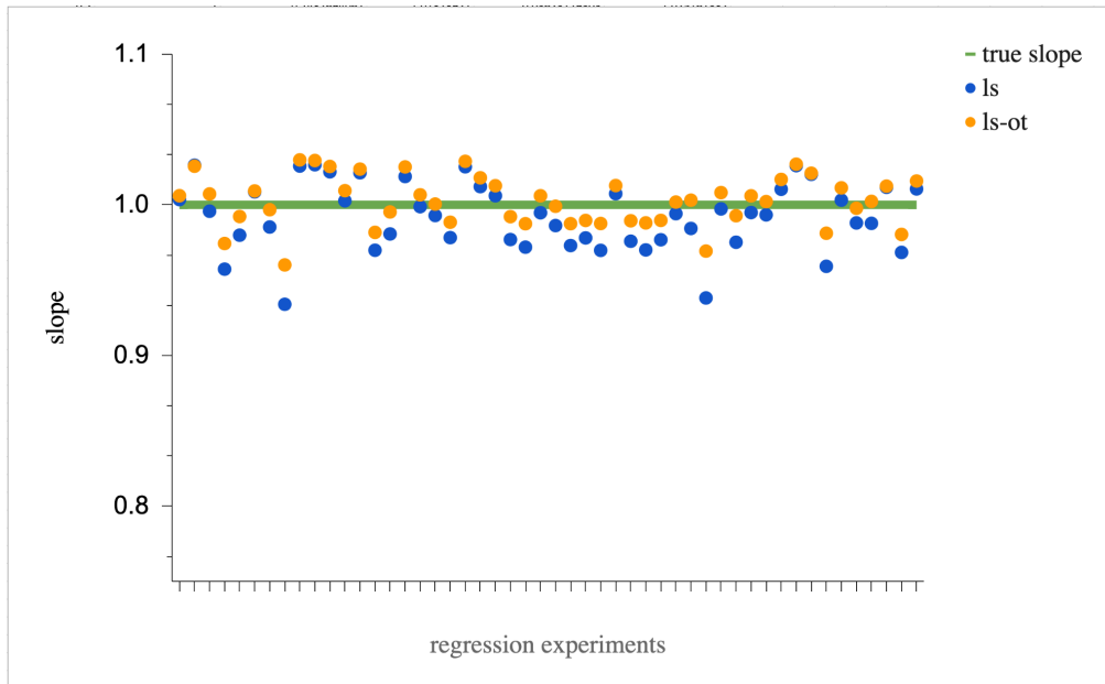
Figure 5: OLS estimated Beta, LS-OT fit using OT transportation plan and chain rule as gradient, and the true slope (data generator parameter)
