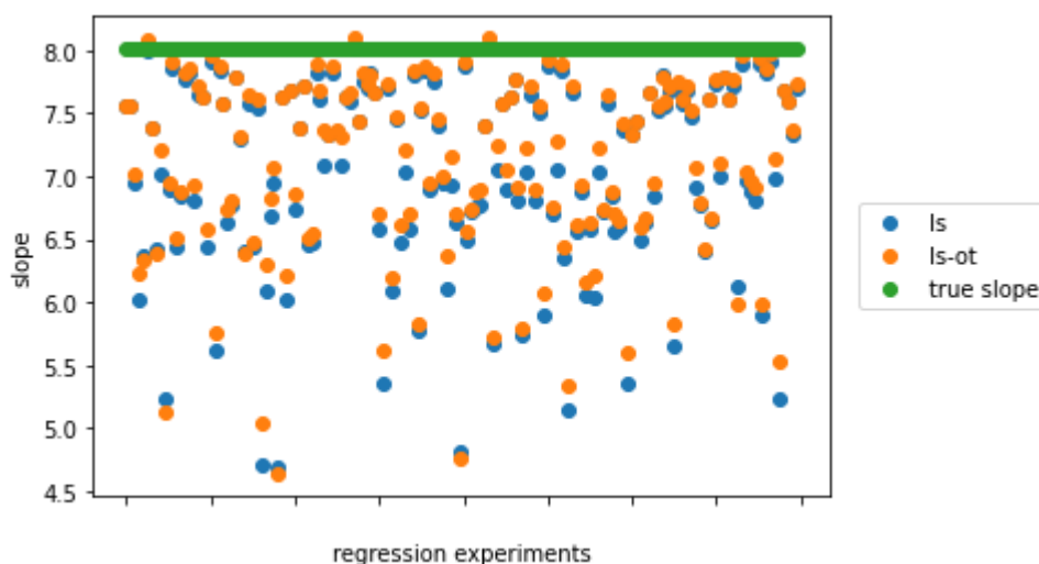
Figure 4: ls shows OLS estimated Beta, LS-OT fit using automatic differentiation, and the true slope (generator parameter) The results of the second method are shown in Figure 2, using OT transportation plan based gradient. Here, the second method brings significant improvement on
