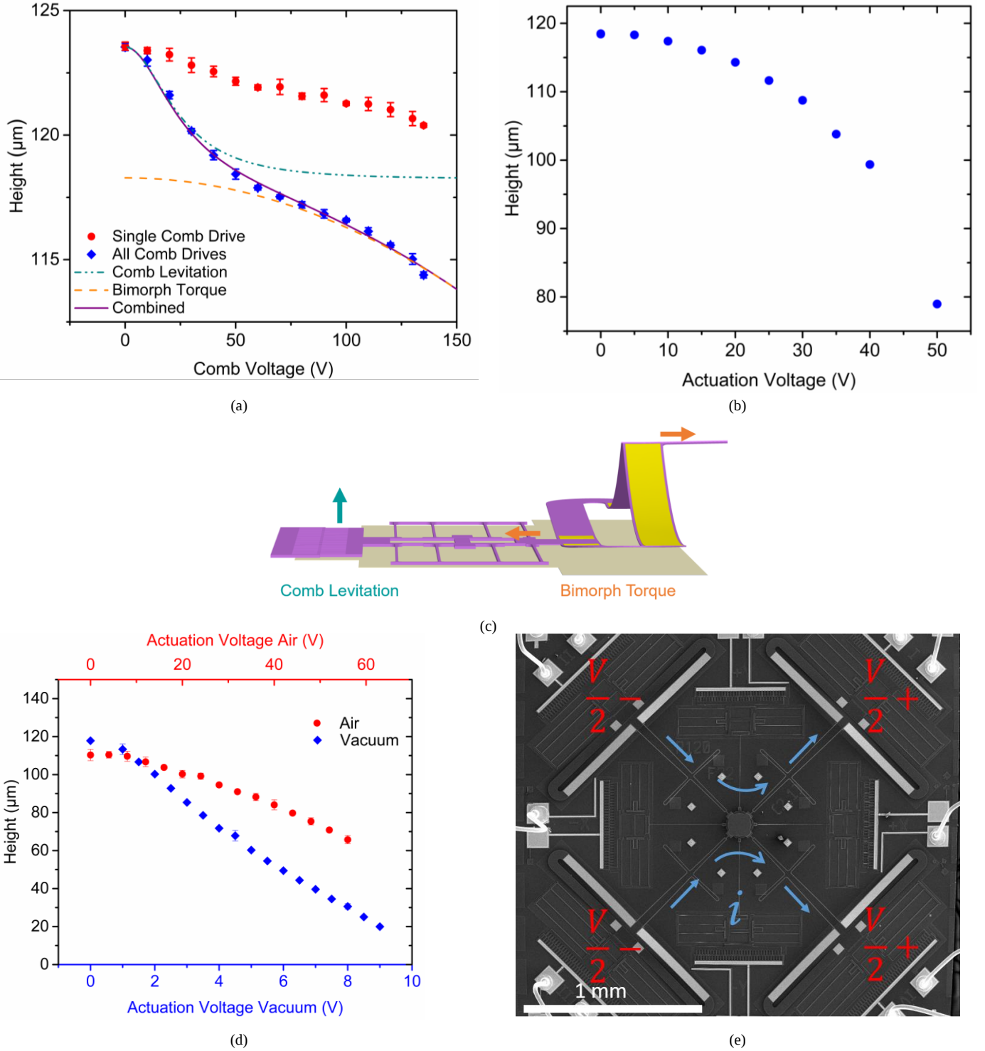
Fig. 4. Three methods of vertical actuation. (a) Plot of actuating all of the comb drives simultaneously also included is a fit based on two different mechanisms which are plotted individually and combined. (b) Plot of actuating by putting a potential difference between the plate and the substrate and electrostatically pulling the plate down. The plate pulled in at about one third the initial separation. (c) A diagram of one quadrant of the device showing the two mechanisms used to fit the data in (a). (d) Plot of actuating the thermal bimorphs by running a current through the tethers and folded beam suspensions in both air and vacuum. (e) SEM image of the device with the potentials and currents used in (d) labeled. The potential difference plotted in (d) is the total potential difference.
