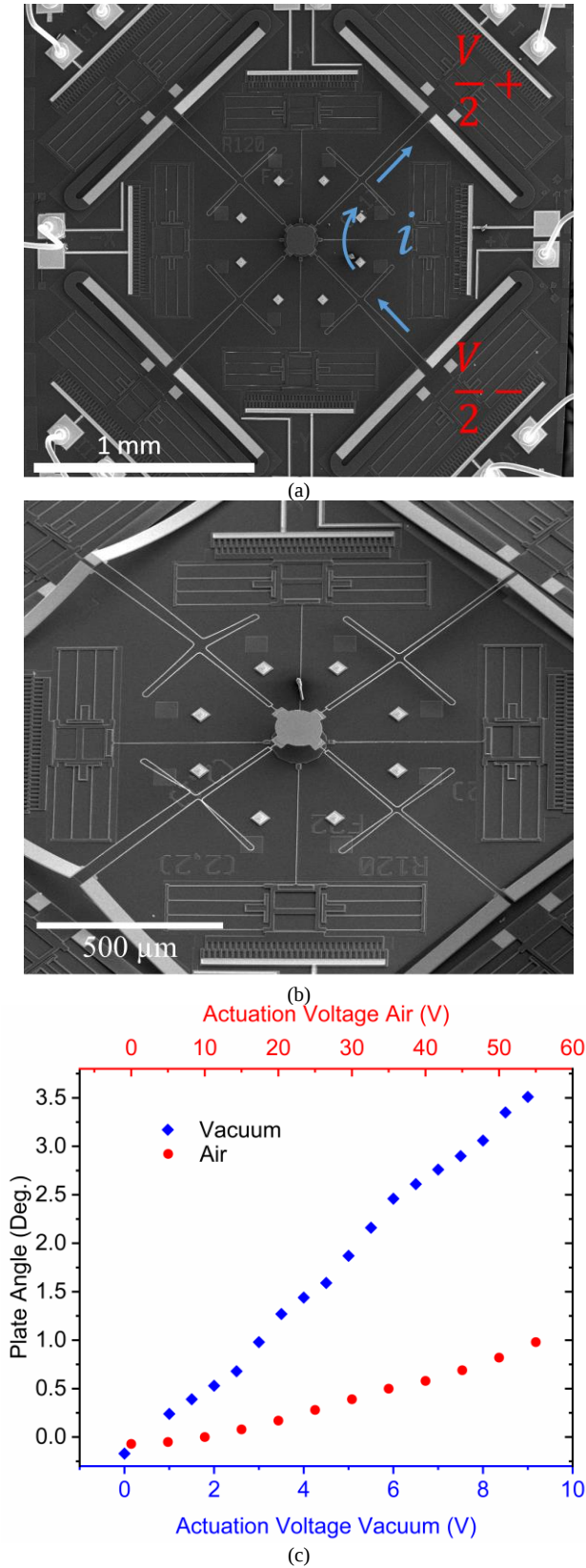
Fig. 5. Shown is the tip/tilt operation. (a) An SEM image of the device with the potentials and current paths used in tip/tilt operation labeled. (b) SEM image of the device at maximum tilt in vacuum. The bimorphs on the right are near the substrate. (c) Plot of the tilt angle versus voltage in vacuum and air. The actuation voltage is the total potential difference between V+ and V- in (a).
