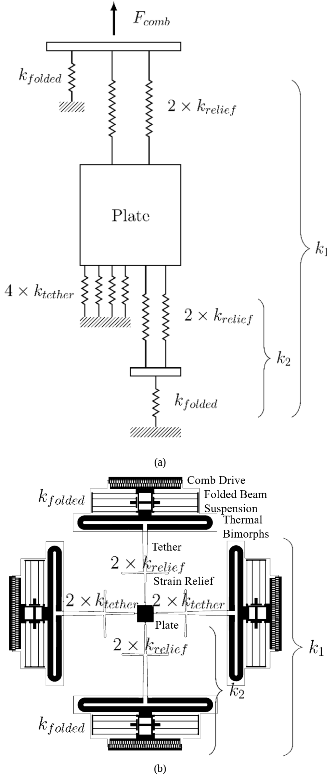
Fig. 2. Diagrams of the mechanics of the device. (a) Diagram of a spring model of the device, (b) Diagram of the device with different components labeled with their name and the name of their corresponding spring in the spring model.
