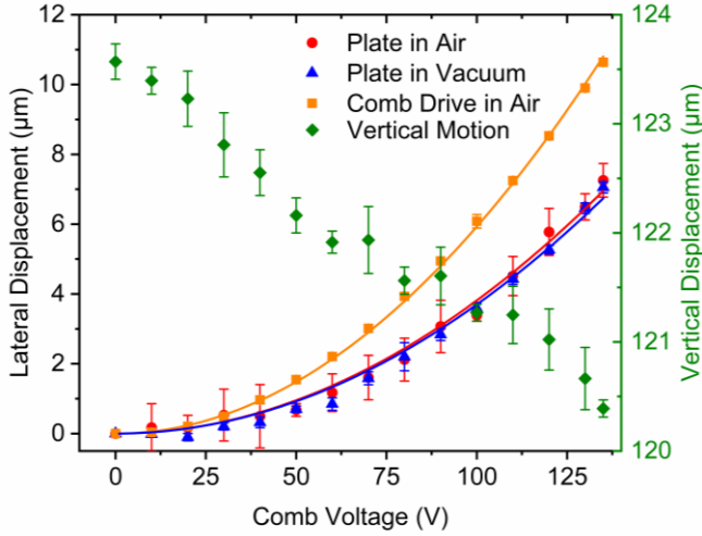
Fig. 3. Lateral actuation of the device obtained using the comb drives. Data and V2 fits are shown for both air and vacuum actuation, for both the central plate and the comb drive itself. Because of an asymmetry in the electrostatic potential on the fingers of the comb drive and a torque on the bimorphs, there is a small vertical motion of the plate when the drives are actuated. Error bars represent twice the standard deviation above and below the average of three measurements.
