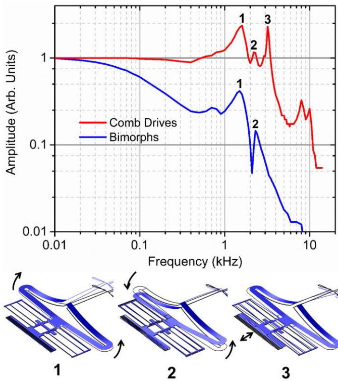
Fig. 6. Frequency response of the 5 DoF scanner. Comb drive actuation responds fully up to 3.2 kHz while actuation using thermal bimorphs begins to fall off above 10 Hz because the response speed is limited by the cooling rate. Below the graph are the various modes associated with the peaks (generated by a FEA in Comsol Multiphysics). Mode 1 is an up and down oscillation of the bimorphs where the bimorphs move in phase with each other. Mode 2 is also an up and down oscillation of the bimorphs, but the bimorphs move out of phase with each other. Mode 2 also possesses some small tilting of the structure. Mode 3 is a lateral in and out oscillation of the comb drive. The peak associated with this mode only appears in the response to the comb drive actuation because the bimorph actuation does not excite it.
