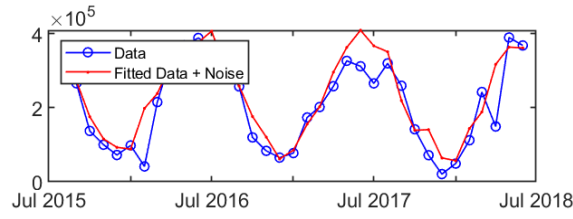
(c) Alternate history of Clarkson Solar energy trace generated using (3.7).
