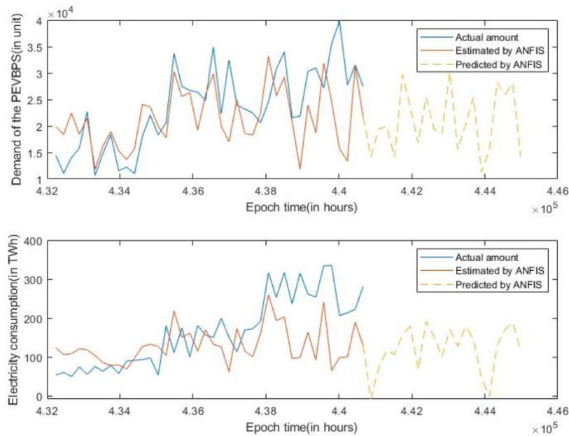
Figure 9 Predicted results for customer demand and electricity consumption using AI Framework
