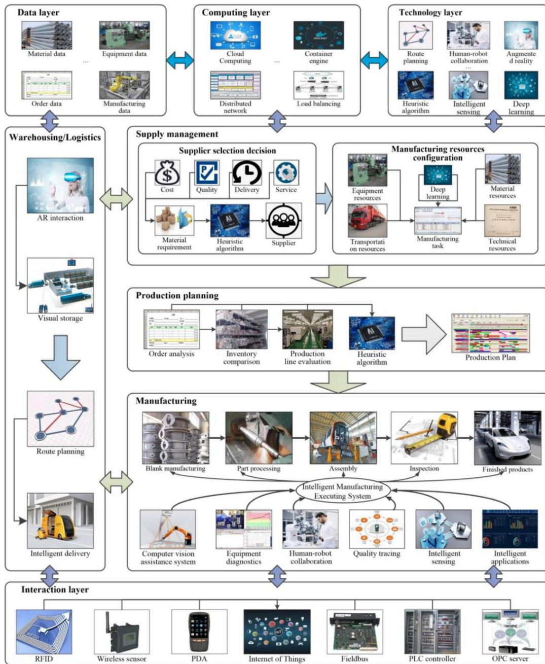
Figure 3 AI-enhanced product manufacturing
