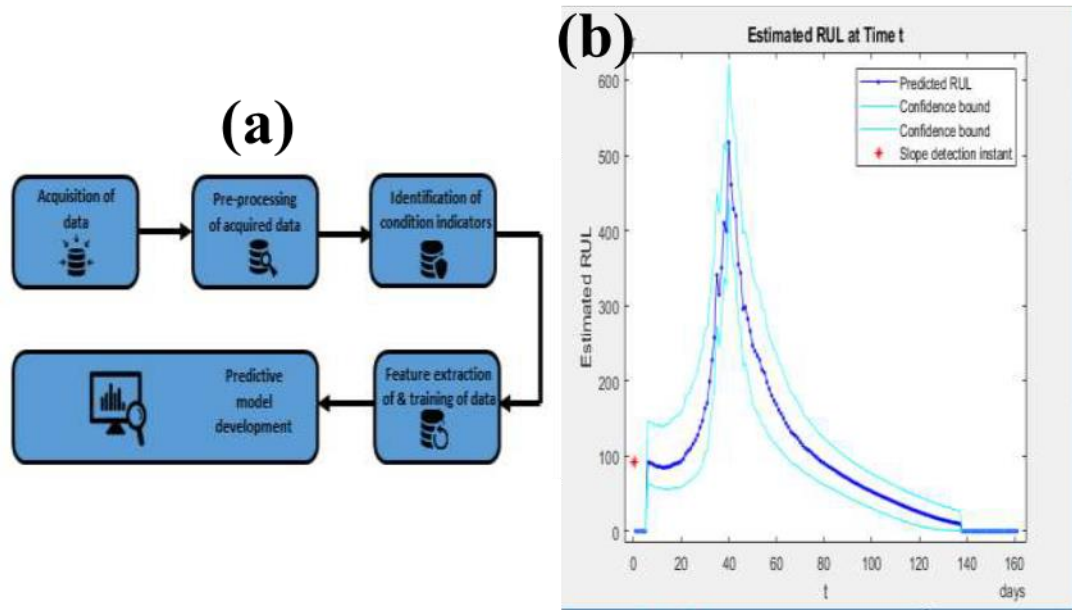
Figure 7 (a) Prediction Process using AI (b) Predicted life using AI framework
