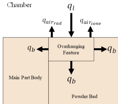
Figure 2: SLM heat transfer model
