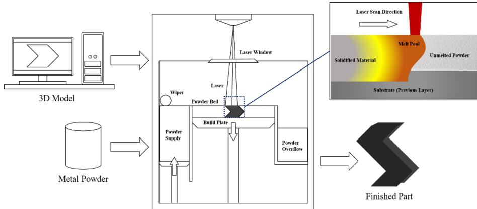
Figure 1: SLM process schematic [5]
