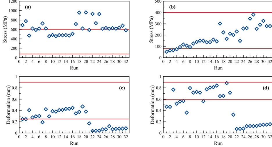
Figure 7: Results compared with experimental data, (a) melt pool stress compared with [6], (b) central feature stress compared with [6], end feature deformation (Ti-6Al-4V) compared with [27], and (d) end feature deformation (316L) compared with [27]
