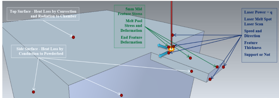
Figure 3: Model Geometry, inputs, and outputs
