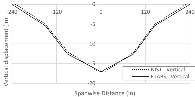
Figure 3. Vertical displacement profiles of beams corresponding to vertical loads for the RBS specimen at 286 kip.
