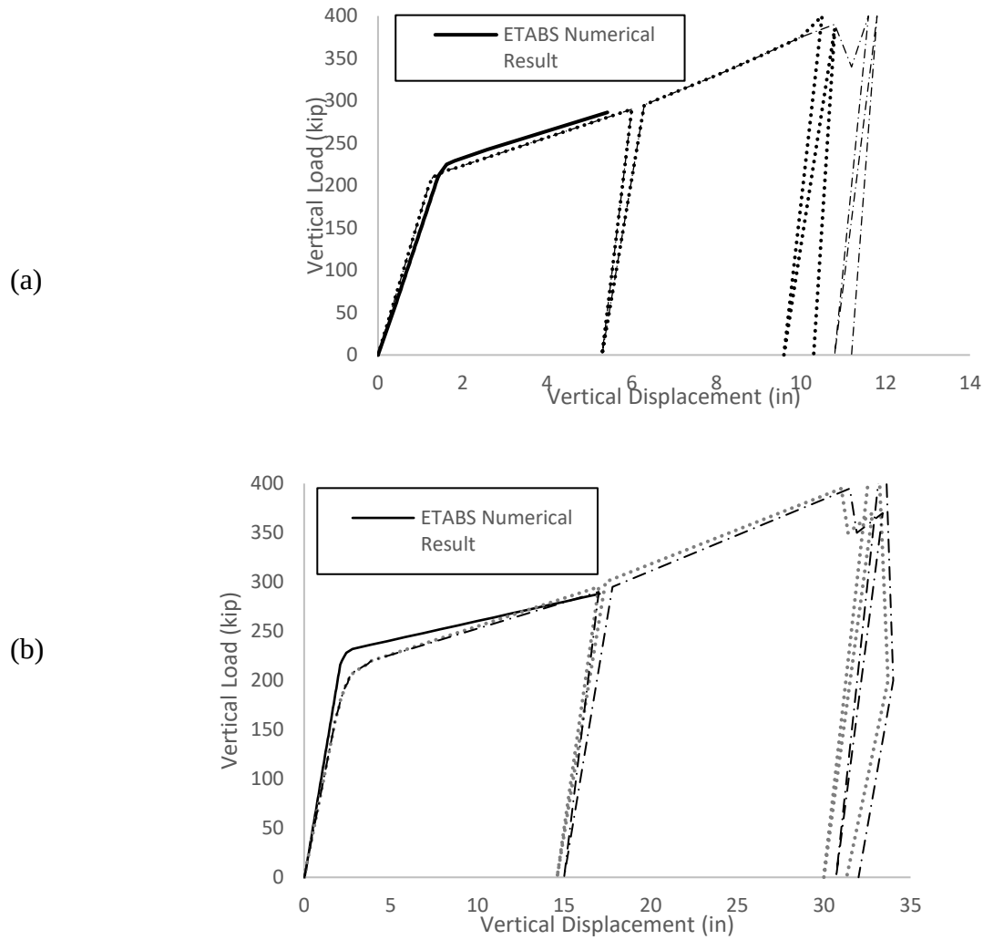
Figure 2. Applied vertical load versus vertical displacements at (a) 1/3 span of beams and (b) center column for the RBS specimen.
