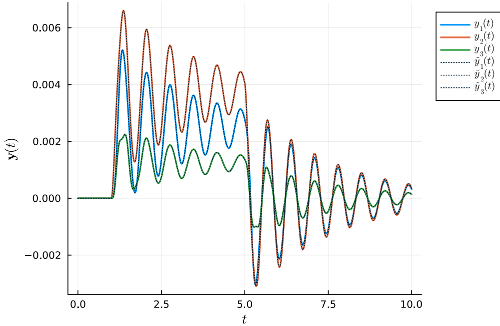
Figure 6: Complete solution for the three DOFs example subjected to an unitary step between t = 1 and t = 5 s. Solutions y_1 , y_2 and y_3 , (real part) obtained by using the proposed approach, are shown as solid lines. Solutions \tilde{y}_1 , \tilde{y}_2 and \tilde{y}_3 , obtained by using the Newmark-beta method are shown as dotted lines.
