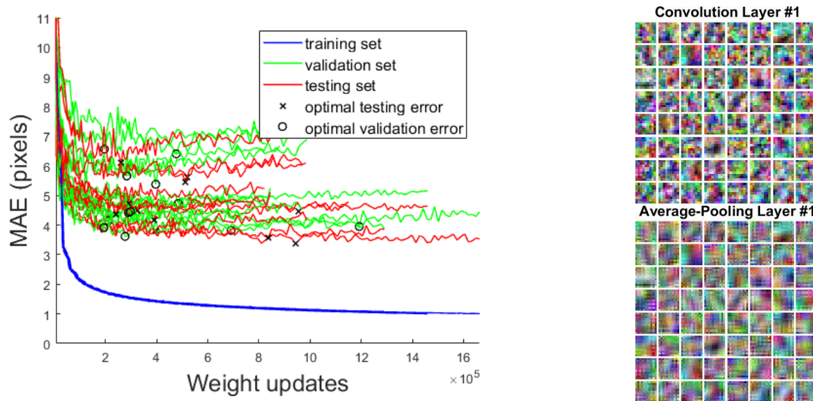
Figure 2. Neural network learning curve and convolution filters. Left: shows the 3 learning curves for all 12 neural networks; the number of weight updates required for convergence over all 12 held-out children was between 200,000 and 1,200,000. The axes show training iterations (weight updates), against mean absolute error in pixels between the neural network and the labels. Initially, speed of convergence is very quick, and then it rapidly slows down. Right: filters learned by the first 2 layers of a trained neural network.
