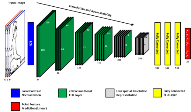
Figure 2. Neural network architecture. Layers of convolutional Exponential Linear Unit (ELU) filters (green) are shown with spatial down-sampling (average-pooling) to learn a low-resolution spatial feature representation of the 256x256x3 (RGB pixels), local contrast normalized (LCN) (blue), input image* (far left). Multiple fully connected ELU layers (yellow) then map that feature representation to the prediction of 13 points of interest, with a final linear regression layer (red).
