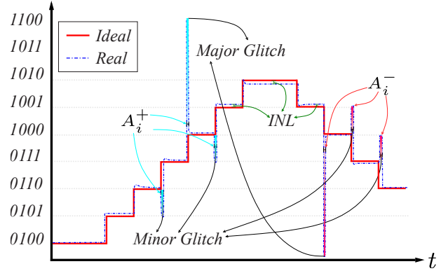
Fig. 1. Persistent non-linear deviations in conventional DACs including INL, and glitches. Where A_i^+ ( A_i^- ), indicate net areas of impulse responses for glitches due to references of rising (falling) trend.
