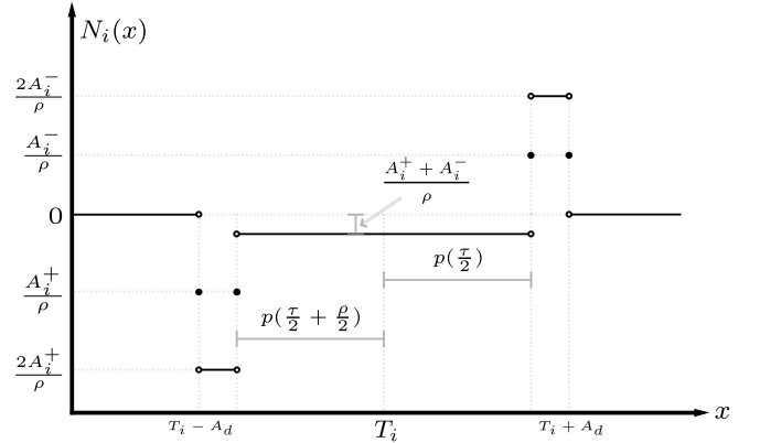
Fig. 4. N_i(x) - the smoothed non-linearity of a single glitch n_{g_i} , due to a periodic dither p(t) .
