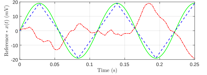
Fig. 7. Dithered glitch response: A) Waveforms of a reconstructed (filtered) 9 Hz, 125 LSB peak-to-peak amplitude triangular wave reference x(t) when using dithers with various frequencies and peak-to-peak amplitudes (plots offset for clarity). B) Isolated glitch-induced error from ideal DAC output.
