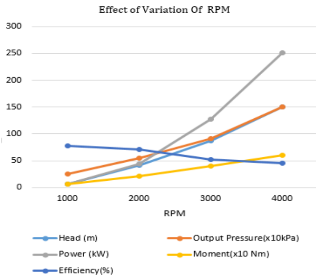
Fig.3.1 Variation of different parameters with RPM
