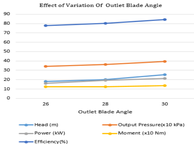
Fig.3.5 Variation of different parameters with Outlet Blade Angle
