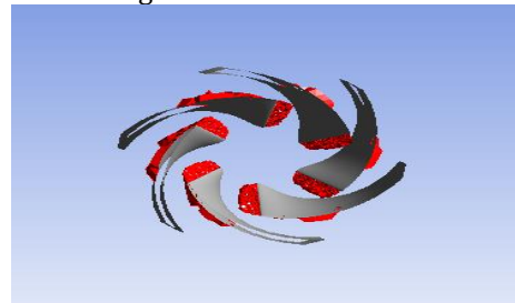
Fig.3.6 Stimulation Result of Cavitation Analysis showing cavitation-affected regions in red.
