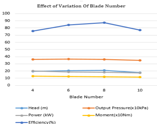
Fig.3.2 Variation of different parameters with Blade Number
