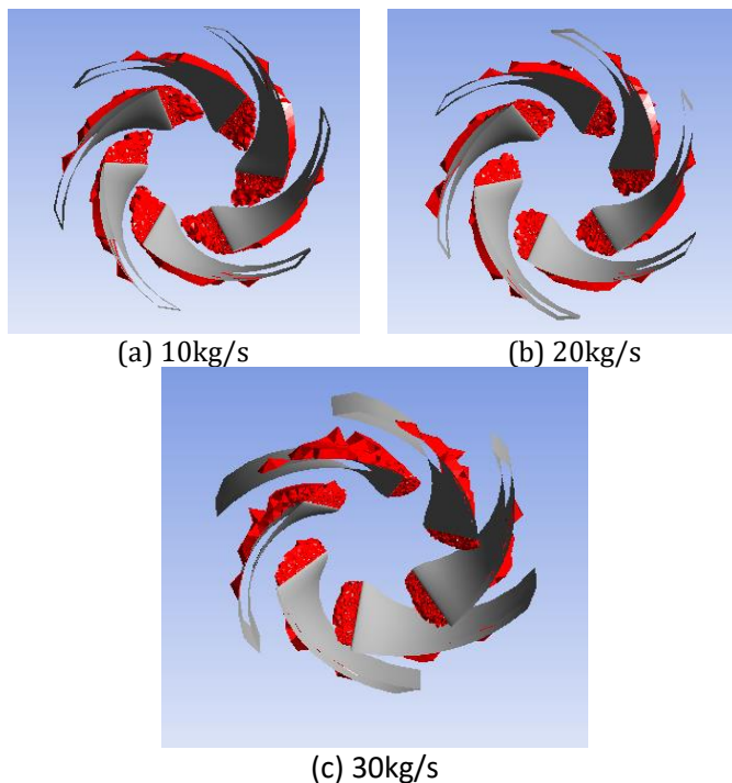
Fig.3.8 Variation of Volume under cavitation with Mass flow rate
