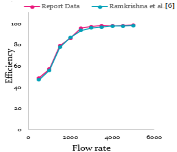
Fig.2.2 Efficiency vs Flow rate plot
