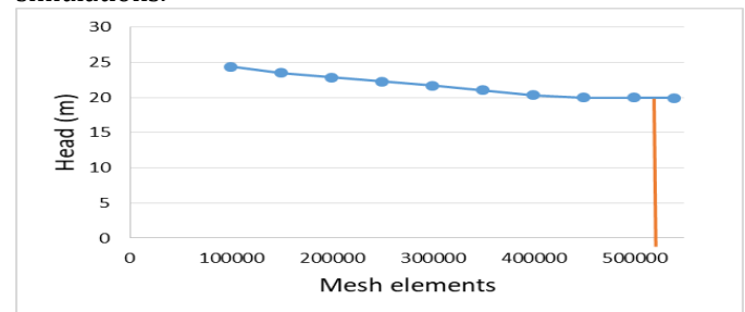
Fig.2.1 Variation of Head with Mesh Elements
