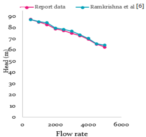
Fig.2.3 Head vs Flow rate plot
