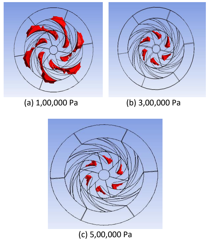
Fig.3.10 Variation of Volume under Cavitation with Outlet Pressure
