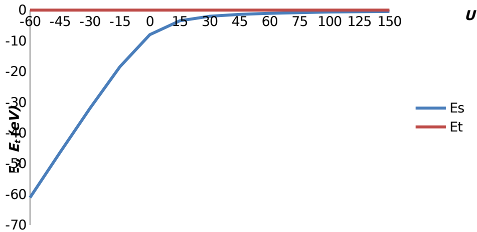
Fig 4.1a: Graph of Singlet ( E_s ) and Triplet ( E_t ) state energies against U for system of 2 electrons on 2 sites.
