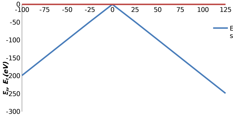
Fig 4.1b: Graph of Singlet ( E_s ) and Triplet ( E_t ) state energies against t for system of 2 electrons on 2 sites.
