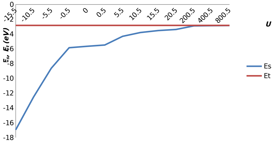
Fig 4.2a: Graph of Singlet ( E_s ) and Triplet ( E_t ) state energies against U for system of 2 electrons on 3 sites.
