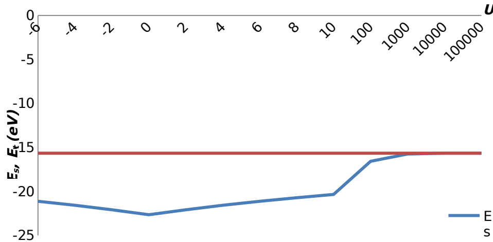
Fig 4.4a: Graph of Singlet ( E_s ) and Triplet ( E_t ) state energies against U for system of 2 electrons on 4 sites.
