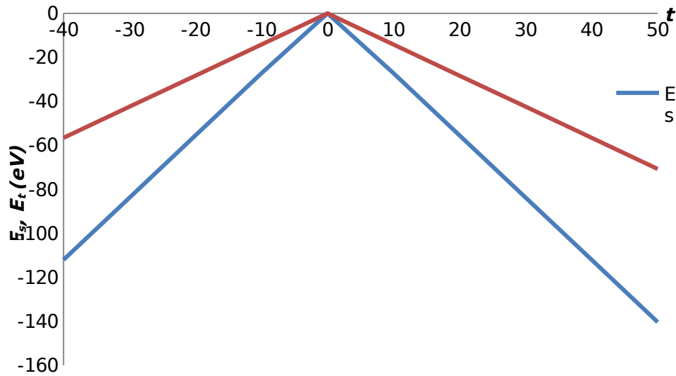
Fig 4.2b: Graph of Singlet ( E_s ) and Triplet ( E_t ) state energies against t for system of 2 electrons on 3 sites.
