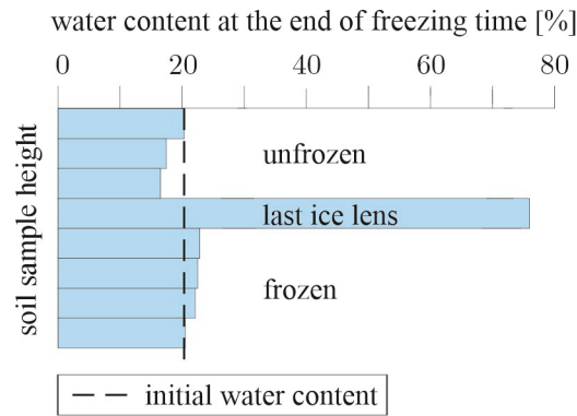
Fig. 4 Soil water distribution after freezing ( T_f = -10^\circ\text{C} ) for BF
