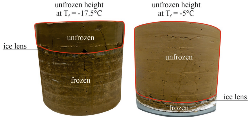
Fig. 3 Unfrozen soil part/flow path (red box) for a freezing temperature of -17.5°C (left) and -5°C (right), BF
