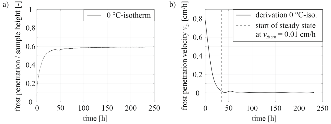
Fig. 7 a) Course of the 0°C-isotherm and b) corresponding frost penetration velocity for BF with a freezing temperature of -12.5°C
