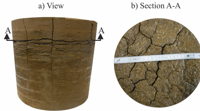
Fig. 6 Longitudinal crack formation of a BF sample
