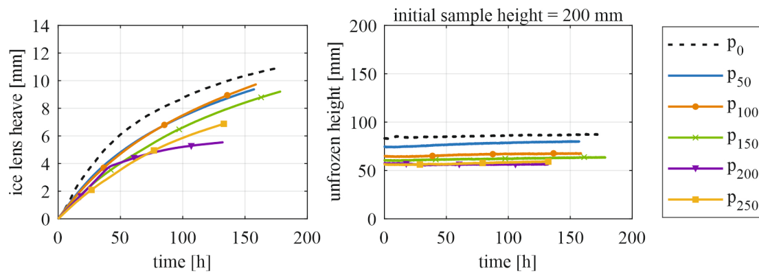
Fig. 16 Ice lens heave (left) and associated unfrozen soil height (right) at the thermal quasi-steady state for a freezing temperature of -12.5^{\circ}\text{C} and varied loads ( p in kPa) for BF
