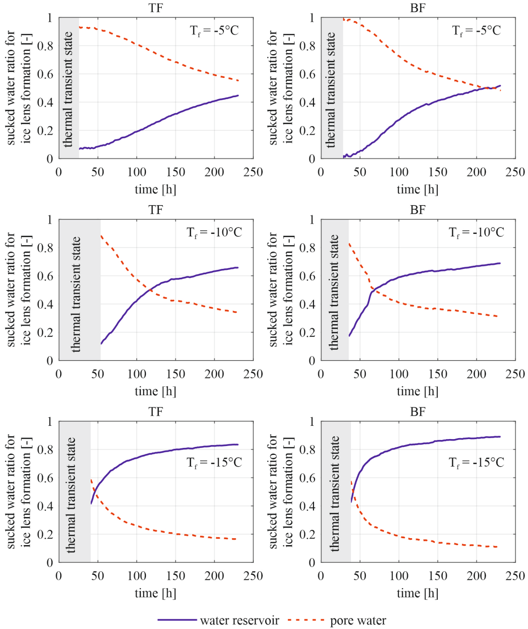
Fig. 5 Origin of the water for the formation of ice lenses at different freezing temperatures for TF and BF
