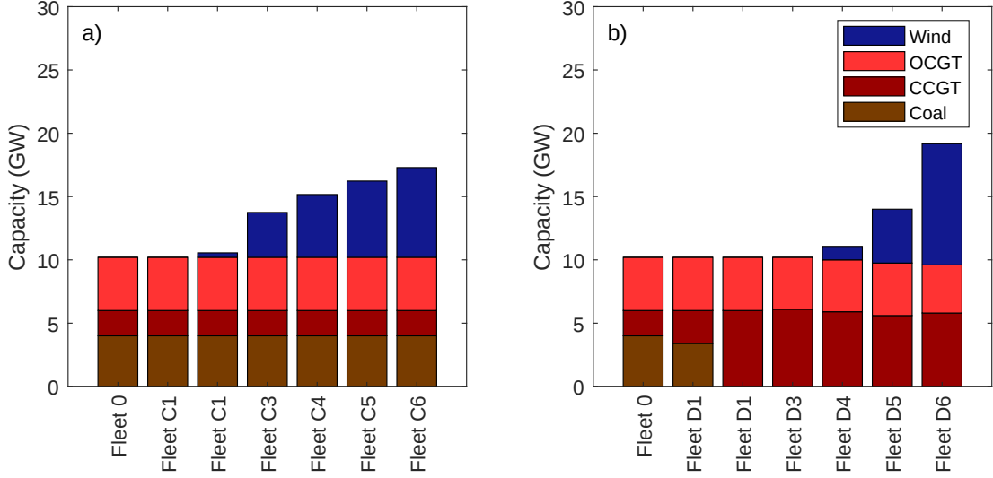
Figure 12: Least cost installed capacities for a) the Fixed Fleet, and b) the Optimised Fleet under a carbon price. Groups of 10 units are shown for coal, CCGT, and 20 units for OCGT. The carbon price increases from the left to right, starting from \$0/\text{tCO}_2 .
