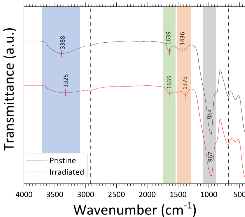
Figure 9. FTIR spectra of pristine versus irradiated metakaolin-based geopolymer in 4000–400 \text{cm}^{-1} wavenumber region, before and after the irradiation.
