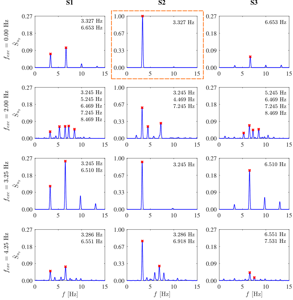
Fig. 9 The normalized PSDs of the velocity component u_y at the probe points S1, S2 and S3 (from left to right) at various f_{exc} . The PSDs are normalized by the peak magnitude at 3.327 Hz of the PSD at S2 in the stationary case, which is encircled by the dashed box in orange. The predominant peaks are marked out with red cross symbols, and the corresponding frequencies are listed aside.
