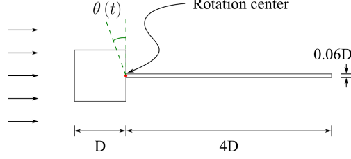
Fig. 1 Schematic of the square blunt body attached with the flexible plate, where the cylinder is in forced vibration. The arrows upstream of the body indicate the inflow direction. The angle \theta(t) varies periodically in time.
