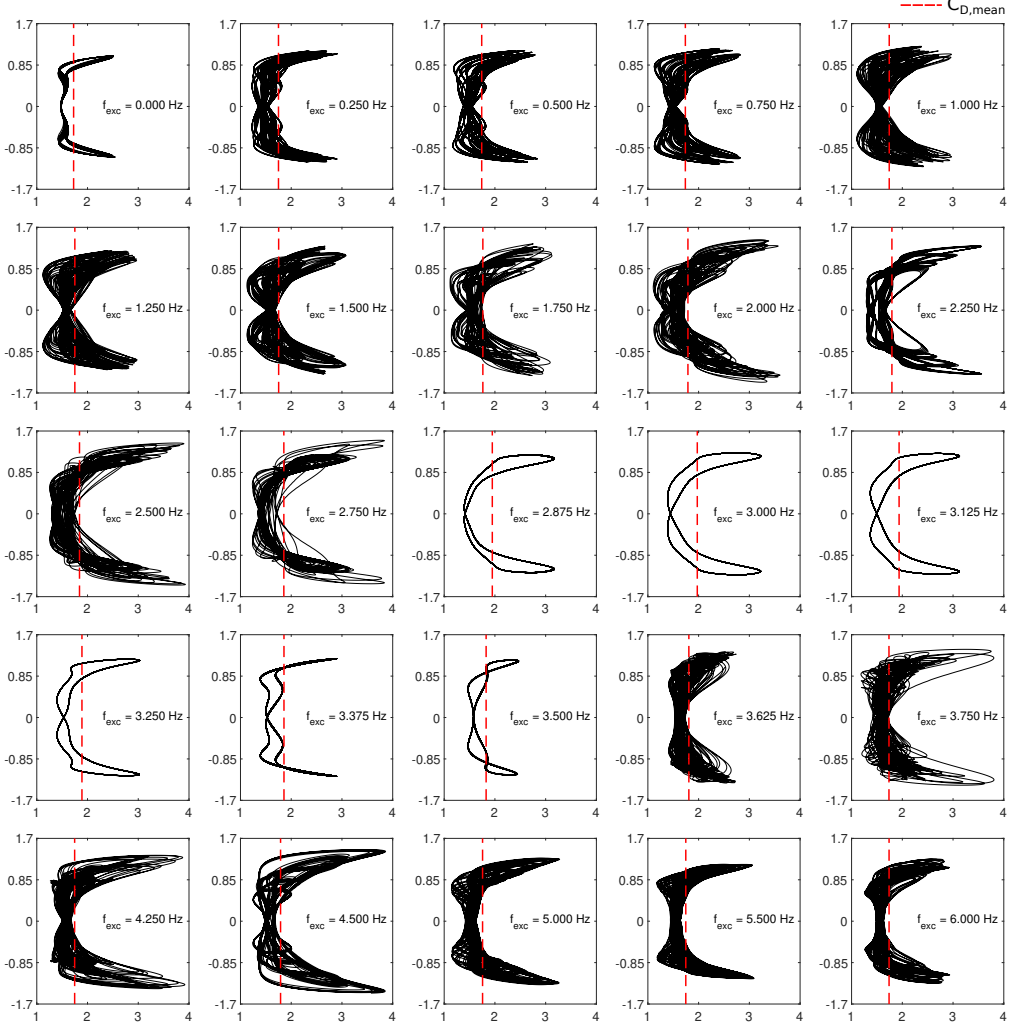
FIGURE 6. The trajectory evolution of y_{tip}/D versus C_D in time. The x-axis is C_D , and the y-axis is y_{tip}/D . The red dash line indicates the time-averaged value of C_D .
