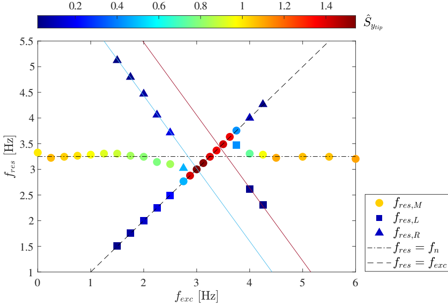
FIGURE 13. The peak frequencies (i.e., the maximum peak frequency f_{res,M} , the secondary peak frequencies f_{res,L} and f_{res,R} below and above f_{res,M} ) of the normalized plate-tip displacement PSD \hat{S}_{ytip} with respect to f_{exc} . The symbols are colored with the normalized magnitudes of the PSDs, \hat{S}_{ytip} , at these frequencies. The dash-dotted line indicates the natural frequency of the plate of f_{n,1} = 3.236 Hz; the blue and red solid lines are plotted based on the ratio of \Delta f_{res}/\Delta f_{exc} = -1 .
