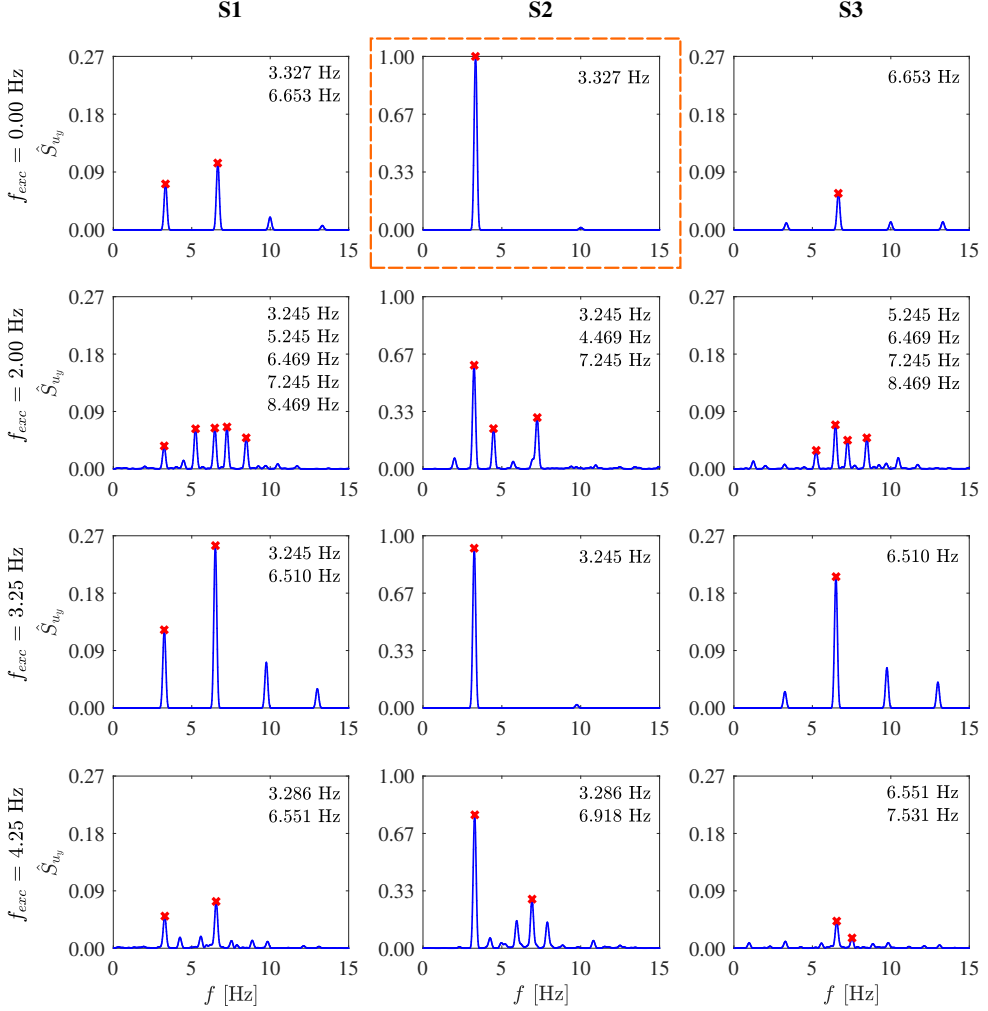
FIGURE 9. The normalized PSDs of the velocity component u_y at the probe points S1, S2 and S3 (from left to right) at various f_{exc} . The PSDs are normalized by the peak magnitude at 3.327 Hz of the PSD at S2 in the stationary case, which is encircled by the dashed box in orange. The predominant peaks are marked out with red cross symbols, and the corresponding frequencies are listed aside.
