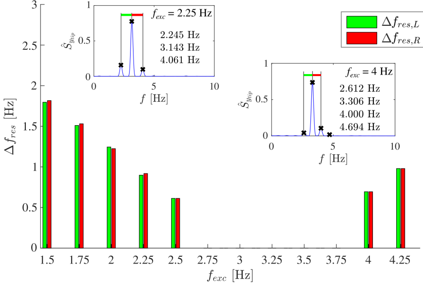
FIGURE 14. The absolute differences between the secondary peak frequencies of the splitter-plate structural responses ( f_{res,L} and f_{res,R} ) and the largest peak frequency f_{res,M} , as a function of the enforced oscillation frequency f_{exc} . These frequencies are referred to Fig. 13.
