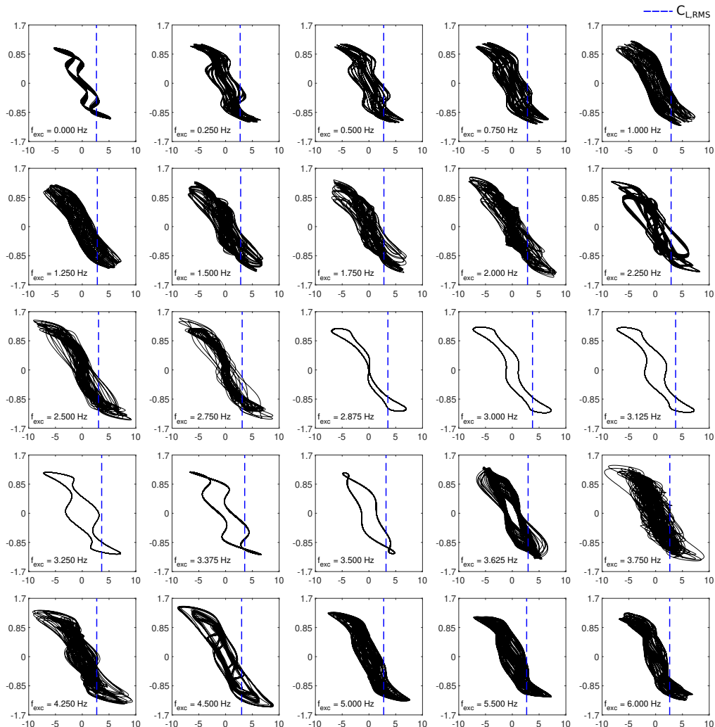
FIGURE 5. The trajectory evolution of y_{tip}/D versus C_L in time. The x-axis is C_L , and the y-axis is y_{tip}/D . The blue dash line indicates the RMS value of C_L .
