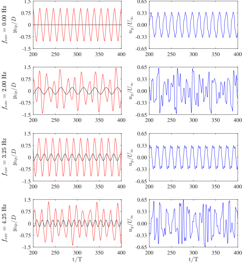
FIGURE 8. The time series of the normalized tip displacement y_{tip}/D and the normalized velocity component u_y/U_\infty at the probe point, S2, in the wake. The black curves in the left figures indicate the tip displacement of a rigid splitter plate.
