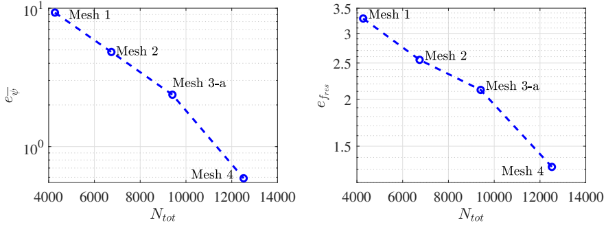
FIGURE 3. The errors of the time-averaged absolute tip displacement \bar{\psi} and the peak frequency of the tip displacement f_{res} from the different mesh resolution in reference to the finest mesh, Mesh 5, as a function of the total number of cells N_{tot} .
