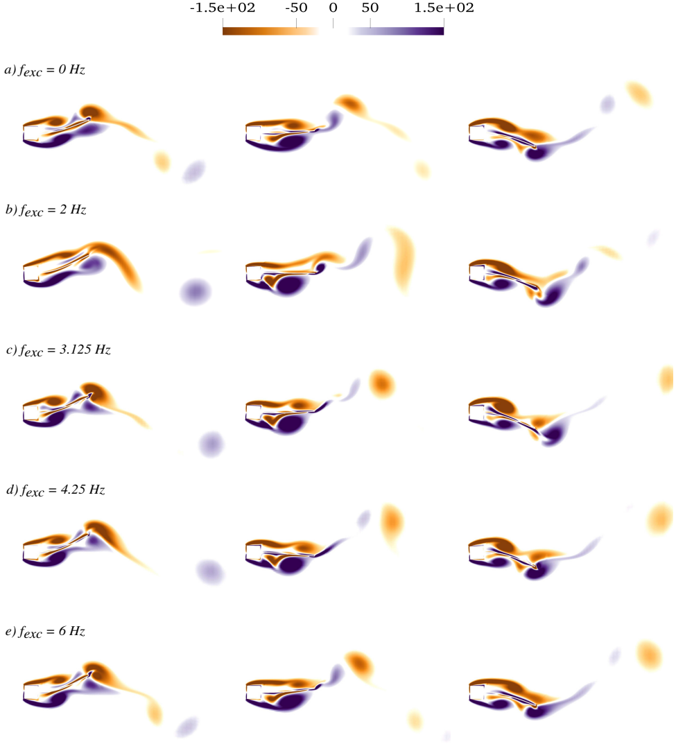
FIGURE 7. Snapshots of the vorticity component \omega_z . From left to right: approximately the position of the maximum tip displacement, the neutral position, and the position of the minimum tip displacement.
