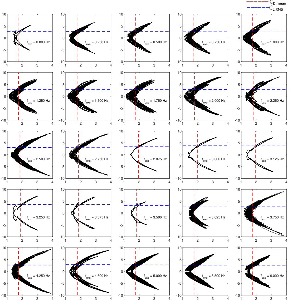
FIGURE 4. The trajectory evolution of C_L versus C_D in time. The x-axis is C_D , and the y-axis is C_L . The red and blue dash lines mark out C_{D,mean} and C_{L,RMS} .
