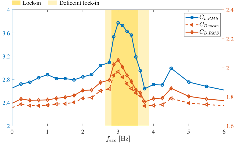
FIGURE 11. The RMS lift coefficient, C_{L,RMS} , and the time-averaged and RMS drag coefficients, C_{D,mean} and C_{D,RMS} , as a function of the enforced oscillation frequency f_{exc} .
