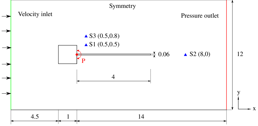
FIGURE 2. Schematic of the fluid and structure computational domains. The dimensions are normalized based on the square cylinder width D . The triangles mark out the probe positions such as S1, S2 and S3 for monitoring flow variables.
