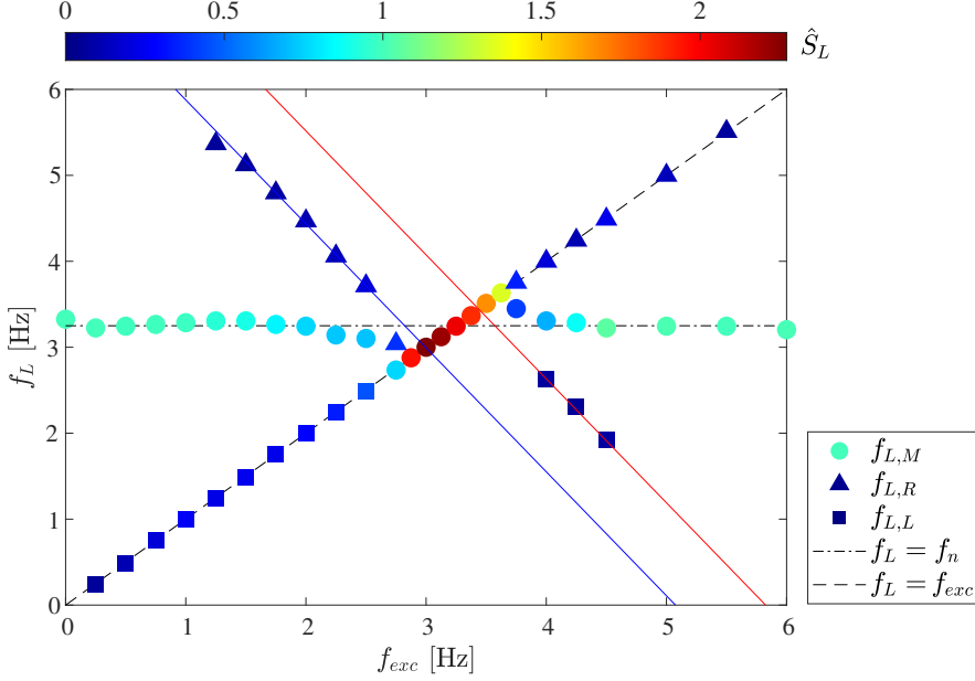
FIGURE 12. The maximum peak frequency in the PSDs of the lift force, f_{L,M} , and the secondary peak frequencies, f_{L,L} and f_{L,R} , with respect to f_{exc} . The symbols are colored with the normalized magnitudes of the PSDs, \hat{S}_L , at these frequencies. The dash-dotted line marks out the natural frequency of the plate of f_{n,1} = 3.236 Hz; the blue and red solid lines are drawn based on the ratio of \Delta f_L / \Delta f_{exc} = -1 .
