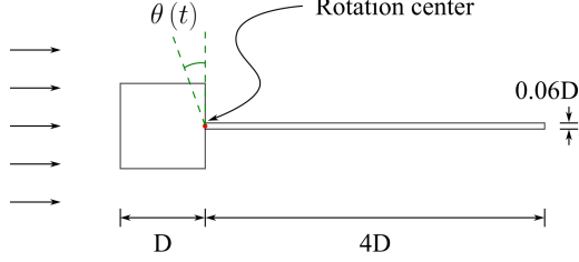
FIGURE 1. Schematic of the square blunt body attached with the flexible plate, where the cylinder is in forced vibration. The arrows upstream of the body indicate the inflow direction. The angle \theta(t) varies periodically in time.
