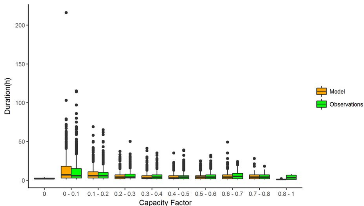
Figure A8: Frequency (hours per year) of simulated and observed historic values for different capacity factor classes
