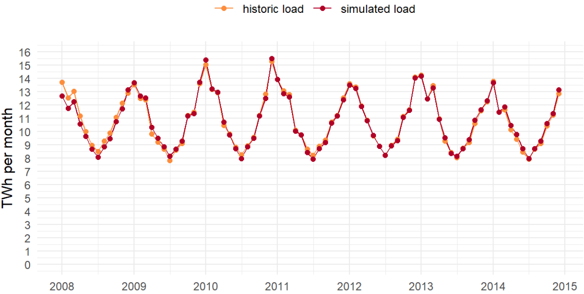
Figure A5: Monthly historic and simulated load from 2008 to 2014
