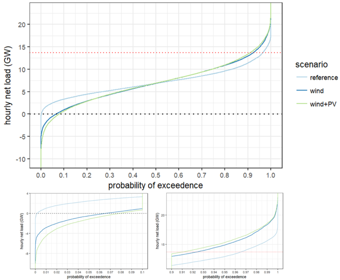
Figure 4: Distribution of hourly residual loads in the reference and the fully renewable scenarios. We define residual load here as load – wind – PV – nuclear. The red dotted line shows the maximum observed hydropower generation between 2007 and 2014. Above: full distribution. Below: Lower and upper end of distribution.
