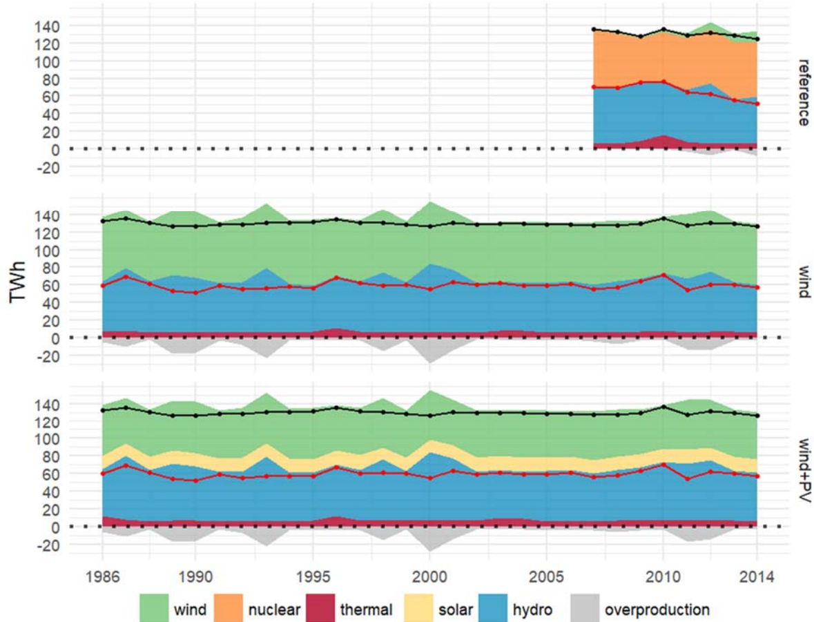
Figure 2: Annual load (black line), residual load (red line) and generation by source (nuclear, thermal, hydro, wind and solar PV) from 1986 to 2014 (the reference scenario relies on historic data from 2007 to 2014).
