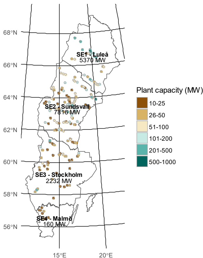
Figure A2: Cumulated hydropower capacity per bidding area and location and capacity of the 200 largest hydropower plants in Sweden that amount to 95 % of the total installed capacity and have been included in our analysis
