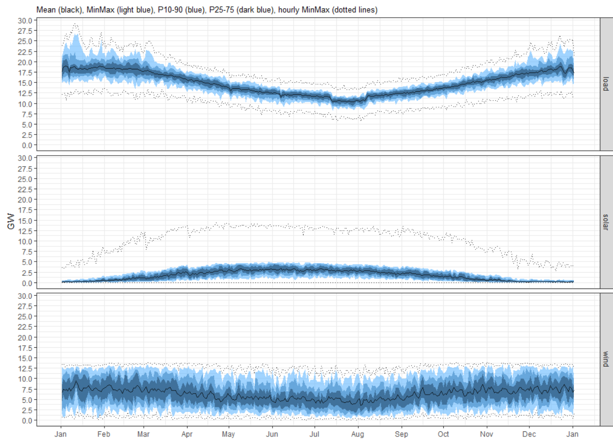
Figure 1: Interannual and seasonal variation of simulated electricity demand (load), solar PV and wind generation from 1986 to 2014 in the Wind+PV scenario. The black line shows the daily mean values over 29 years of simulated temperature dependent load and generation. The shaded areas indicate the observed variation of daily mean values in the simulated time series: minimum and maximum values in light blue, 10th to 90th percentile in blue and 25th to 75th percentile in dark blue. The dotted lines show the hourly minimum and maximum load and generation for each day.
