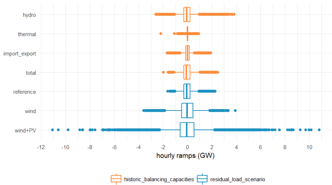
Figure 5: Hourly residual load ramps (blue) in the three scenarios (Reference, Wind and Wind+PV) compared with historically observed ramps of balancing capacities (orange) (hydro and thermal power plants, as well as imports and exports). The “total” ramp boxplot shows the observed combined hourly ramps of all balancing capacities.
