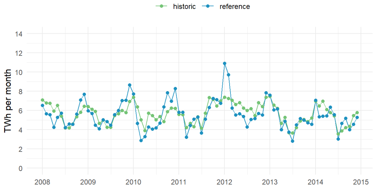
Figure A4: Monthly historic and optimized hydropower generation in the reference scenario. The historic hydropower generation shows data from Svenska Kraftnät and the reference scenario time series shows results of the optimization model for minimizing residual load demand.
