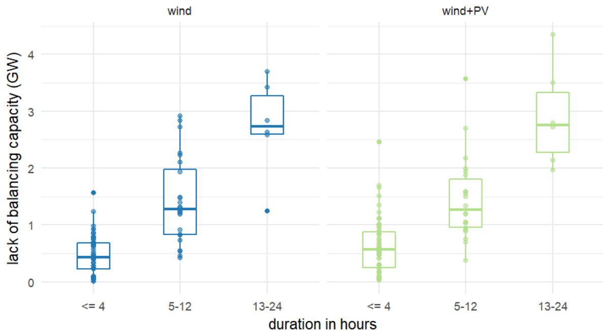
Figure 7: Lack of balancing capacities in the Wind and Wind+PV scenarios, grouped by the duration of the extreme residual load events
