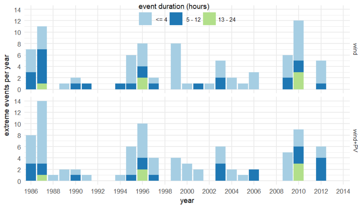
Figure 6: Number of extreme residual load events in the Wind and Wind+PV scenarios that exceed the balancing capacity of current hydro and thermal power plants.
