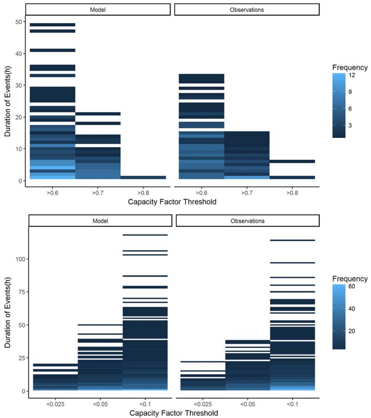
Figure A99: Comparison of durations and frequencies of high (above) and low (below) generation events in the simulated and the historically observed time series
