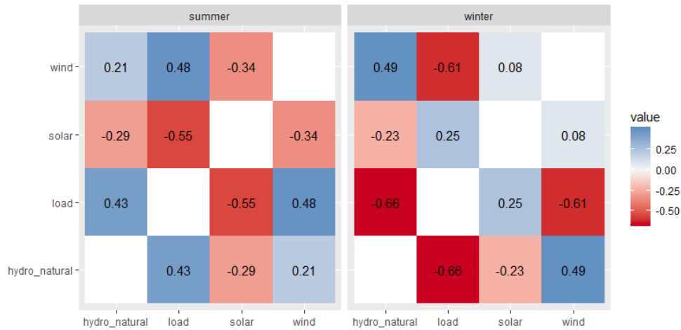
Figure 3: Correlation matrix of deseasonalized monthly load, solar, wind and simulated hydro generation for the summer (June, July and August) and winter months (December, January and February)
