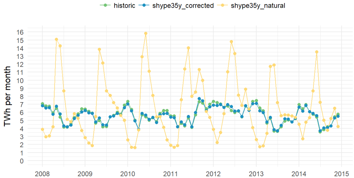
Figure A3: Monthly historic and simulated hydropower generation in TWh. The shype35y_corrected time series accounts for the effect of historic hydropower generation on river runoff, while shype35y_natural shows the theoretic hydropower generation without hydro reservoirs or any other human interference
