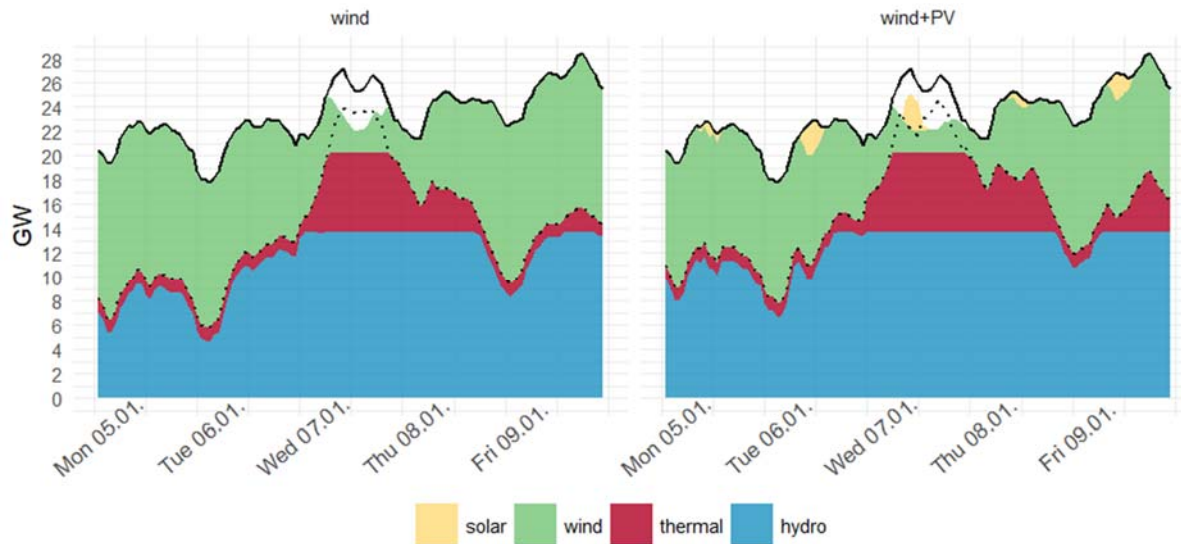
Figure 8: Hourly load (black line), residual load (black dotted line) and generation capacities (solar, wind, thermal and hydro) for the week in 1987 with the highest and longest extreme residual load event within in the complete 29 year period.
