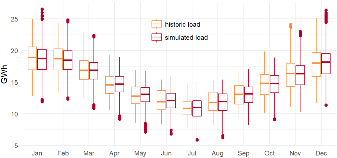
Figure A6: Distribution of historic and simulated hourly loads for all month from 2008 to 2014.
