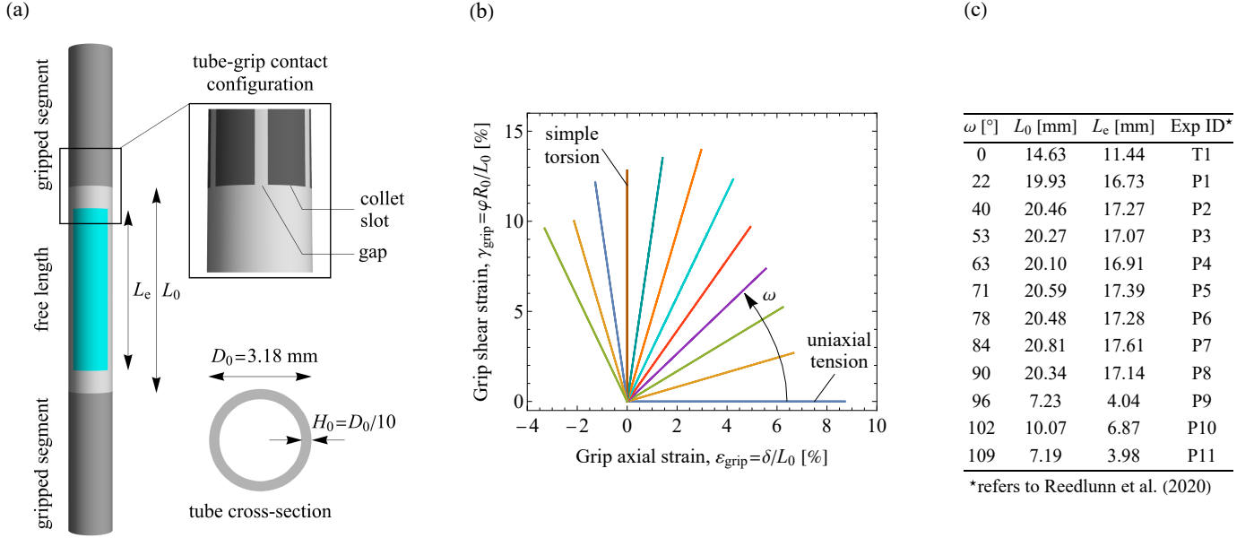
Figure 2: Setup of the problem: (a) tube geometry and the gripping layout, (b) the proportional axial–shear strain paths selected for the simulations, and (c) geometric and loading parameters of each simulation and the corresponding experiment from Reedlunn et al. (2020a). The blue-shaded area in panel (a) represents a section of the tube (with an axial length L_e and an angular extent of 100^\circ ) that resembles the virtual DIC extensometer region in the experiment.
