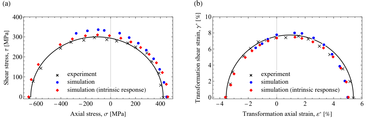
Figure 19: The predicted transformation-onset stress and transformation strain loci and their comparison with the experimental results of Reedlunn et al. (2020a). The superimposed ellipses (solid lines) are the parametric surfaces proposed by Reedlunn et al. (2020a) and are fitted to the experimental data, see their Fig. 26.
