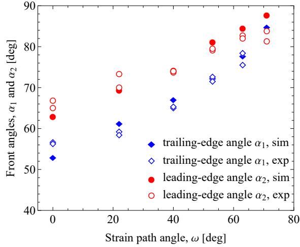
Figure 21: Front angles \alpha_1 and \alpha_2 as a function of strain-path angle \omega in combined tension–torsion. The angles \alpha_1 and \alpha_2 are measured in the undeformed and unwrapped-tube configuration.
