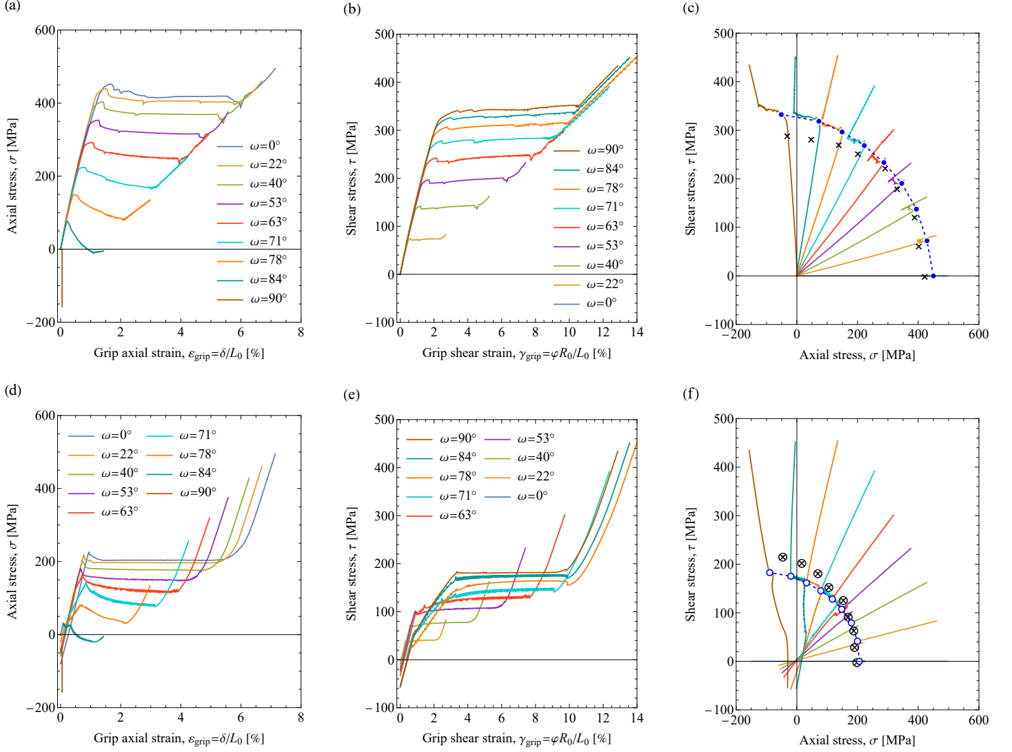
Figure 18: Global mechanical responses in combined tension–torsion: (a,b,c) loading stage, and (d,e,f) unloading stage. The blue circles in panels (c,f) denote the characteristic transformation stresses extracted from the simulation results, while the cross markers denote the analogous experimental points. All cases, including uniaxial tension (see Fig. 4), correspond to the limit friction stress of T_c = 20 MPa. The response for simple torsion ( \omega = 90^\circ ) corresponds to the case with an initial radial compression induced by the collets.
