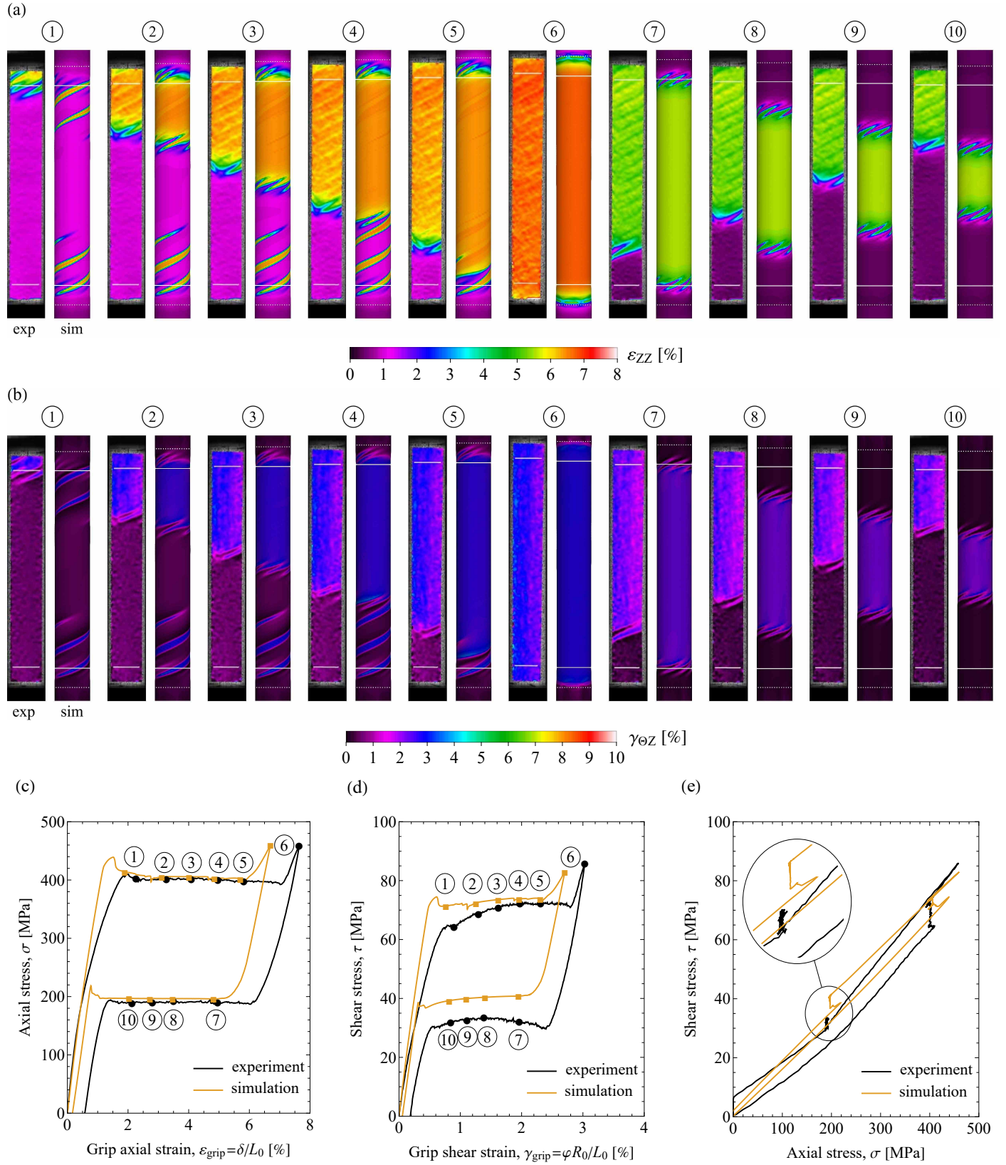
Figure 11: Simulation results for the case of combined tension–torsion at \omega = 22^\circ and their comparison with the experimental results (case P1) of Reedlunn et al. (2020a). The left-hand and right-hand snapshots in panels (a) and (b) correspond, respectively, to the experiment (reproduced with permission from Elsevier) and simulation.
