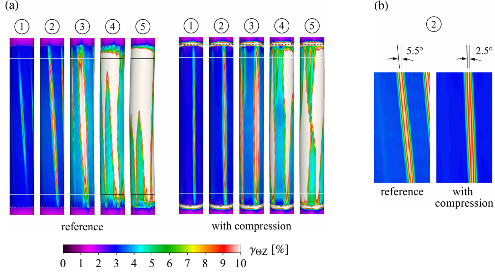
Figure 8: The impact of the radial compression induced by the collet grips on the transformation pattern during loading (a) and the orientation of the longitudinal bands (b) in simple torsion. The close-up views in panel (b) are taken in the undeformed and unwrapped-tube configuration.
