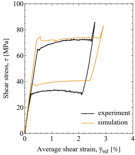
Figure F.1: Selected mechanical responses in terms of the average strains \bar{\epsilon}_{ZZ} and \bar{\gamma}_{\theta Z} and their comparison with the experimental results of Reedlunn et al. (2020a): (a) tension–torsion with \omega = 22^\circ (case P1), (b) tension–torsion with \omega = 63^\circ (case P4), and (c) compression–torsion with \omega = 102^\circ (case P10).
