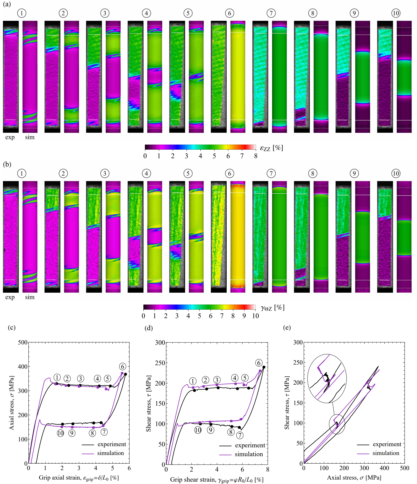
Figure 13: Simulation results for the case of combined tension–torsion at \omega = 53^\circ and their comparison with the experimental results (case P3) of Reedlunn et al. (2020a). The left-hand and right-hand snapshots in panels (a) and (b) correspond, respectively, to the experiment (reproduced with permission from Elsevier) and simulation.
