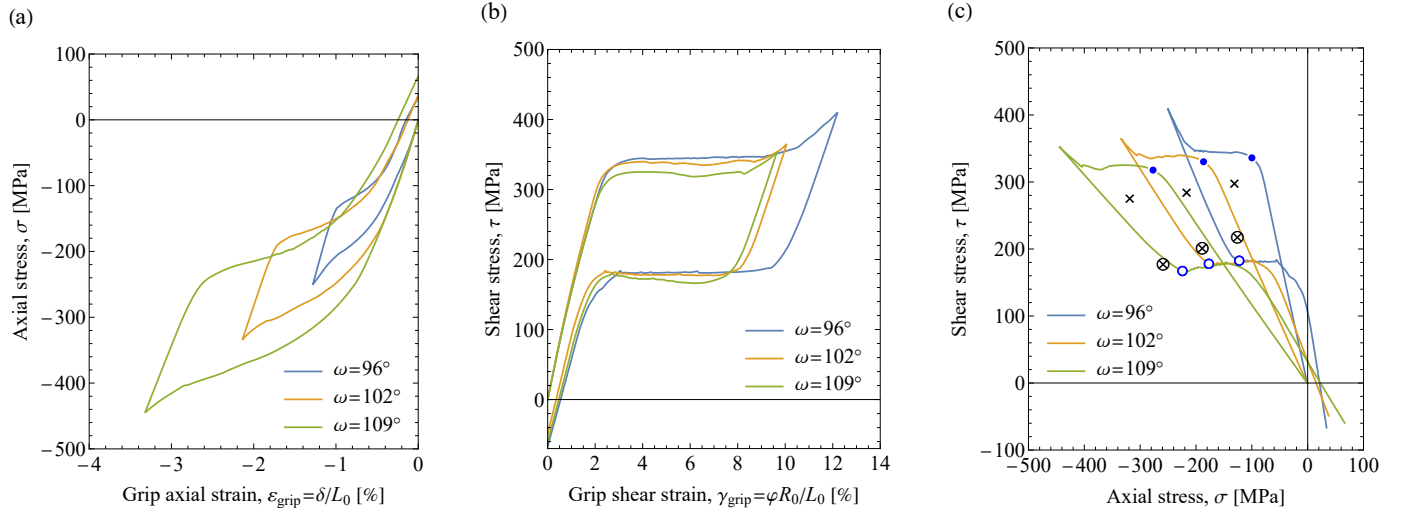
Figure 25: Global mechanical responses in combined compression-torsion. The blue circles in panel (c) denote the characteristic transformation stresses extracted from the simulation responses, while the cross markers denote the analogous experimental points.
