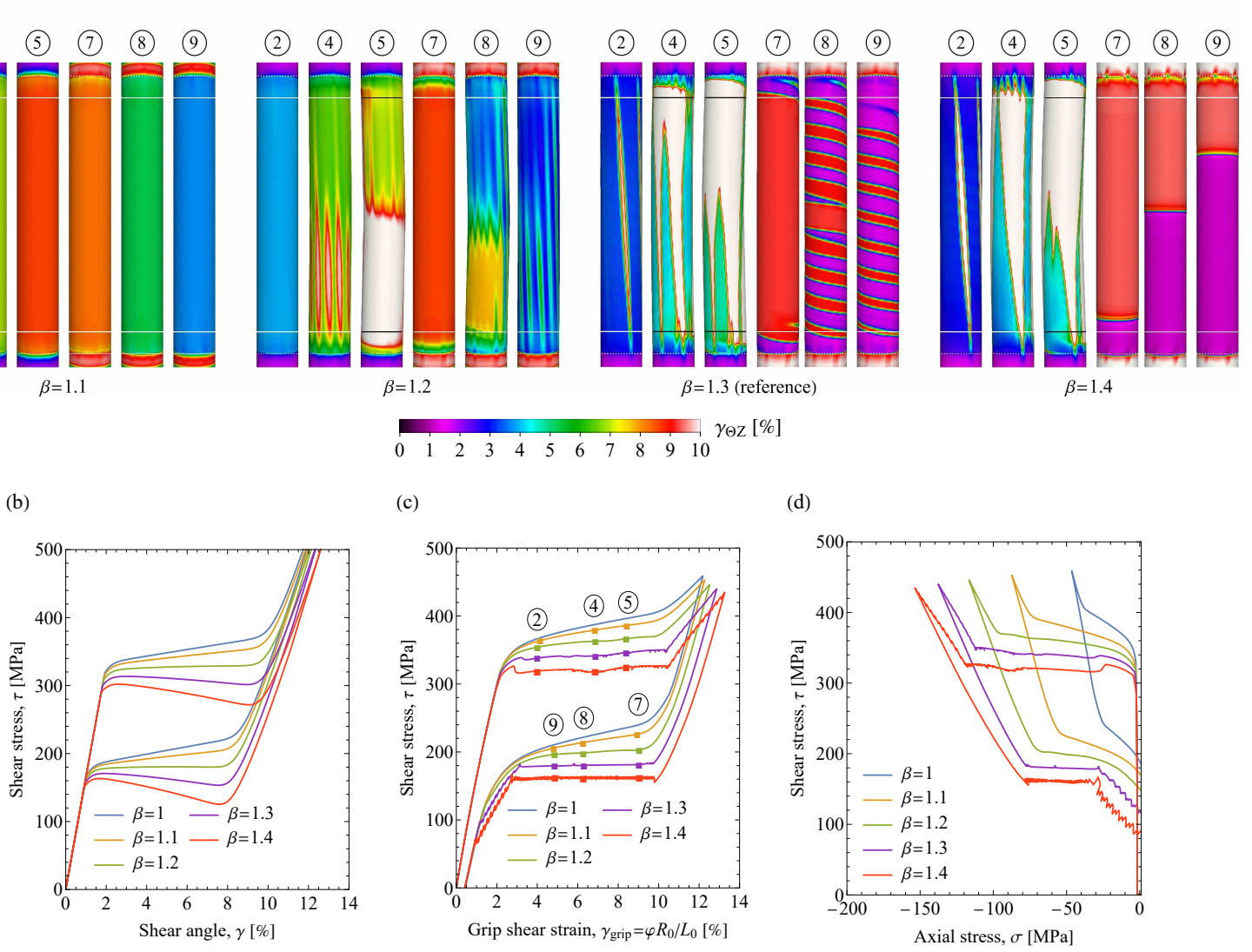
Figure 10: The effect of parameter \beta , controlling the degree of transverse isotropy, on the transformation pattern and on the mechanical response in simple torsion: (a) snapshots of the shear strain field \gamma_{\Theta Z} , (b) the intrinsic response in shear, (c) the global shear stress–grip shear strain ( \tau – \gamma_{grip} ) response, and (d) the global shear stress–axial stress ( \tau – \sigma ) response. The case with \beta = 1.3 represents the reference simulation. Note that the homogeneous transformation obtained for \beta = 1 is roughly the same as that of \beta = 1.1 , and thus is not shown in panel (a).
