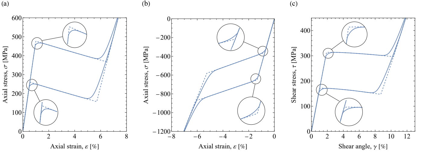
Figure 1: The intrinsic stress-strain response corresponding to (a) uniaxial tension, (b) uniaxial compression, and (c) shear (material parameters correspond to those specified in Table E.1). The dashed curves indicate the trilinear response obtained by excluding the contribution of h(\eta) . Within the transformation-saturation region, the model with h(\eta) exhibits a very gradual transition with a stress-strain slope that tends to the apparent elastic modulus of martensite.
