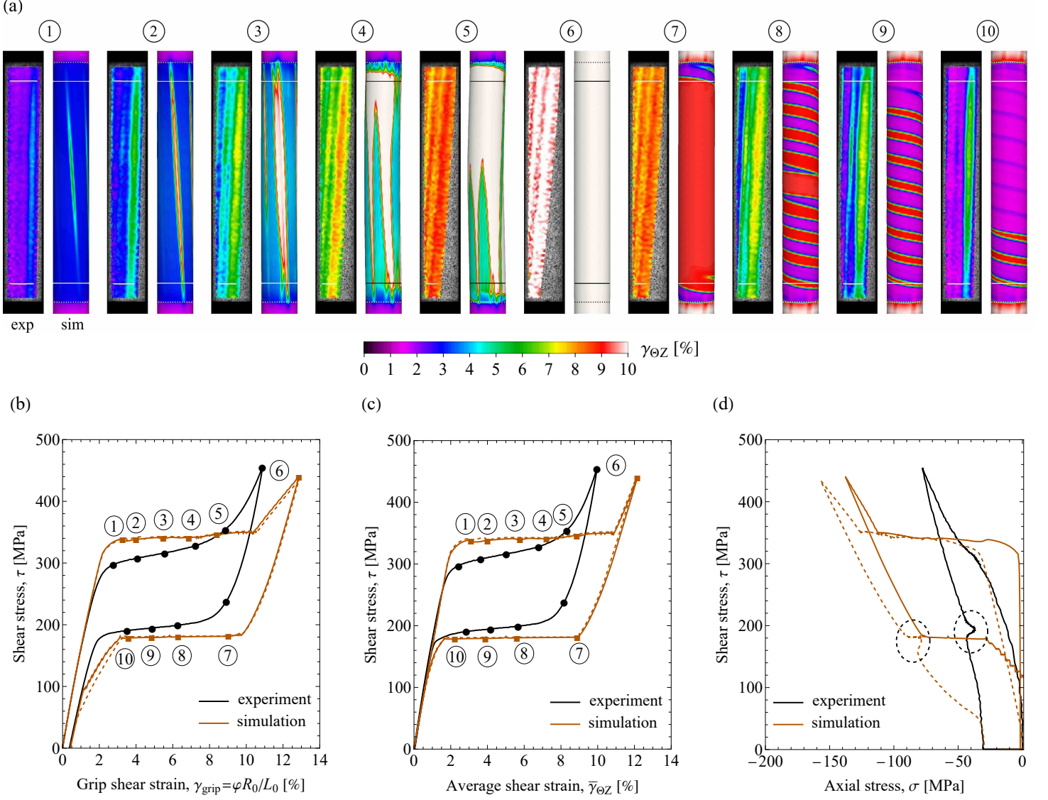
Figure 7: Simulation results for the case of simple torsion ( \omega = 90^\circ ) and their comparison with the experimental results (case P8) of Reedlunn et al. (2020a): (a) snapshots of the shear strain field \gamma_{\Theta Z} , (b,c,d) the global mechanical response represented in terms of (b) shear stress–grip shear strain ( \tau – \gamma_{\text{grip}} ), (c) shear stress–average shear strain ( \tau – \bar{\gamma}_{\Theta Z} ), and (d) shear stress–axial stress ( \tau – \sigma ). The left-hand and right-hand snapshots in panel (a) correspond, respectively, to the experiment (reproduced with permission from Elsevier) and simulation. The dashed curves in panels (b,c,d) represent the response for the case with a radial compression induced by the collet grips.
