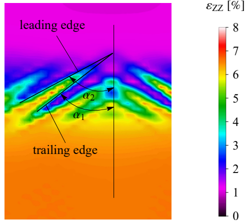
Figure 5: A close-up view of the propagating front (taken in the undeformed and unwrapped-tube configuration) in uniaxial tension.
