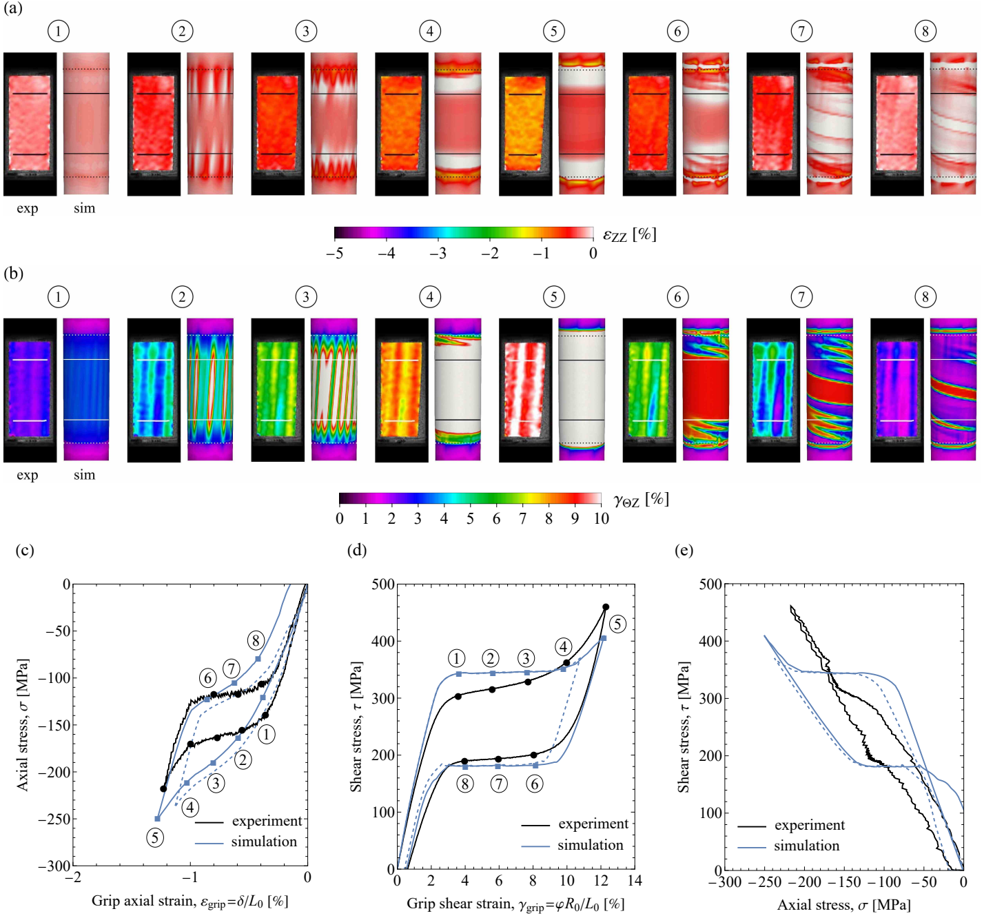
Figure 22: Simulation results for the case of combined compression–torsion at \omega = 96^\circ and their comparison with the experimental results (case P9) of Reedlunn et al. (2020a). The left-hand and right-hand snapshots in panels (a) and (b) correspond, respectively, to the experiment (reproduced with permission from Elsevier) and simulation. The dashed curves represent the mechanical response for the case with a radial compression induced by the collet grips.
