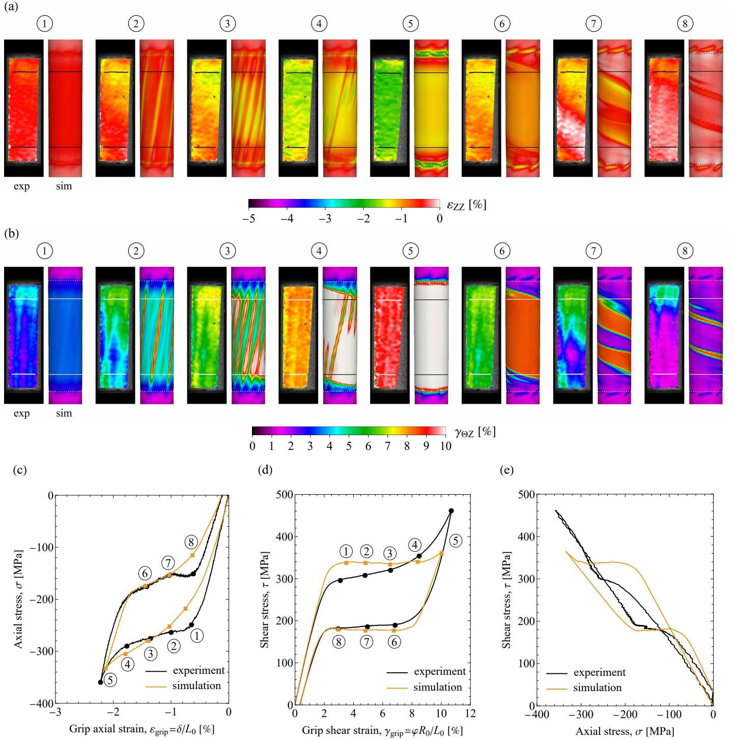
Figure 23: Simulation results for the case of combined compression–torsion at \omega = 102^\circ and their comparison with the experimental results (case P10) of Reedlunn et al. (2020a). The left-hand and right-hand snapshots in panels (a) and (b) correspond, respectively, to the experiment (reproduced with permission from Elsevier) and simulation.
