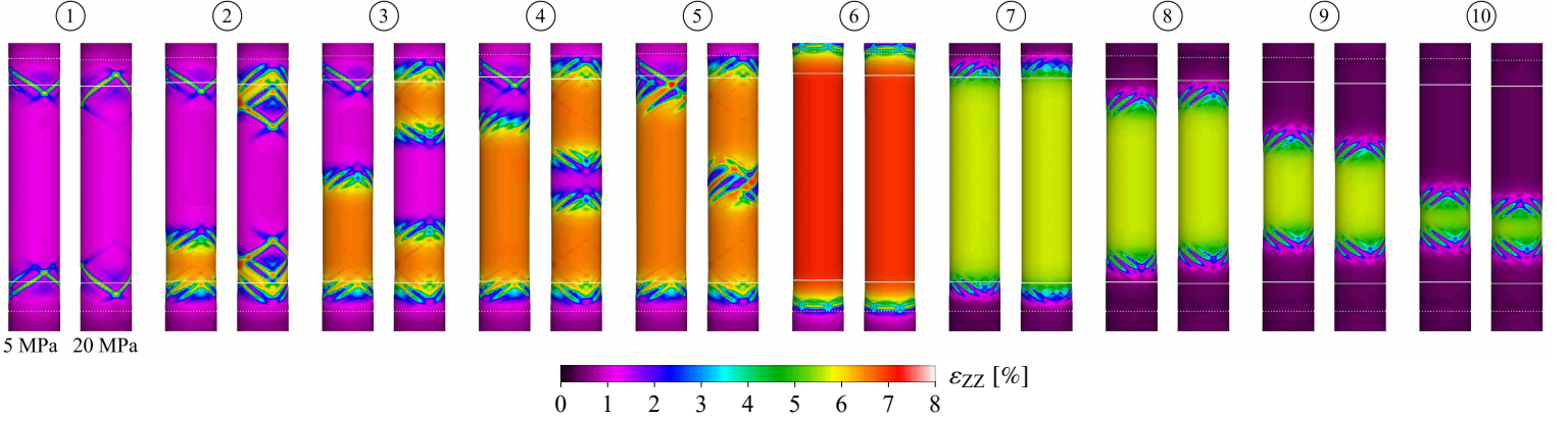
Figure 6: Transformation pattern for the case of uniaxial tension ( \omega = 0^\circ ) with a limit friction stress of T_c = 20 MPa and its comparison with that of the reference simulation with T_c = 5 MPa. The snapshots are taken at approximately the same average axial strain \bar{\varepsilon}_{ZZ} , see Fig. 4(c).
