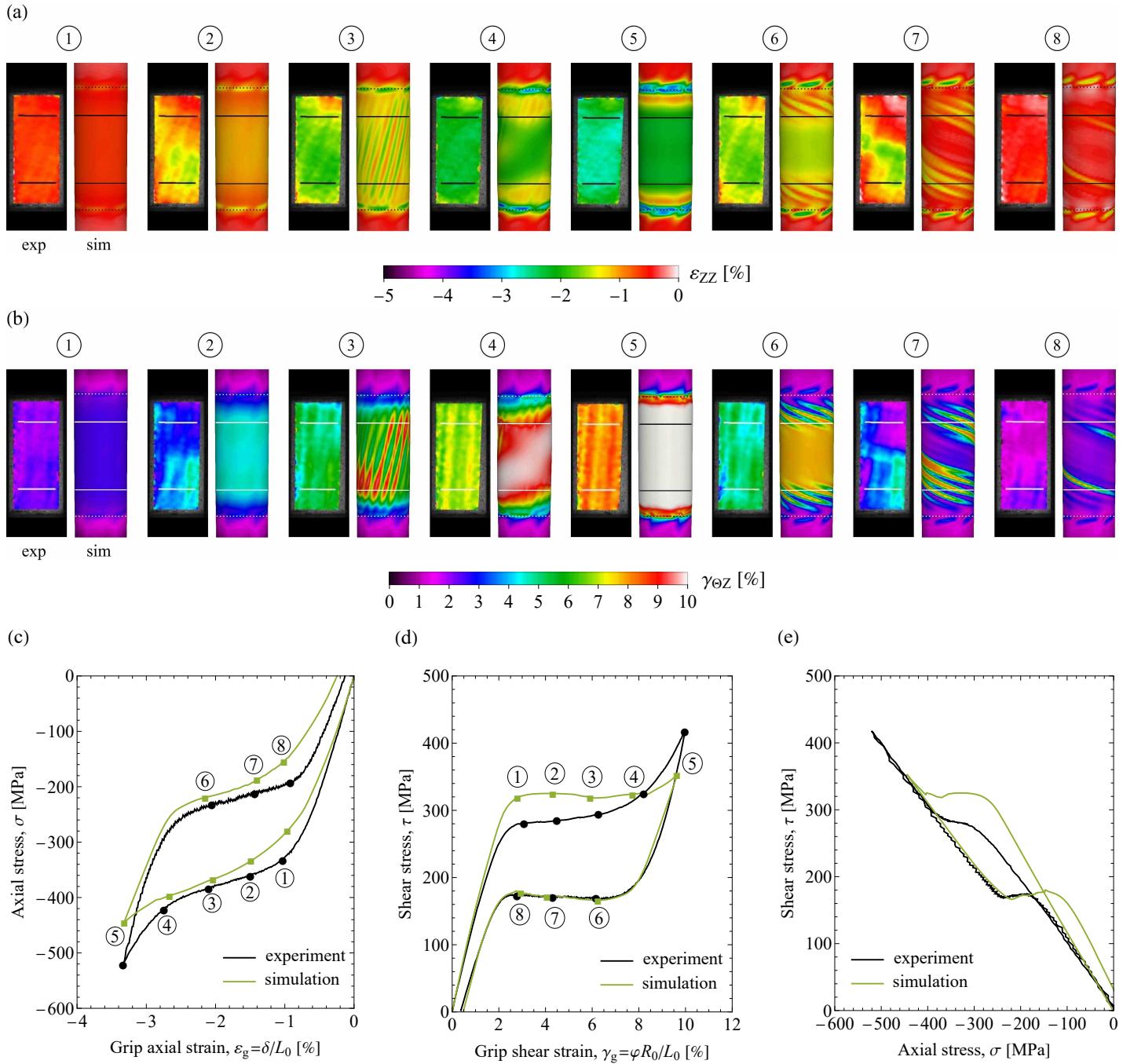
Figure 24: Simulation results for the case of combined compression-torsion at \omega = 109^\circ and their comparison with the experimental results (case P11) of Reedlunn et al. (2020a). The left-hand and right-hand snapshots in panels (a) and (b) correspond, respectively, to the experiment (reproduced with permission from Elsevier) and simulation.
