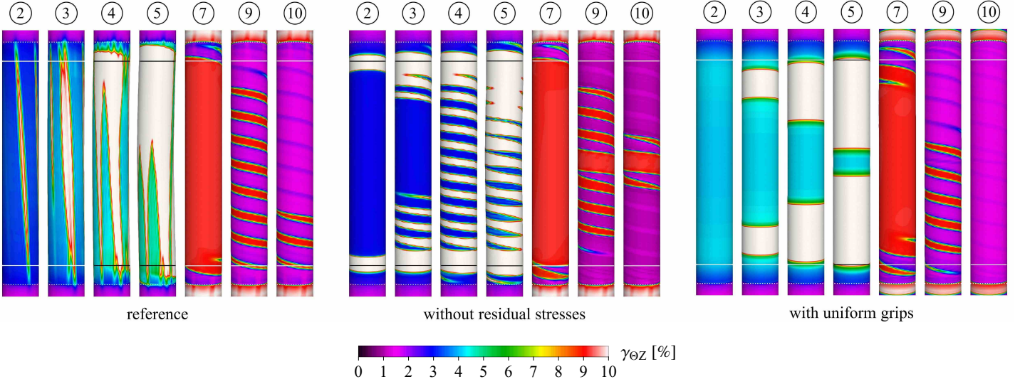
Figure 9: The impact of residual stresses and collet grips on the transformation pattern in simple torsion. In the reference simulation, both the internal stresses and the non-uniformity of the collet grips are accounted for.
