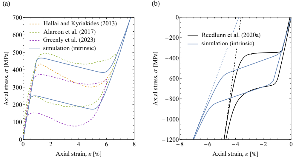
Figure 3: Comparison between the calibrated intrinsic response in tension (a) and compression (b) with the NiTi responses obtained from experiments. The dashed curves in panel (a) refer to the experimentally-determined intrinsic responses (note that only the loading stage is reported by Hallai and Kyriakides (2013)). The dashed lines in panel (b) depict the stress-free transformation strains.
