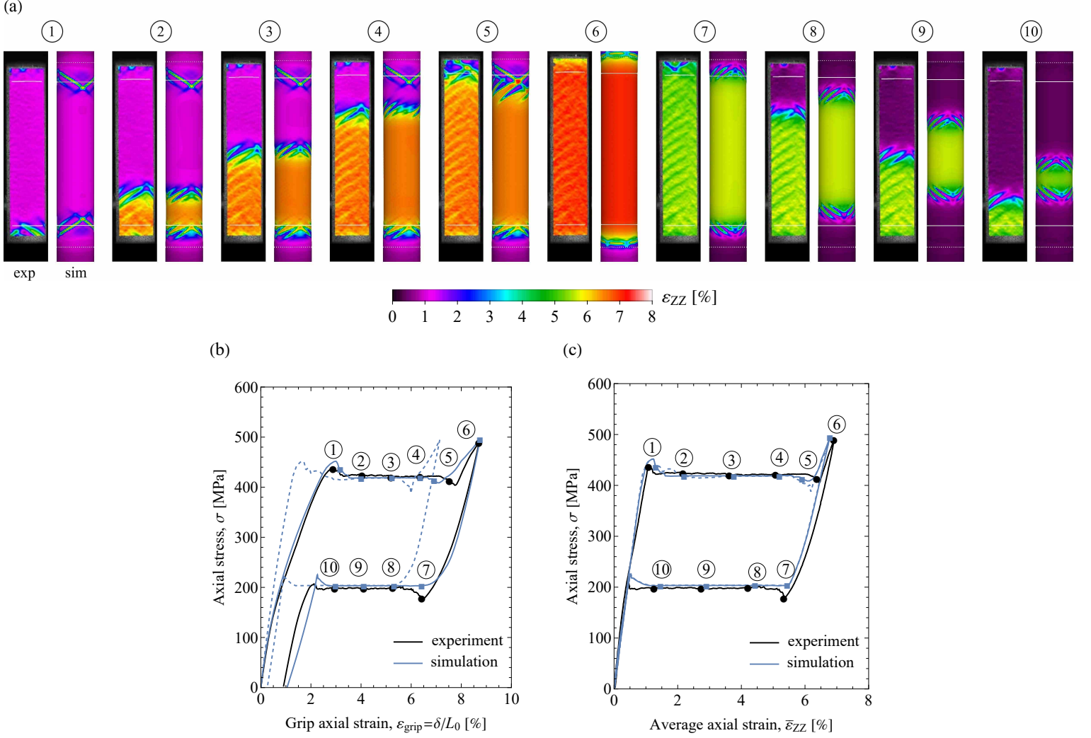
Figure 4: Simulation results for the case of uniaxial tension ( \omega = 0^\circ ) and their comparison with the experimental results (case T1) of Reedlunn et al. (2020a): (a) snapshots of the axial strain field \varepsilon_{ZZ} , (b,c) the global mechanical response represented in terms of (b) axial stress–grip axial strain ( \sigma – \varepsilon_{\text{grip}} ), and (c) axial stress–average axial strain ( \sigma – \bar{\varepsilon}_{ZZ} ). The left-hand and right-hand snapshots in panel (a) correspond, respectively, to the experiment (reproduced with permission from Elsevier) and simulation. The dashed curves in panels (b,c) represent the response for the case with the limit friction stress of T_c = 20 MPa, while the corresponding transformation pattern is shown in Fig. 6.
