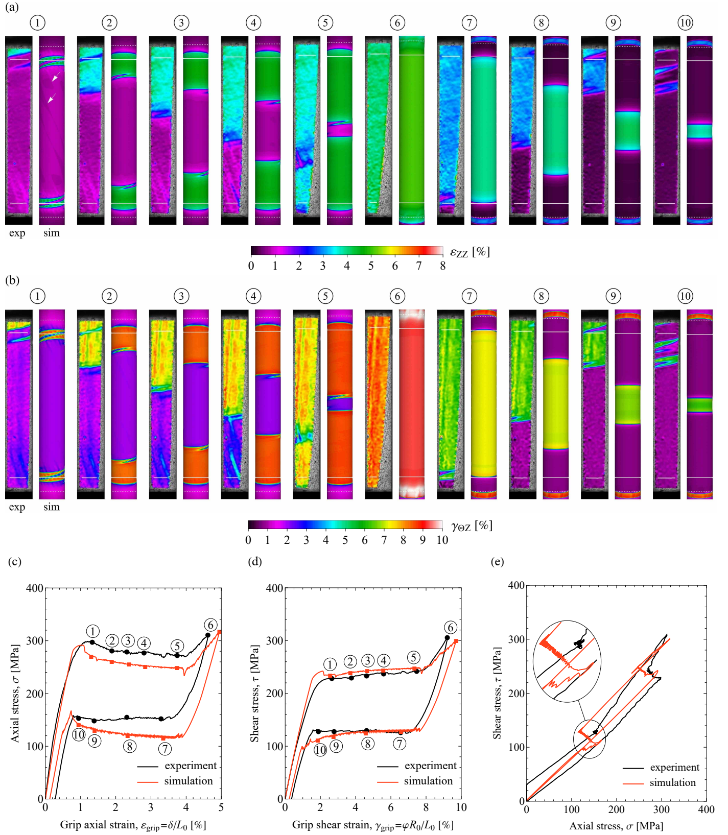
Figure 14: Simulation results for the case of combined tension–torsion at \omega = 63^\circ and their comparison with the experimental results (case P4) of Reedlunn et al. (2020a). The left-hand and right-hand snapshots in panels (a) and (b) correspond, respectively, to the experiment (reproduced with permission from Elsevier) and simulation.
