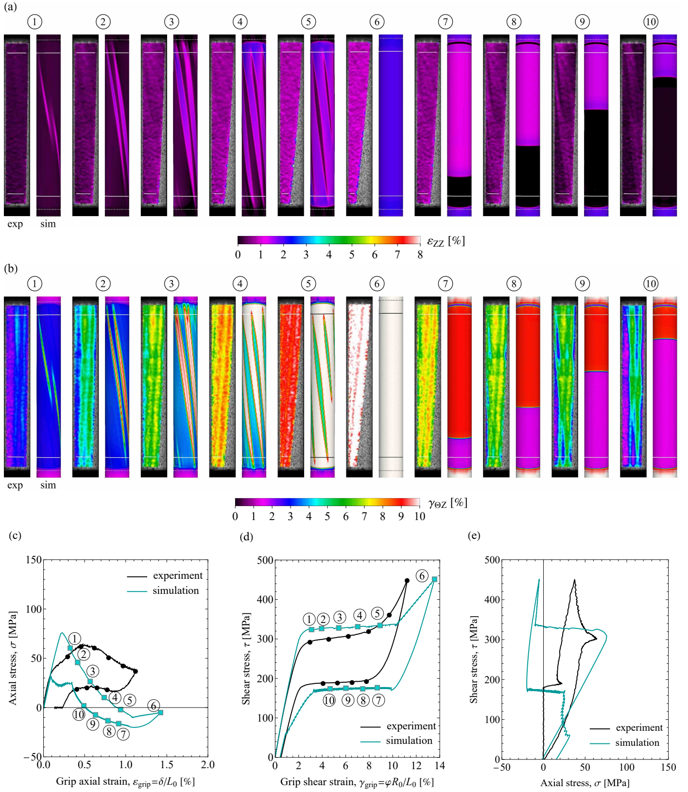
Figure 17: Simulation results for the case of combined tension–torsion at \omega = 84^\circ and their comparison with the experimental results (case P7) of Reedlunn et al. (2020a). The left-hand and right-hand snapshots in panels (a) and (b) correspond, respectively, to the experiment (reproduced with permission from Elsevier) and simulation.
