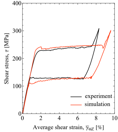
Figure F.1: Selected mechanical responses in terms of the average strains \bar{\epsilon}_{ZZ} and \bar{\gamma}_{\theta Z} and their comparison with the experimental results of Reedlunn et al. (2020a): (a) tension–torsion with \omega = 22^\circ (case P1), (b) tension–torsion with \omega = 63^\circ (case P4), and (c) compression–torsion with \omega = 102^\circ (case P10).
