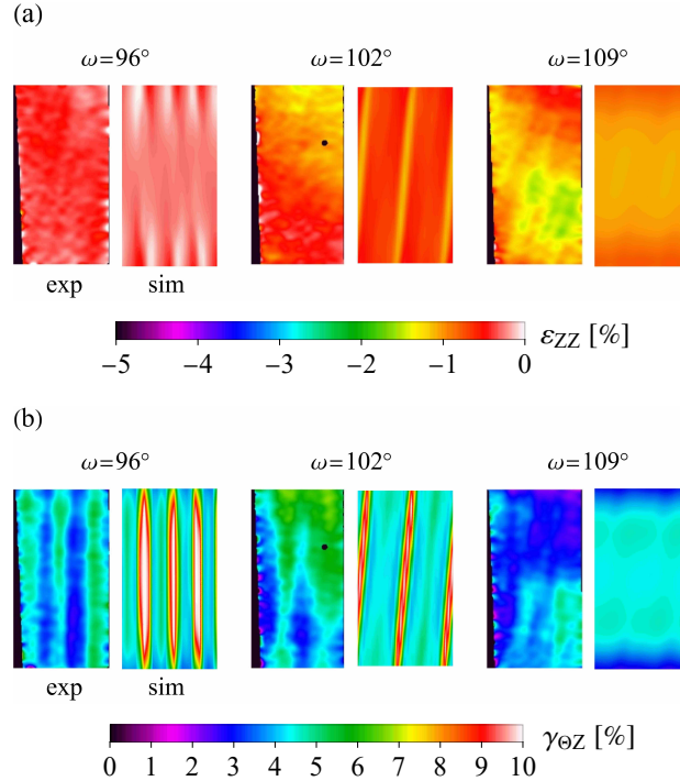
Figure 26: Close-up views of the transformation pattern (taken in the undeformed and unwrapped-tube configuration) represented by (a) the axial strain field \varepsilon_{ZZ} , and (b) the shear strain field \gamma_{\Theta Z} in combined compression-torsion. The left-hand and right-hand snapshots correspond, respectively, to the experiment (taken from Fig. 22 of Reedlunn et al. (2020a), reproduced with permission from Elsevier) and simulation.
