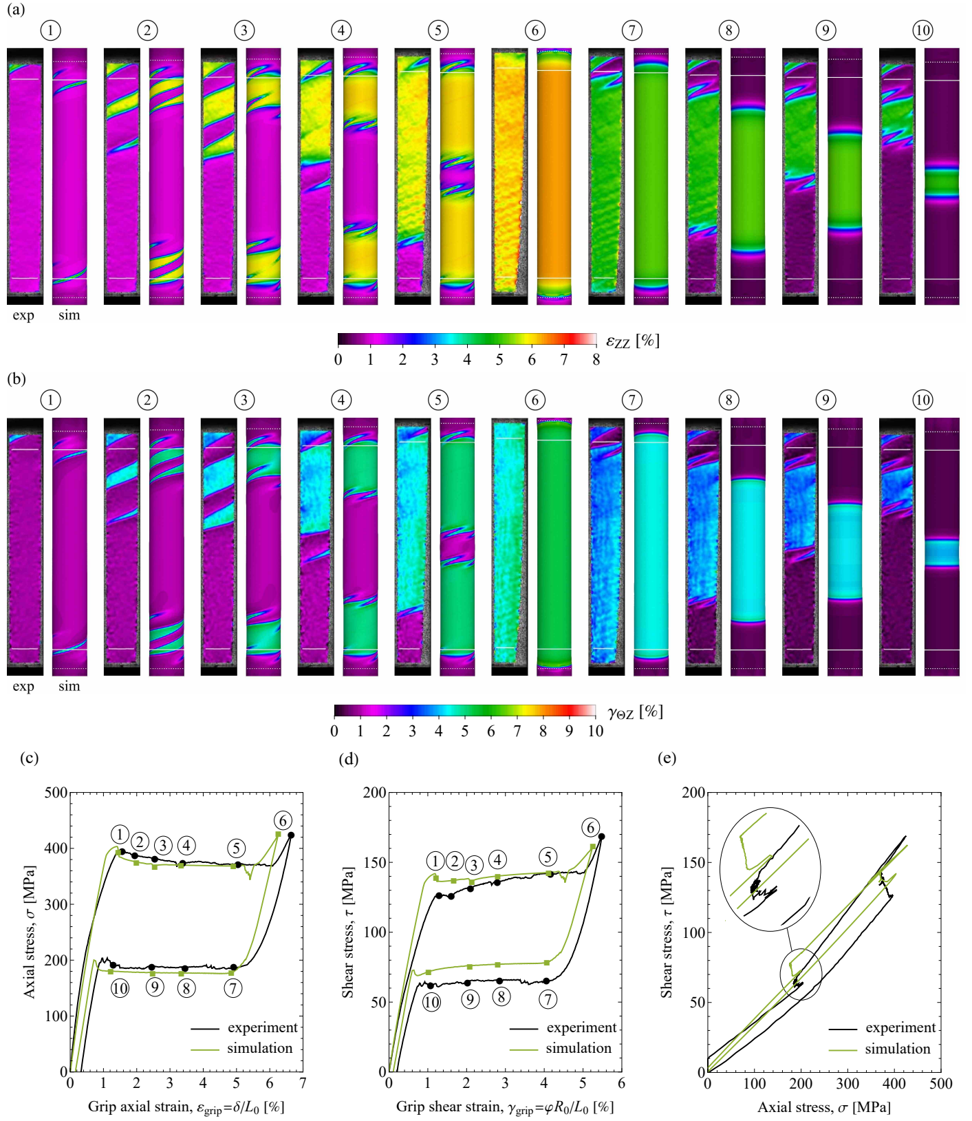
Figure 12: Simulation results for the case of combined tension–torsion at \omega = 40^\circ and their comparison with the experimental results (case P2) of Reedlunn et al. (2020a). The left-hand and right-hand snapshots in panels (a) and (b) correspond, respectively, to the experiment (reproduced with permission from Elsevier) and simulation.
