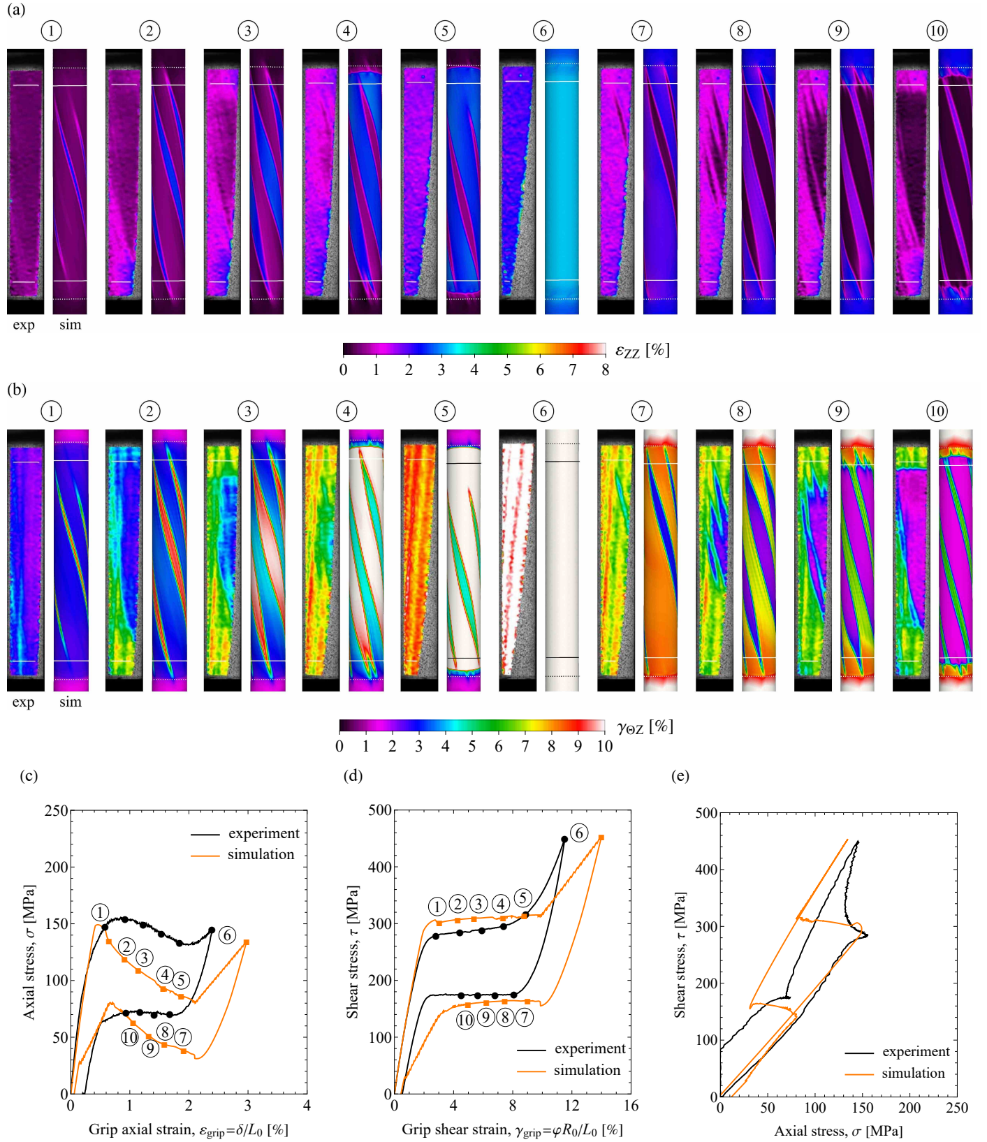
Figure 16: Simulation results for the case of combined tension–torsion at \omega = 78^\circ and their comparison with the experimental results (case P6) of Reedlunn et al. (2020a). The left-hand and right-hand snapshots in panels (a) and (b) correspond, respectively, to the experiment (reproduced with permission from Elsevier) and simulation.
