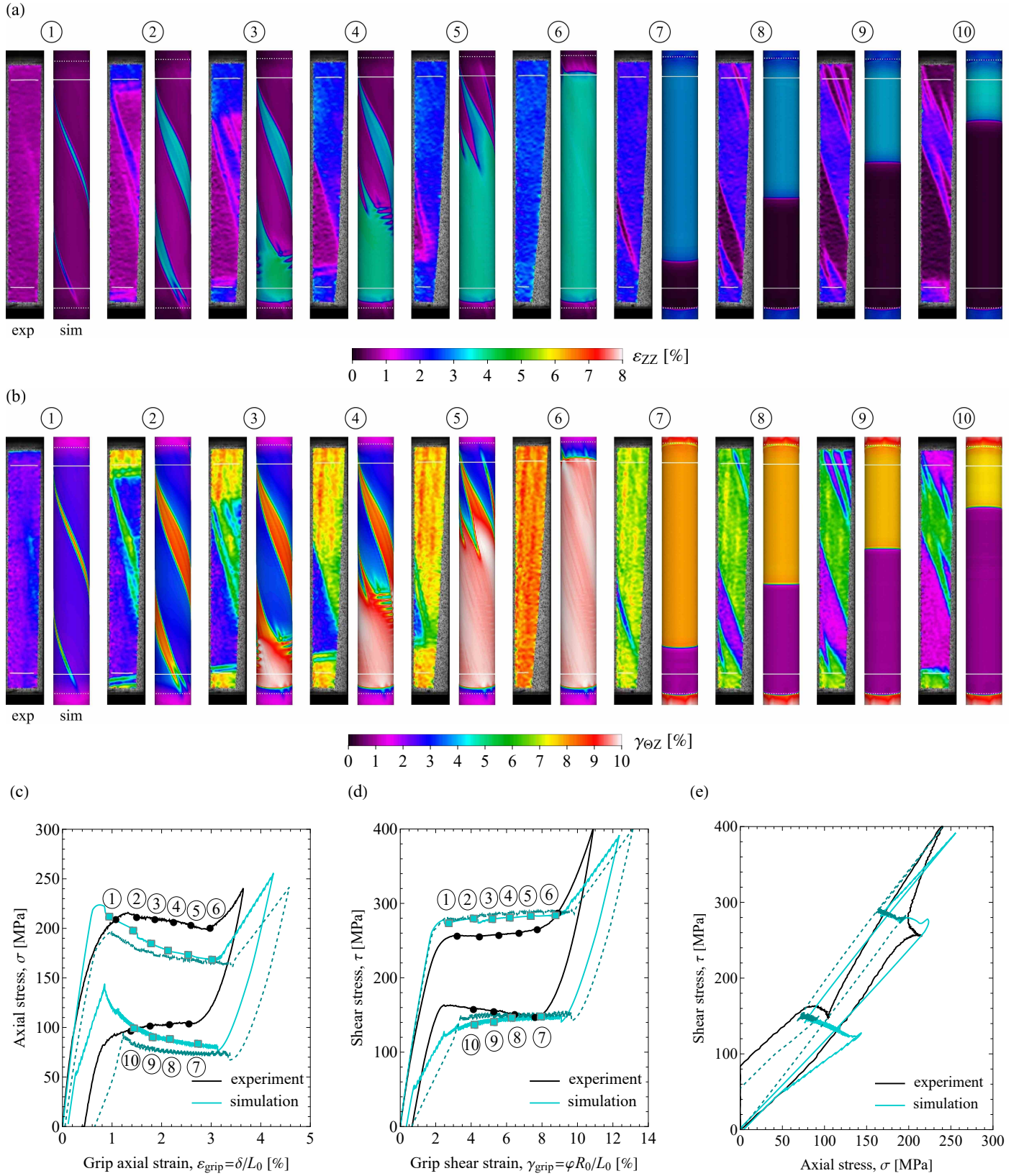
Figure 15: Simulation results for the case of combined tension–torsion at \omega = 71^\circ and their comparison with the experimental results (case P5) of Reedlunn et al. (2020a). The left-hand and right-hand snapshots in panels (a) and (b) correspond, respectively, to the experiment (reproduced with permission from Elsevier) and simulation. The dashed curves represent the mechanical response for the case with a radial compression induced by the collet grips.
