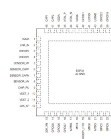
Fig. 1. ESP32 Pinout
