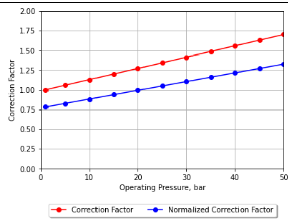
Figure S4b: Original and normalized pressure correction factor as a function of operating pressure from 1 bar to 50 bar.
