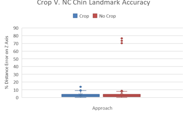
Figure 8. Box plot distribution of z-axis error for chin landmark with crop and no crop approaches.
