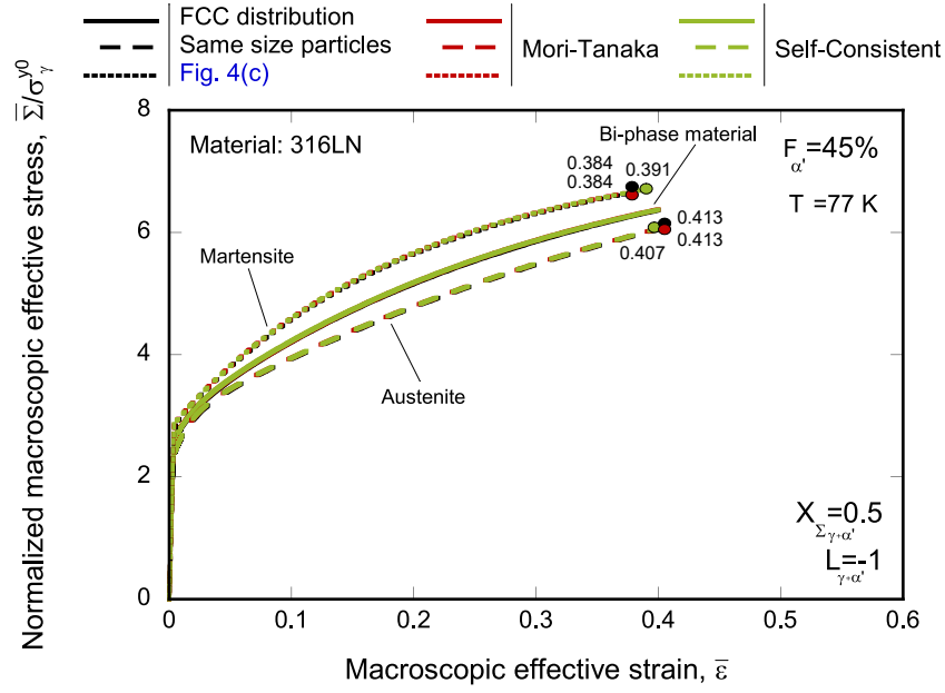
Figure C.22: Unit-cell finite element simulations. Monotonic loading. Material 316LN, temperature T = 77 K, and volume fraction of martensite F_{\alpha'} = 45\% . Comparison of Mori-Tanaka and Self-Consistent homogenization schemes with calculations corresponding to the FCC-symmetric spatial distribution of inclusions with the same size and a boundary layer devoid of particles, Fig. 4(c) . Evolution of the normalized macroscopic effective stress \bar{\Sigma}/\sigma_{\gamma}^{y0} with the macroscopic effective strain \bar{\epsilon} . Results corresponding to the bi-phase material, the austenite phase, and the martensite phase for stress triaxiality X_{\Sigma_{\gamma+\alpha'}} = 0.5 and Lode parameter L_{\gamma+\alpha'} = -1 . The colored markers indicate the maximum value of the macroscopic effective strain for a macroscopic effective strain of the bi-phase material of \bar{\epsilon}_{\gamma+\alpha'} = 0.4 . (For interpretation of the references to color in this figure legend, the reader is referred to the web version of this article.)
