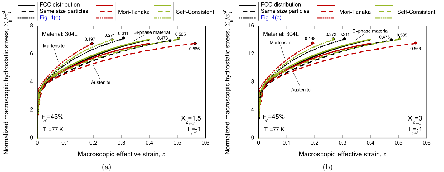
Figure 11: Unit-cell finite element simulations. Monotonic loading. Material 304L, temperature T = 77 K, and volume fraction of martensite F_{\alpha'} = 45\% . Comparison of Mori-Tanaka and Self-Consistent homogenization schemes with calculations corresponding to the FCC-symmetric spatial distribution of inclusions with the same size and a boundary layer devoid of particles , see Fig. 4(c). Evolution of the normalized macroscopic hydrostatic stress \bar{\Sigma}_h/\sigma_{\gamma}^{y0} with the macroscopic effective strain \bar{\epsilon} . Results corresponding to the bi-phase material, the austenite phase, and the martensite phase for the Lode parameter in the unit-cell L_{\gamma+\alpha'} = -1 . Stress triaxiality in the unit-cell: (a) X_{\Sigma_{\gamma+\alpha'}} = 1.5 and (b) X_{\Sigma_{\gamma+\alpha'}} = 3 . The colored markers indicate the value of the macroscopic effective strain in the individual phases for a macroscopic effective strain in the bi-phase material of \bar{\epsilon}_{\gamma+\alpha'} = 0.4 . (For interpretation of the references to color in this figure legend, the reader is referred to the web version of this article.)
