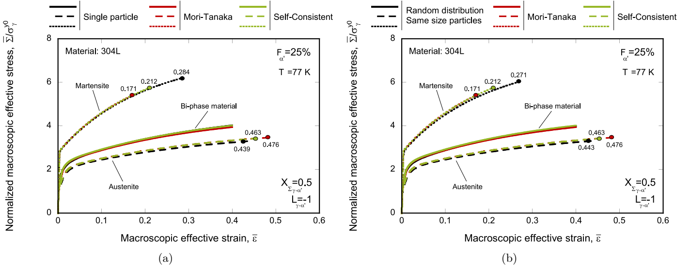
Figure 13: Unit-cell finite element simulations. Monotonic loading. Material 304L, temperature T = 77 K, and volume fraction of martensite F_{\alpha'} = 25\% . Comparison of Mori-Tanaka and Self-Consistent homogenization schemes with calculations corresponding to two different microstructures: (a) single central particle, see Fig. 4(a), and (b) random spatial distribution of inclusions with the same size and a boundary layer devoid of particles, see Fig. 4(d). Evolution of the normalized macroscopic effective stress \bar{\Sigma}/\sigma_{\gamma}^{y0} with the macroscopic effective strain \bar{\epsilon} . Results corresponding to the bi-phase material, the austenite phase, and the martensite phase for a stress triaxiality and Lode parameter in the unit-cell equal to X_{\bar{\Sigma}_{\gamma+\alpha'}} = 0.5 and L_{\gamma+\alpha'} = -1 , respectively. The colored markers indicate the value of the macroscopic effective strain in the individual phases for a macroscopic effective strain in the bi-phase material of \bar{\epsilon}_{\gamma+\alpha'} = 0.4 . (For interpretation of the references to color in this figure legend, the reader is referred to the web version of this article.)
