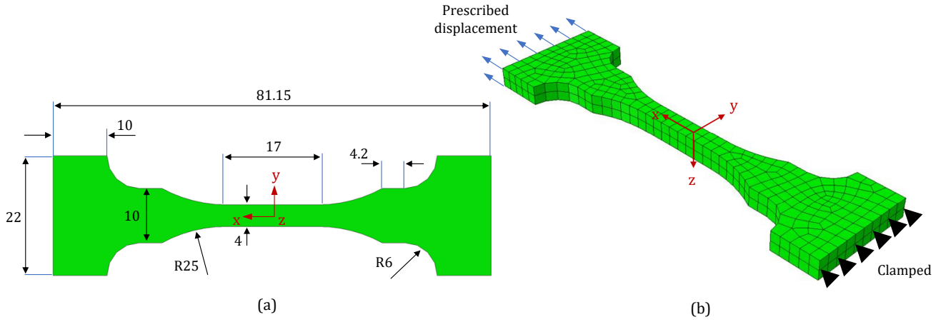
Figure 5: Tensile sample finite element model: (a) geometry and dimensions in millimeters (thickness is 4 mm), (b) mesh and boundary conditions.
