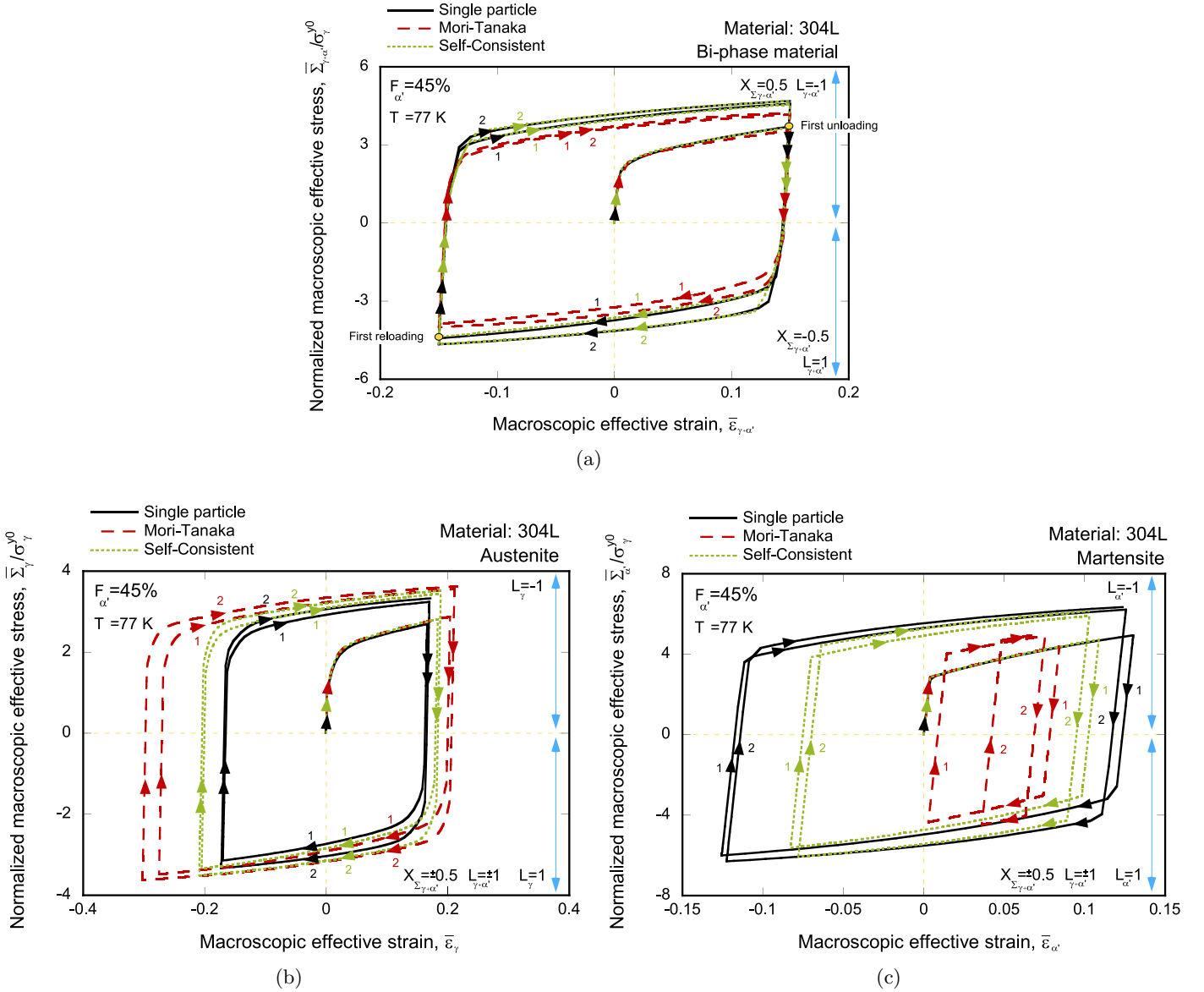
Figure 12: Unit-cell finite element simulations. Cyclic loading. Material 304L, temperature T = 77 K, and volume fraction of martensite F_{\alpha'} = 45\% . Varying stress triaxiality X_{\Sigma_{\gamma+\alpha'}} = \pm 0.5 and Lode parameter L_{\gamma+\alpha'} = \pm 1 in the unit-cell. Comparison of Mori-Tanaka and Self-Consistent homogenization schemes with calculations corresponding to a single central particle, see Fig. 4(a). Evolution of the normalized macroscopic effective stress \bar{\Sigma}/\sigma_{\gamma}^{y0} with the macroscopic effective strain \bar{\epsilon} varying the macroscopic effective strain of the bi-phase material between 0.15 and -0.15 . Results corresponding to: (a) bi-phase material, (b) austenite phase, and (c) martensite phase. The colored arrows and numbers indicate the loading sequence and order of cycles. (For interpretation of the references to color in this figure legend, the reader is referred to the web version of this article.)
