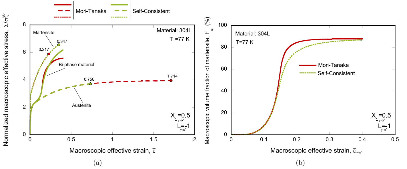
Figure 15: Unit-cell finite element simulations. Monotonic loading. Material 304L, temperature T = 77 K. Stress triaxiality and Lode parameter in the unit-cell are X_{\Sigma_{\gamma+\alpha'}} = 0.5 and L_{\gamma+\alpha'} = -1 , respectively. Comparison of Mori-Tanaka and Self-Consistent homogenization schemes. (a) Evolution of the normalized macroscopic effective stress \bar{\Sigma}/\sigma_{\gamma}^{y0} with the macroscopic effective strain \bar{\epsilon} . The red and green markers indicate the value of the macroscopic effective strain in the individual phases for a macroscopic effective strain in the bi-phase material of \bar{\epsilon}_{\gamma+\alpha'} = 0.4 . (b) Evolution of the macroscopic volume fraction of martensite F_{\alpha'} (%) with the macroscopic effective strain in the bi-phase material \bar{\epsilon}_{\gamma+\alpha'} . (For interpretation of the references to color in this figure legend, the reader is referred to the web version of this article.)
