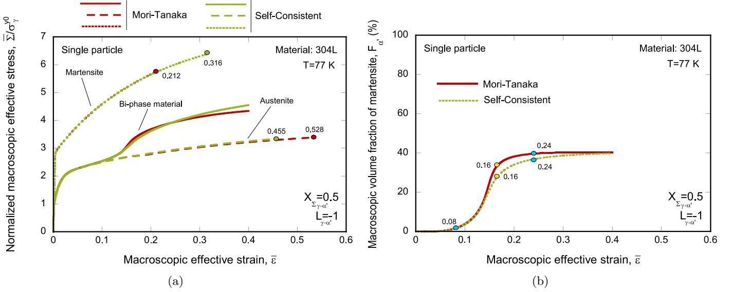
Figure 16: Unit-cell finite element simulations. Monotonic loading. Material 304L, temperature T = 77 K. Stress triaxiality and Lode parameter in the unit-cell are X_{\Sigma_{\gamma+\alpha'}} = 0.5 and L_{\gamma+\alpha'} = -1 , respectively. Comparison of Mori-Tanaka and Self-Consistent homogenization schemes. The unit-cell contains an austenite inclusion of 45% volume, which is modeled with Mori-Tanaka and Self-Consistent homogenization schemes, separately, while accounting for the martensitic transformation in a non-transforming austenite matrix. (a) Evolution of the normalized macroscopic effective stress \bar{\Sigma}/\sigma_{\gamma}^0 with the macroscopic effective strain \bar{\epsilon} . The red and green markers indicate the value of the macroscopic effective strain in the individual phases for a macroscopic effective strain in the bi-phase material of \bar{\epsilon}_{\gamma+\alpha'} = 0.4 . (b) Evolution of the macroscopic volume fraction of martensite F_{\alpha'} (%) with the macroscopic effective strain in the bi-phase material \bar{\epsilon}_{\gamma+\alpha'} . The yellow markers indicate the value of the macroscopic effective strain in the bi-phase material corresponding to the maximum difference in the martensite volume fraction between the Mori-Tanaka and Self-Consistent models (for this strain value, the contours and evolution of the microscopic volume fraction of martensite are shown in Figs. 17 and 18, respectively). The blue markers correspond to values of the macroscopic effective strain in the bi-phase material of 0.08 and 0.24 (for these strain values, the evolution of the microscopic volume fraction of martensite is also shown in Fig. 18). (For interpretation of the references to color in this figure legend, the reader is referred to the web version of this article.)
