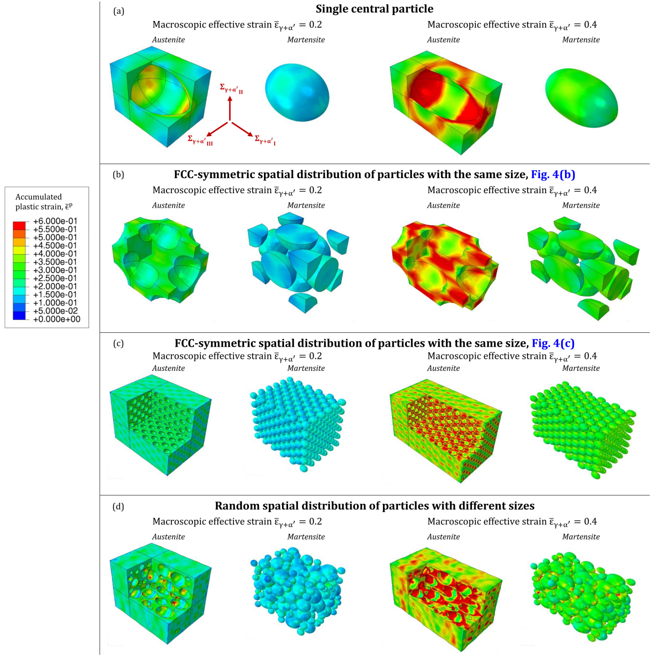
Figure 8: Unit-cell finite element simulations. Monotonic loading. Material 304L, temperature T = 77 K, and volume fraction of martensite F_{\alpha'} = 45\% . Contours of accumulated plastic strain \bar{\epsilon}^p for calculations corresponding to different microstructures: (a) single central particle, Fig. 4(a), (b) FCC-symmetric spatial distribution of inclusions with the same size and particles intersecting the boundaries, Fig. 4(b), (c) FCC-symmetric spatial distribution of inclusions with the same size and a boundary layer devoid of particles, Fig. 4(c), and (d) random spatial distribution of particles with different sizes, Fig. 4(e). Stress triaxiality and Lode parameter in the unit-cell: X_{\Sigma_{\gamma+\alpha'}} = 0.5 and L_{\gamma+\alpha'} = -1 , respectively. (For interpretation of the references to color in this figure legend, the reader is referred to the web version of this article.)
