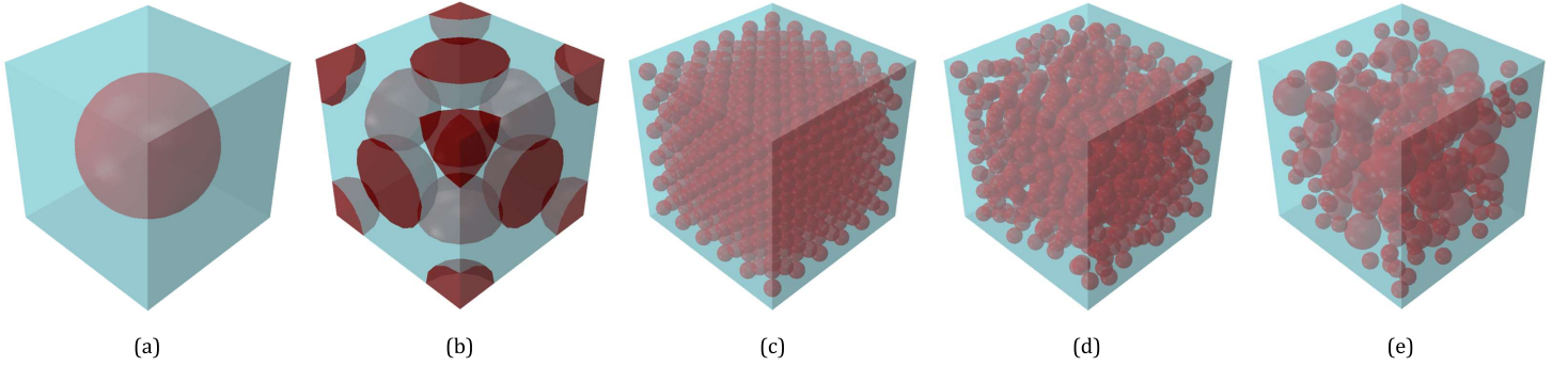
Figure 4: Unit-cell finite element model with explicit depiction of the martensite inclusions colored in red and the austenite matrix colored in blue: (a) single central inclusion, (b) representative volume element of a FCC-symmetric spatial distribution of inclusions with the same size and particles intersecting the boundaries, (c) FCC-symmetric spatial distribution of inclusions with the same size and a boundary layer devoid of particles, (d) random spatial distribution of inclusions with the same size and a boundary layer devoid of particles, and (e) random spatial distribution of inclusions with different sizes and a boundary layer devoid of particles. The finite element models correspond to the case of F_{\alpha'} = 25\% .
