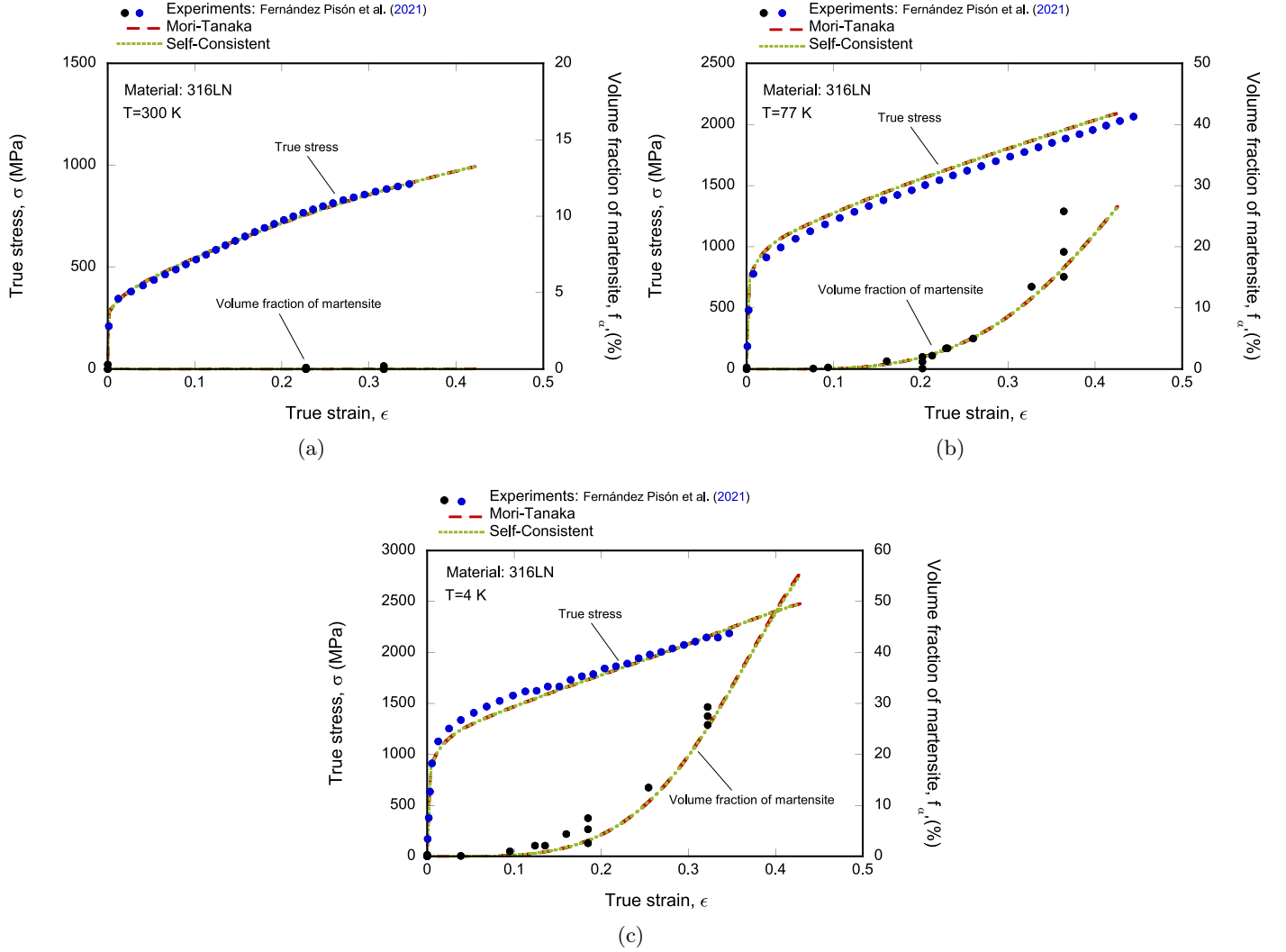
Figure 20: Tensile test finite element simulations. Material 316LN. Evolution of the true stress \sigma and the volume fraction of martensite f_{\alpha'} versus the true strain \epsilon for calculations performed with Mori-Tanaka and Self-Consistent homogenization schemes accounting for the martensitic transformation in an initial fully austenitic material. Comparison with the experimental results reported in Fernández-Pisón et al. (2021). Temperature: (a) T = 300 K, (b) T = 77 K, and (c) T = 4 K. (For interpretation of the references to color in this figure legend, the reader is referred to the web version of this article.)
