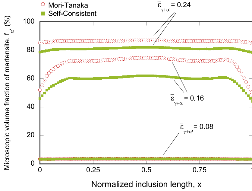
Figure 18: Unit-cell finite element simulations. Monotonic loading. Material 304L and temperature T = 77 K. Comparison of Mori-Tanaka and Self-Consistent homogenization schemes. Calculations corresponding to a single austenite inclusion of 45% volume, which is modeled with Mori-Tanaka and Self-Consistent homogenization schemes, while accounting for the martensitic transformation in a fully non-evolving austenite matrix. Evolution of the microscopic volume fraction of martensite f_{\alpha'} (%) along the normalized major semi-axis of the inclusion \bar{x} , see white solid line in Fig. 17. The data correspond to three values of the macroscopic effective strain in the bi-phase material of \bar{\epsilon}_{\gamma+\alpha'} : 0.08, 0.16 and 0.24. The corresponding values of the macroscopic volume fraction are: F_{\alpha'} = 1.5\% , 33% and 40%, and F_{\alpha'} = 1.5\% , 27% and 37%, for the Mori-Tanaka and Self-Consistent homogenization schemes, respectively (see the yellow and blue markers in Fig. 16(b)). (For interpretation of the references to color in this figure legend, the reader is referred to the web version of this article.)
