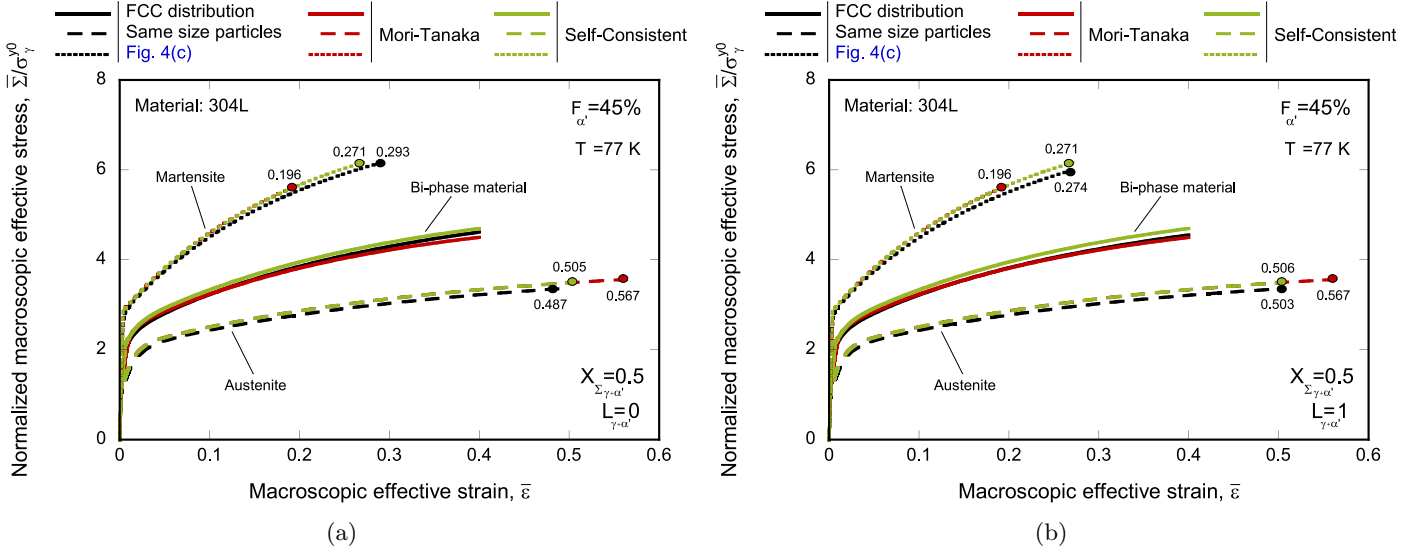
Figure 9: Unit-cell finite element simulations. Monotonic loading. Material 304L, temperature T = 77 K, and volume fraction of martensite F_{\alpha'} = 45\% . Comparison of Mori-Tanaka and Self-Consistent homogenization schemes with calculations corresponding to the FCC-symmetric spatial distribution of inclusions with the same size and a boundary layer devoid of particles, see Fig. 4(c) . Evolution of the normalized macroscopic effective stress \bar{\Sigma}/\sigma_{\gamma}^{y0} with the macroscopic effective strain \bar{\epsilon} . Results corresponding to the bi-phase material, the austenite phase, and the martensite phase for stress triaxiality in the unit-cell X_{\Sigma_{\gamma+\alpha'}} = 0.5 . Lode parameter in the unit-cell: (a) L_{\gamma+\alpha'} = 0 and (b) L_{\gamma+\alpha'} = 1 . The colored markers indicate the value of the macroscopic effective strain in the individual phases for a macroscopic effective strain in the bi-phase material of \bar{\epsilon}_{\gamma+\alpha'} = 0.4 . (For interpretation of the references to color in this figure legend, the reader is referred to the web version of this article.)
