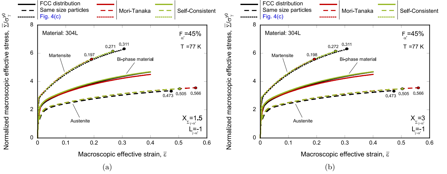
Figure 10: Unit-cell finite element simulations. Monotonic loading. Material 304L, temperature T = 77 K, and volume fraction of martensite F_{\alpha'} = 45\% . Comparison of Mori-Tanaka and Self-Consistent homogenization schemes with calculations corresponding to the FCC-symmetric spatial distribution of inclusions with the same size and a boundary layer devoid of particles , see Fig. 4(c). Evolution of the normalized macroscopic effective stress \bar{\Sigma}/\sigma_{\gamma}^{y0} with the macroscopic effective strain \bar{\epsilon} . Results corresponding to the bi-phase material, the austenite phase, and the martensite phase for the Lode parameter in the unit-cell L_{\gamma+\alpha'} = -1 . Stress triaxiality in the unit-cell: (a) X_{\Sigma_{\gamma+\alpha'}} = 1.5 and (b) X_{\Sigma_{\gamma+\alpha'}} = 3 . The colored markers indicate the value of the macroscopic effective strain in the individual phases for a macroscopic effective strain in the bi-phase material of \bar{\epsilon}_{\gamma+\alpha'} = 0.4 . (For interpretation of the references to color in this figure legend, the reader is referred to the web version of this article.)
