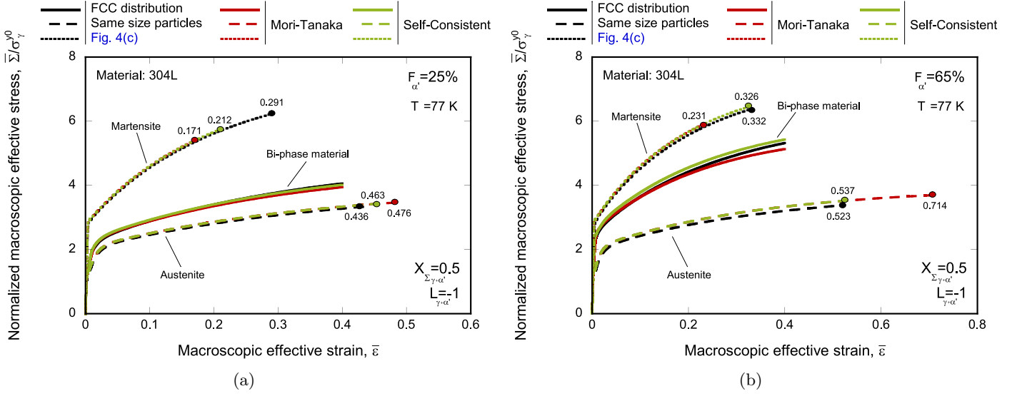
Figure 14: Unit-cell finite element simulations. Monotonic loading. Material 304L, temperature T = 77 K. Comparison of Mori-Tanaka and Self-Consistent homogenization schemes with calculations corresponding to the FCC-symmetric spatial distribution of inclusions with the same size and a boundary layer devoid of particles, see Fig. 4(c) , for two volume fractions of martensite: (a) F_{\alpha'} = 25\% and (b) F_{\alpha'} = 65\% . Evolution of the normalized macroscopic effective stress \bar{\Sigma}/\sigma_{\gamma}^{y0} with the macroscopic effective strain \bar{\epsilon} . Results corresponding to the bi-phase material, the austenite phase, and the martensite phase for a stress triaxiality and Lode parameter in the unit-cell equal to X_{\Sigma_{\gamma+\alpha'}} = 0.5 and L_{\gamma+\alpha'} = -1 , respectively. The colored markers indicate the value of the macroscopic effective strain in the individual phases for a macroscopic effective strain in the bi-phase material of \bar{\epsilon}_{\gamma+\alpha'} = 0.4 . (For interpretation of the references to color in this figure legend, the reader is referred to the web version of this article.)
