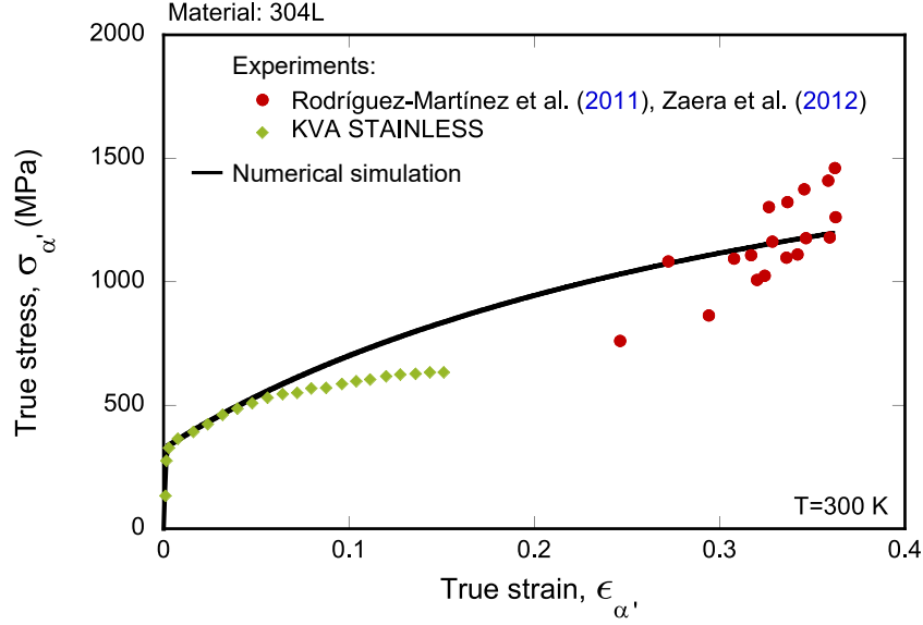
Figure 2: Comparison of the stress-strain curve for the martensite phase resulting from the calibration performed in this work for AISI 304L and experimental data at T = 300 K. The results of the simulations are shown with a black solid line. The experimental data from Rodríguez-Martínez et al. (2011) and Zaera et al. (2012), red markers, corresponds to the mechanical behavior of the single martensite phase on AISI 304 samples. The experimental data supplied by the manufacturer KVA STAINLESS, green markers, corresponds to a martensitic stainless steel AISI 410 (Data source: https://www.kvastainless.com ).
