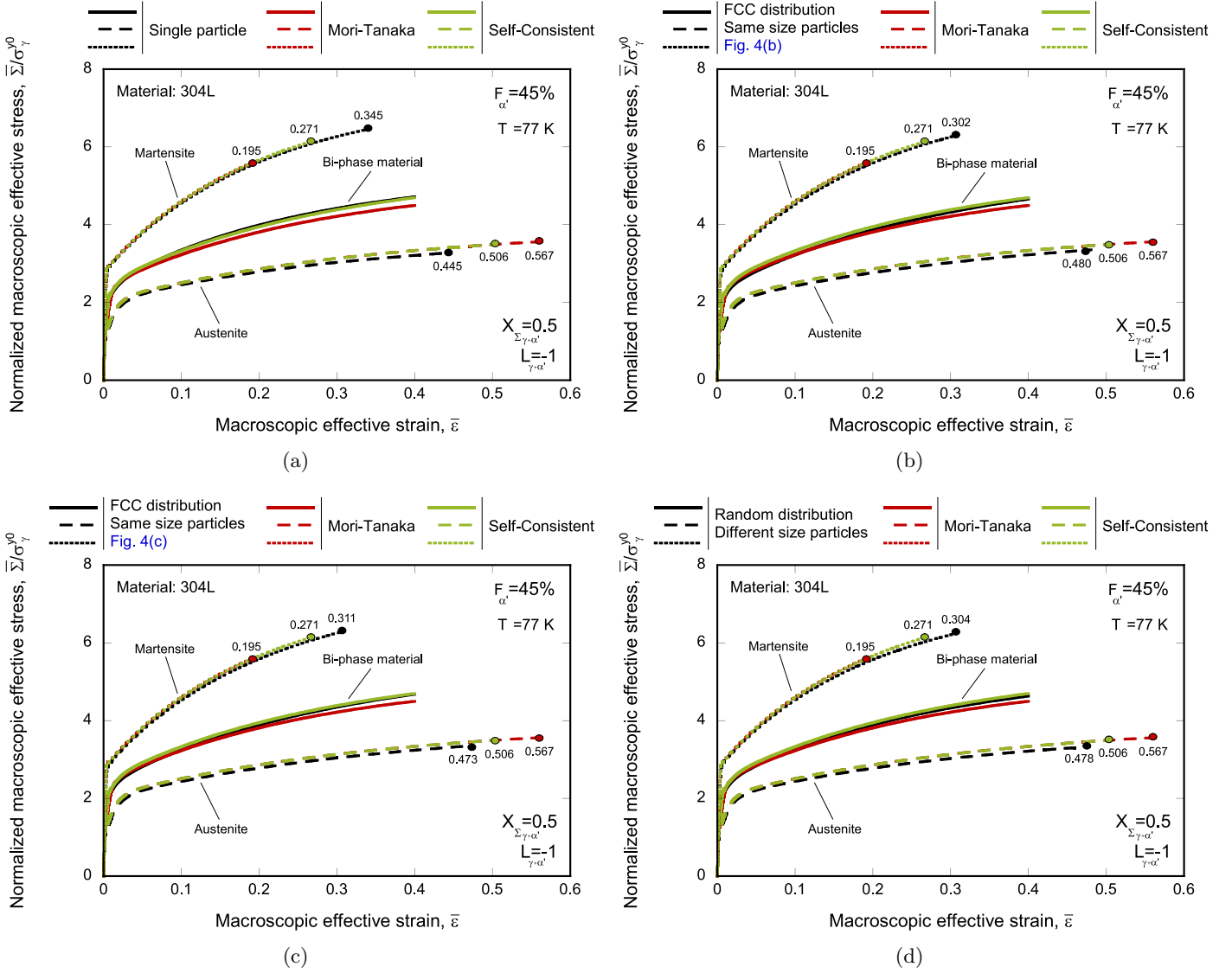
Figure 6: Unit-cell finite element simulations. Monotonic loading. Material 304L, temperature T = 77 K, and volume fraction of martensite F_{\alpha'} = 45\% . Comparison of Mori-Tanaka and Self-Consistent homogenization schemes with calculations corresponding to different microstructures: (a) single central particle, Fig. 4(a), (b) FCC-symmetric spatial distribution of inclusions with the same size and particles intersecting the boundaries, Fig. 4(b), (c) FCC-symmetric spatial distribution of inclusions with the same size and a boundary layer devoid of particles, Fig. 4(c), and (d) random spatial distribution of particles with different sizes, Fig. 4(e). Evolution of the normalized macroscopic effective stress \bar{\Sigma}/\sigma_{\gamma}^0 with the macroscopic effective strain \bar{\epsilon} . Results corresponding to the bi-phase material, the austenite phase, and the martensite phase for a stress triaxiality and Lode parameter in the unit-cell equal to X_{\Sigma_{\gamma+\alpha'}} = 0.5 and L_{\gamma+\alpha'} = -1 , respectively. The colored markers indicate the value of the macroscopic effective strain in the individual phases for a macroscopic effective strain in the bi-phase material of \bar{\epsilon}_{\gamma+\alpha'} = 0.4 . (For interpretation of the references to color in this figure legend, the reader is referred to the web version of this article.)
