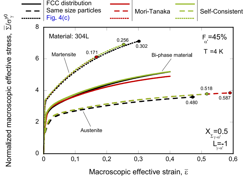
Figure B.21: Unit-cell finite element simulations. Monotonic loading. Material 304L, temperature T = 4 K, and volume fraction of martensite F_{\alpha'} = 45\% . Comparison of Mori-Tanaka and Self-Consistent homogenization schemes with calculations corresponding to the FCC-symmetric spatial distribution of inclusions with the same size and a boundary layer devoid of particles, Fig. 4(c) . Evolution of the normalized macroscopic effective stress \bar{\Sigma}/\sigma_{\gamma}^{y0} with the macroscopic effective strain \bar{\epsilon} . Results corresponding to the bi-phase material, the austenite phase, and the martensite phase for stress triaxiality X_{\Sigma_{\gamma+\alpha'}} = 0.5 and Lode parameter L_{\gamma+\alpha'} = -1 . The colored markers indicate the maximum value of the macroscopic effective strain for the individual phases for a macroscopic effective strain of the bi-phase material of \bar{\epsilon}_{\gamma+\alpha'} = 0.4 . (For interpretation of the references to color in this figure legend, the reader is referred to the web version of this article.)
