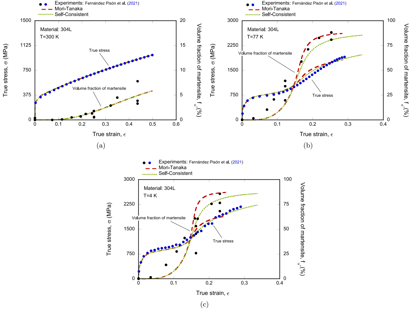
Figure 19: Tensile test finite element simulations. Material 304L. Evolution of the true stress \sigma and the volume fraction of martensite f_v versus the true strain \epsilon for calculations performed with Mori-Tanaka and Self-Consistent homogenization schemes accounting for the martensitic transformation in an initial fully austenitic material. Comparison with the experimental results reported in Fernández-Pisón et al. (2021). Temperature: (a) T = 300 K, (b) T = 77 K, and (c) T = 4 K. (For interpretation of the references to color in this figure legend, the reader is referred to the web version of this article.)
