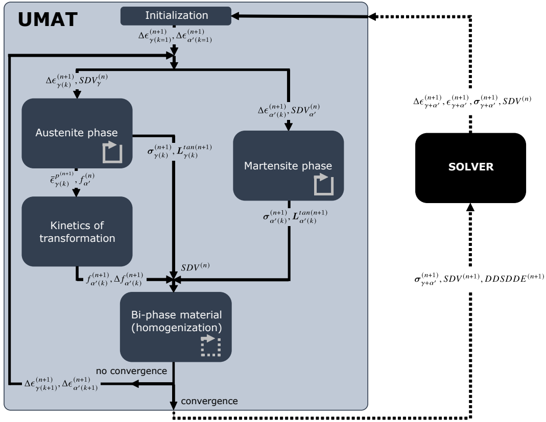
Figure 1: Sketch of the implementation of the homogenized constitutive model (Mori-Tanaka or Self-Consistent scheme) in ABAQUS/Standard.
