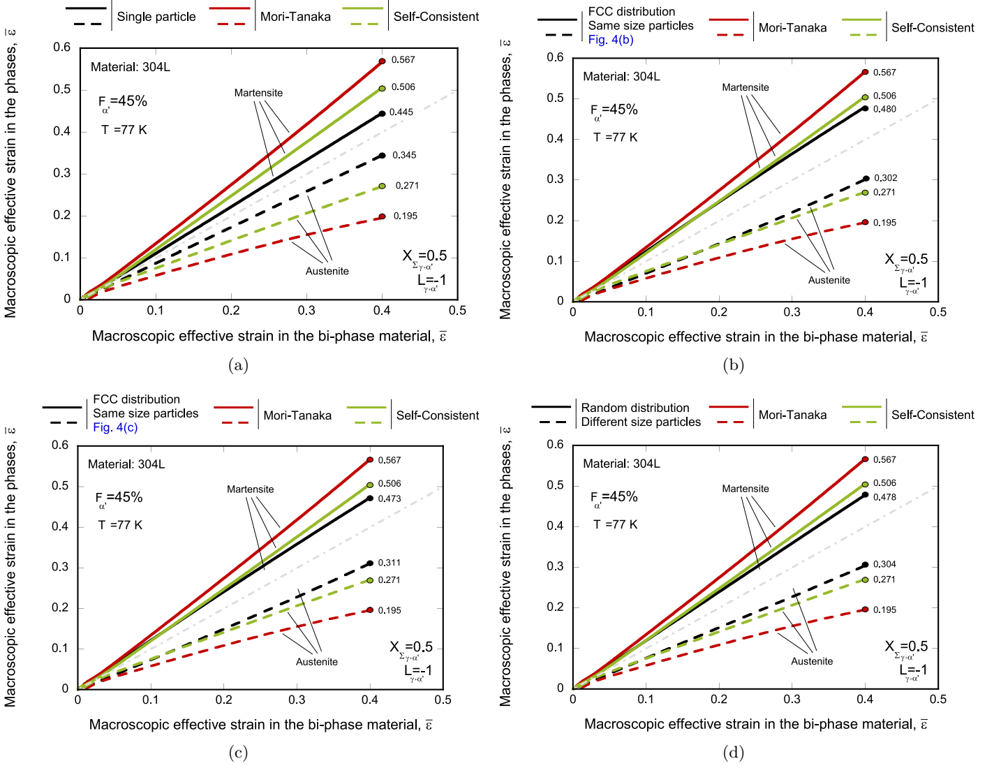
Figure 7: Unit-cell finite element simulations. Monotonic loading. Material 304L, temperature T = 77 K, and volume fraction of martensite F_{\alpha'} = 45\% . Comparison of Mori-Tanaka and Self-Consistent homogenization schemes with calculations corresponding to different microstructures: (a) single central particle, Fig. 4(a), (b) FCC-symmetric spatial distribution of inclusions with the same size and particles intersecting the boundaries, Fig. 4(b), (c) FCC-symmetric spatial distribution of inclusions with the same size and a boundary layer devoid of particles, Fig. 4(c), and (d) random spatial distribution of particles with different sizes, Fig. 4(e). Evolution of the macroscopic effective strain in the austenite \bar{\epsilon}_{\gamma} and the martensite \bar{\epsilon}_{\alpha'} with the macroscopic effective strain in the bi-phase material \bar{\epsilon}_{\gamma+\alpha'} . Results for a stress triaxiality and Lode parameter in the unit-cell equal to X_{\Sigma_{\gamma+\alpha'}} = 0.5 and L_{\gamma+\alpha'} = -1 , respectively. The colored markers indicate the value of the macroscopic effective strain in the individual phases for a macroscopic effective strain in the bi-phase material of \bar{\epsilon}_{\gamma+\alpha'} = 0.4 . (For interpretation of the references to color in this figure legend, the reader is referred to the web version of this article.)
