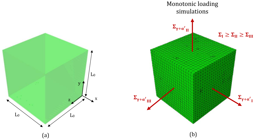
Figure 3: Cubic unit-cell finite element model: (a) dimensions and Cartesian coordinate system (x, y, z) , (b) loading directions for the case of monotonic loading simulations with \Sigma_{\gamma+\alpha'_{I}} , \Sigma_{\gamma+\alpha'_{II}} , and \Sigma_{\gamma+\alpha'_{III}} being the principal values of the macroscopic stress tensor of the bi-phase material.
