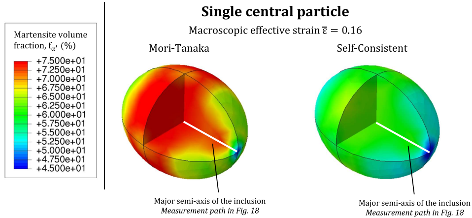
Figure 17: Unit-cell finite element simulations. Monotonic loading. Material 304L and temperature T = 77 K. Contours of the microscopic volume fraction of martensite f_{\alpha'} (%) for calculations corresponding to a single austenite inclusion of 45% volume, which is modeled with Mori-Tanaka and Self-Consistent homogenization schemes, separately, while accounting for the martensitic transformation in a fully non-evolving austenite matrix. The plots correspond to a macroscopic effective strain in the bi-phase material of \bar{\epsilon}_{\gamma+\alpha'} = 0.16 and a macroscopic volume fraction of F_{\alpha'} = 33\% and F_{\alpha'} = 27\% for the Mori-Tanaka and Self-Consistent homogenization schemes, respectively (see the yellow marker in Fig. 16(b)). The white solid line included in the figure indicates the major semi-axis of the inclusion, which corresponds to the measurement path used in Fig. 18. (For interpretation of the references to color in this figure legend, the reader is referred to the web version of this article.)
