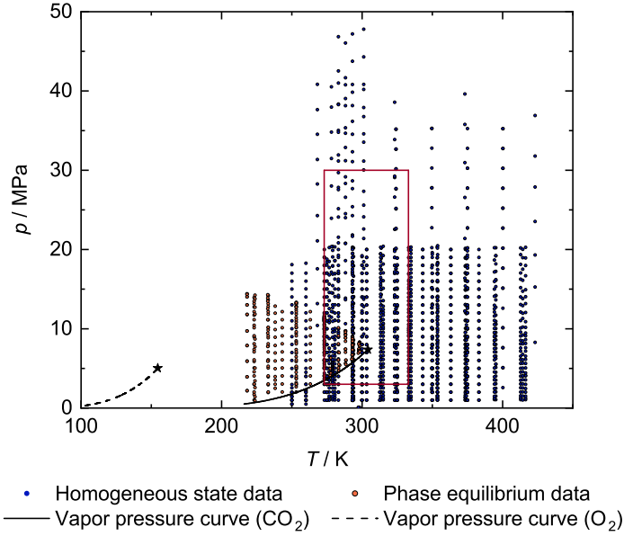
Fig. 1 Pressure-temperature diagram with the homogeneous state data and phase equilibrium data compiled in the database, cf. Table 1 and 2. Additionally, the vapor pressure curves of \text{CO}_2 and \text{O}_2 are shown (computed from the reference EOS models from Refs. [30, 43]). The star indicates the critical points. The area of the training data is marked by the red box.
