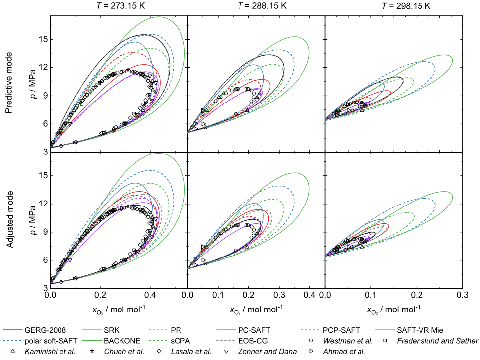
Fig. 2 Phase envelope of the system \text{CO}_2 + \text{O}_2 calculated by different EOS (lines) compared to literature data (symbols) [4, 6, 61, 63–66]. Results from predictions based on pure component models (top) are compared to results that were obtained after adjusting binary parameters (bottom) to the training data. The GERG-2008 and EOS-CG results collapse to one line in the top figures (predictive mode). For details, see text.
