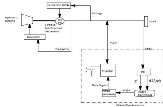
Fig -2: Proposed Scheme of VSM
