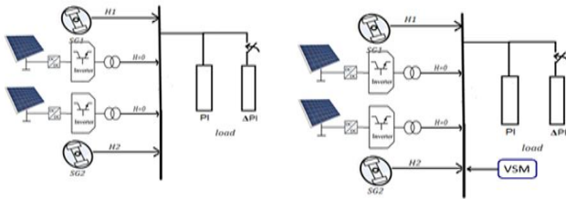
Fig -1: Micro-grid without VSM and with VSM
