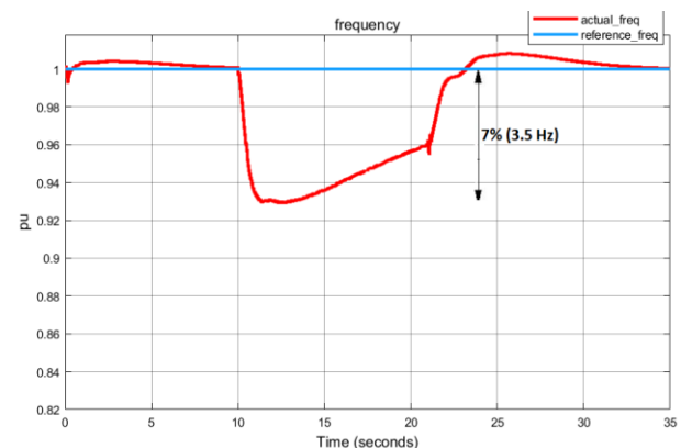
Fig -8: Frequency plot after using VSM
