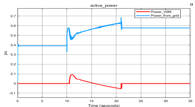
Fig -9: Active Power from grid and VSM
