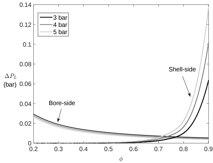
Figure 4: Bore-side (feed) and shell-side (permeate) hydraulic losses as a function of module packing density and applied pressure. Except for \phi and its corresponding RR , all nominal specifications were fixed at the values reported in Table 1.
