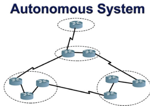
Figure 3:Autonomous System
