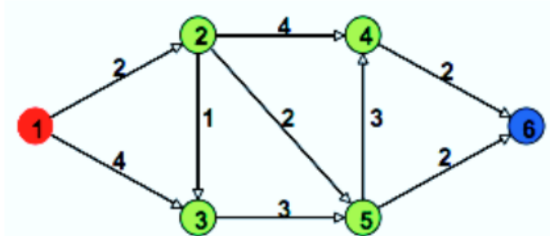
Figure 5:Source is 1 and Destination is 6, shortest path is (1, 2, 5, 6) with value 6
