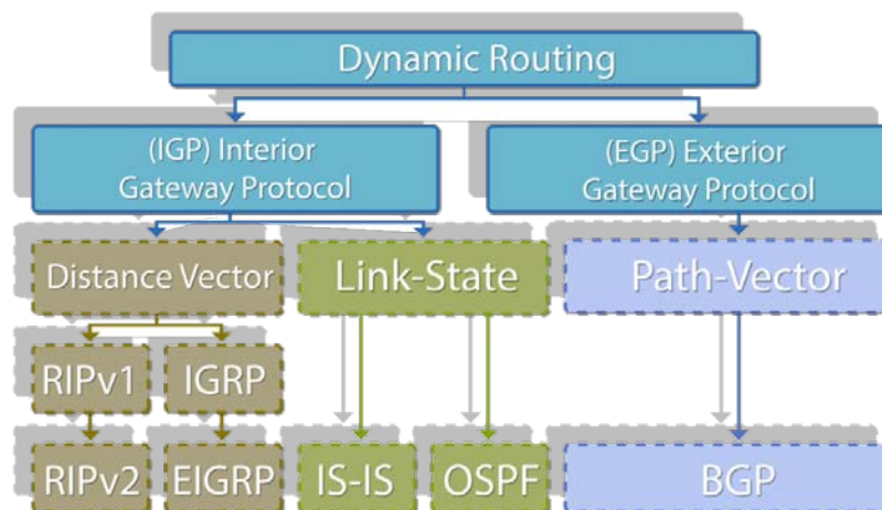
Figure 1: Routing Protocols
