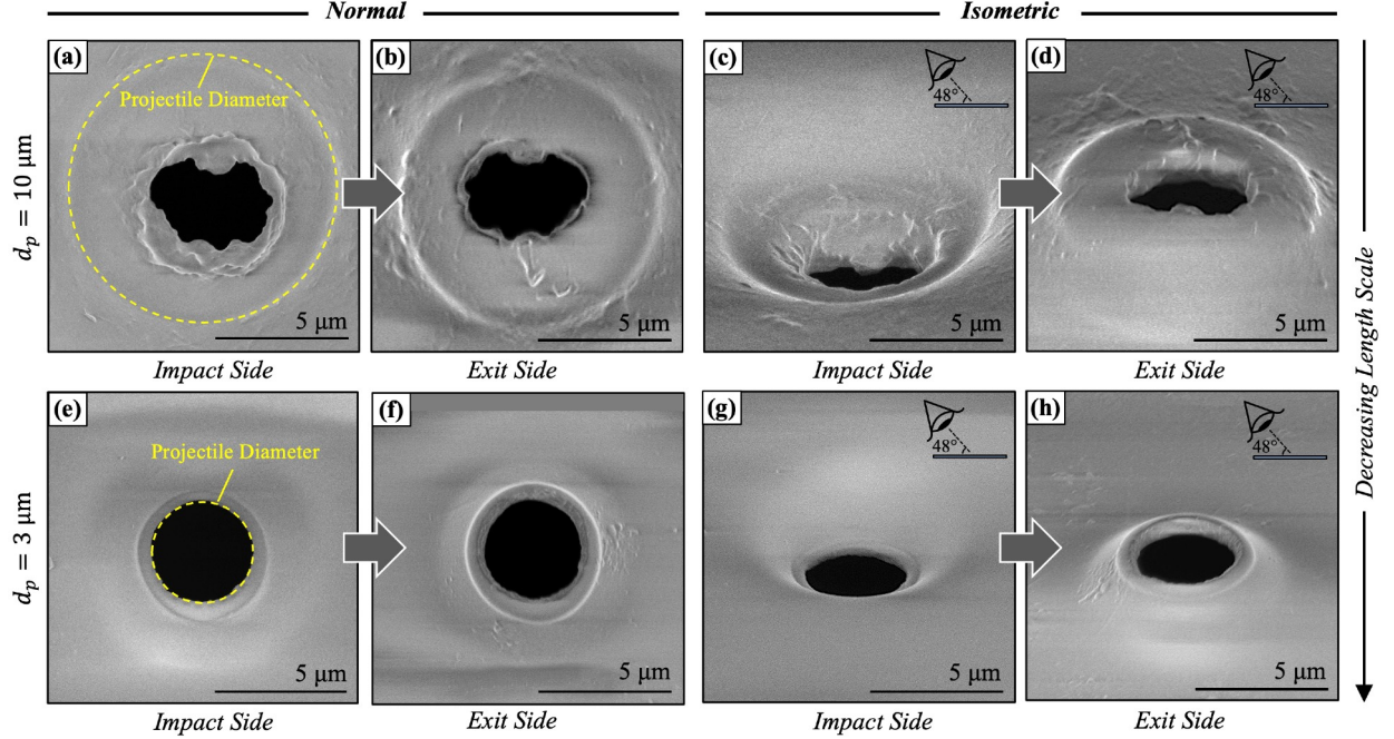
Figure S5: Orthogonal ( 90^\circ ) and isometric ( 48^\circ ) SEM images of the PC target perforations resulting from LIPIT impacts from alumina spheres with diameters of (a–d) d_p = 10\ \mu\text{m} and (e–h) d_p = 3\ \mu\text{m} . For each viewing perspective, an (a, c, e, g) impact side and exit side (b, d, f, h) image is shown. On each normal micrograph, a 2D projection of the projectile is overlaid, indicated by a dashed yellow line, to serve as a point of reference.
