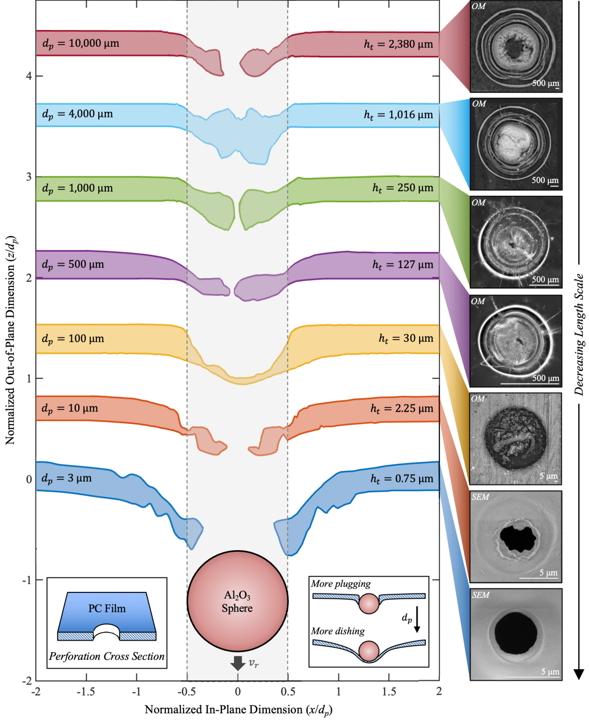
Figure 11: Representative experimental one-dimensional cross-sectional profiles of the perforated PC target samples (hatched region, figure inset). All profile data was captured using laser confocal microscopy and normalized by the respective projectile diameter ( d_p ) for comparison across length scales. At each scale, impact and exit side profiles (dark solid lines) are displaced by the corresponding h_t/d_p values provided in Table 1 for ease of visualization. An impact side micrograph of the target perforation is shown for each cross-sectional profile, with the microscopy technique noted in the top left corner: optical microscopy (OM) or scanning electron microscopy (SEM). Length scale decreases from top to bottom. Vertical dashed lines show the projectile diameter ( d_p/d_p = 1 ) relative to the perforation regions: normalized effective deformation area [ A_d/A_p ; Eq. (4)] grows with decreasing length scale.
