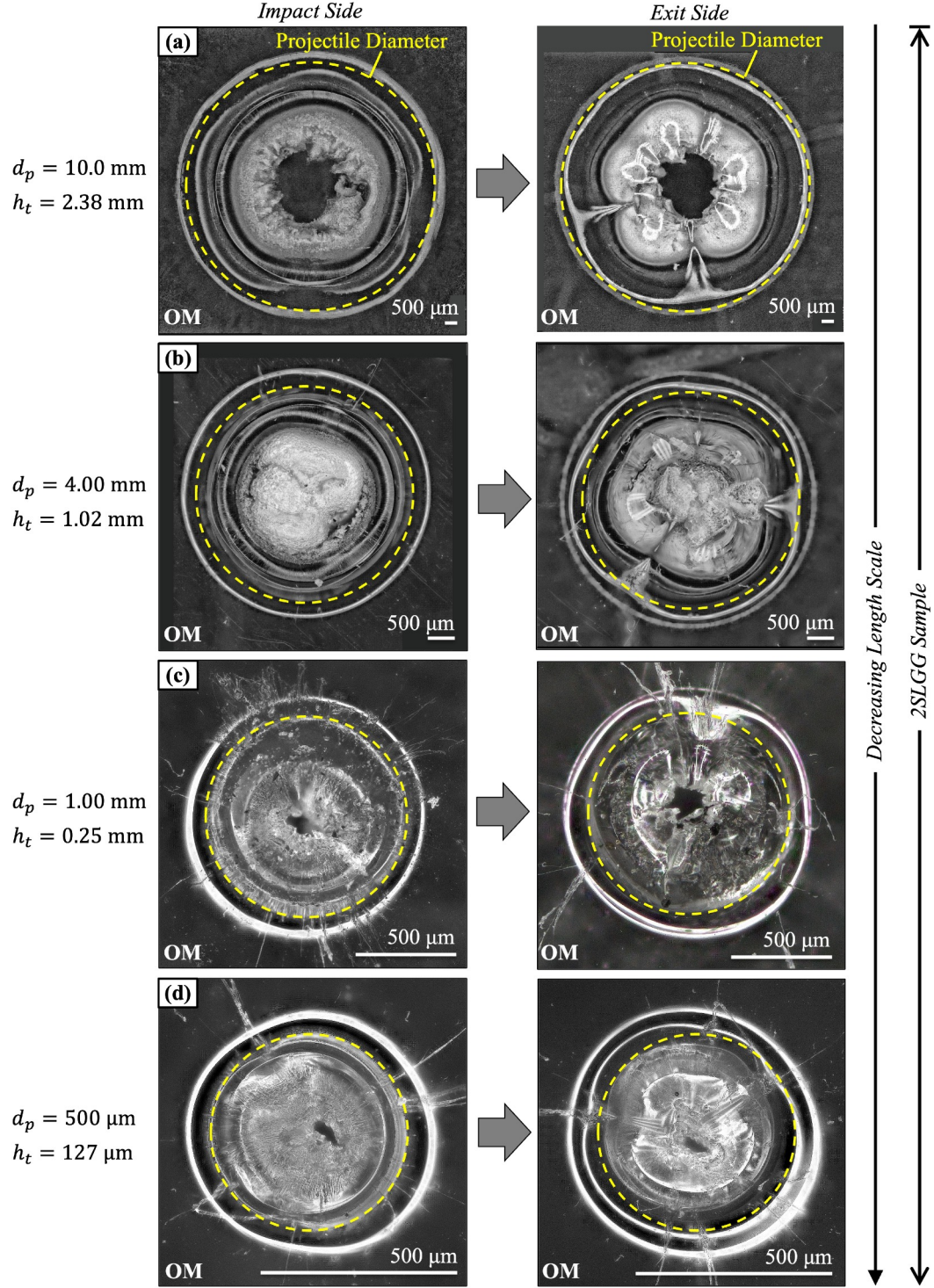
Figure 10: Microscopy images of perforated PC targets caused by impacts from alumina spheres with diameters of (a) d_p = 10 \text{ mm} , (b) d_p = 4 \text{ mm} , (c) d_p = 1 \text{ mm} , (d) d_p = 0.5 \text{ mm} , (e) d_p = 0.1 \text{ mm} , (f) d_p = 10 \mu\text{m} , and (g) d_p = 3 \mu\text{m} . The left column shows the impact face of the target, whereas the right column depicts the exit face. On each micrograph, a 2D projection of the projectile is overlaid for reference purposes. The microscopy technique is provided in the bottom left of each image.
