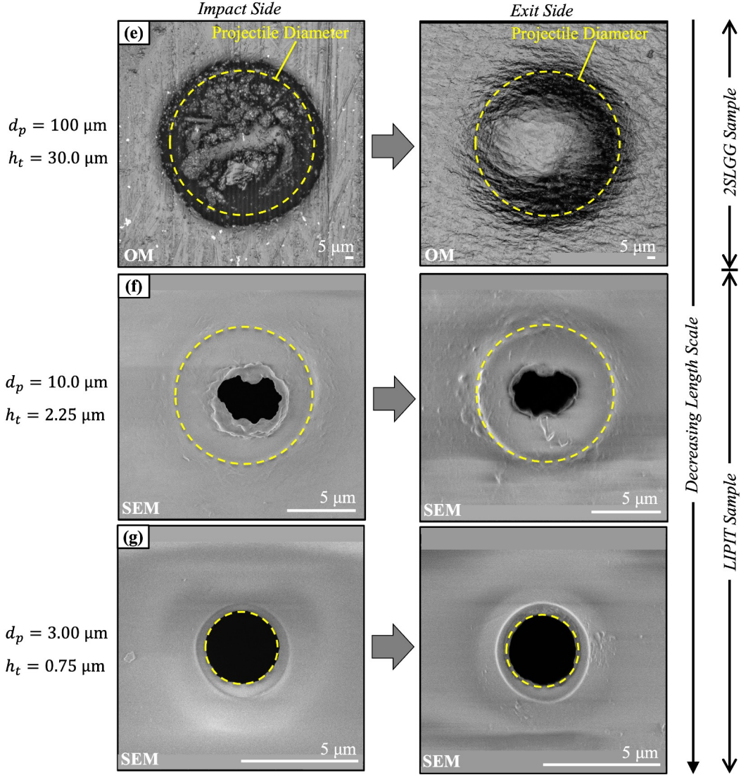
Figure 10 (Continued): Microscopy images of perforated PC targets caused by impacts from alumina spheres with diameters of (a) d_p = 10 mm, (b) d_p = 4 mm, (c) d_p = 1 mm, (d) d_p = 0.5 mm, (e) d_p = 0.1 mm, (f) d_p = 10 \mu\text{m} , and (g) d_p = 3 \mu\text{m} . The left column shows the impact face of the target, whereas the right column depicts the exit face. On each micrograph, a 2D projection of the projectile is overlaid for reference purposes. The microscopy technique is provided in the bottom left of each image.
