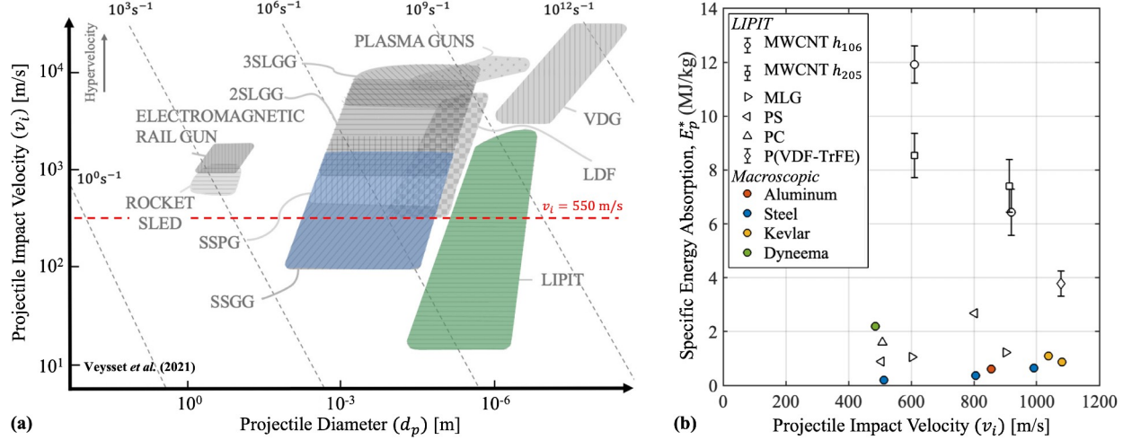
Figure 1: An overview of relevant launching techniques and experimental results from the literature: (a) representative launch capabilities as a function of impactor scale (adapted from [36]) and (b) specific energy absorption as a function of impact velocity for macro- and micro-scales (adapted from [40]). Apparatuses include the single-stage gas gun (SSGG), single-stage powder gun (SSPG), two-stage light gas gun (2SLGG), three-stage light gas gun (3SLGG), Van de Graaff accelerators (VDF), laser-driven flyer (LDF), laser-induced particle impact test (LIPIT), rocket sled, rail gun, and plasma gun. Materials impacted with similar h_t/d_p ratios include multi-walled carbon nanotubes (MWCNT) of thicknesses h_{106} and h_{205} nm, multi-layer graphene (MLG), polystyrene (PS), polycarbonate (PC), poly(vinylidene fluoride-co-trifluoroethylene) P(VDF-TrFE), as well as macroscopic target aluminum, steel, Kevlar, and Dyneema.
