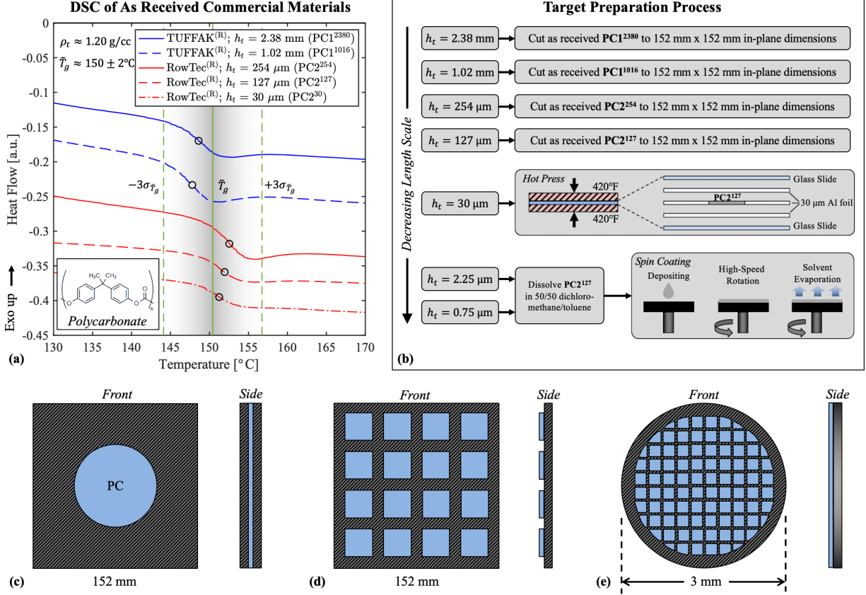
Figure 3: An overview of the polycarbonate (PC) targets: (a) a representative differential scanning calorimetry curve for each as-received target material and (b) the target preparation process for each film thickness, h_t . Two materials were used in target preparation: Plaskolite, LLC. TUFFAK ® (PC1; h_t = 1.02, 2.38 mm) and Rowland Advanced Polymer Films RowTec ® (PC2; h_t = 0.75, 2.25, 30, 127, 250 \mu\text{m} ). All material had similar densities ( \rho_t ) and glass transition temperature ( T_g ) values. Targets were fixed (c) between apertured plates ( h_t = 127, 254, 1,016, 2,380 \mu\text{m} ), (d) in an array on a custom grid ( h_t = 30 \mu\text{m} ), or (e) on a 200 mesh TEM grid ( h_t = 0.75, 2.25 \mu\text{m} ).
