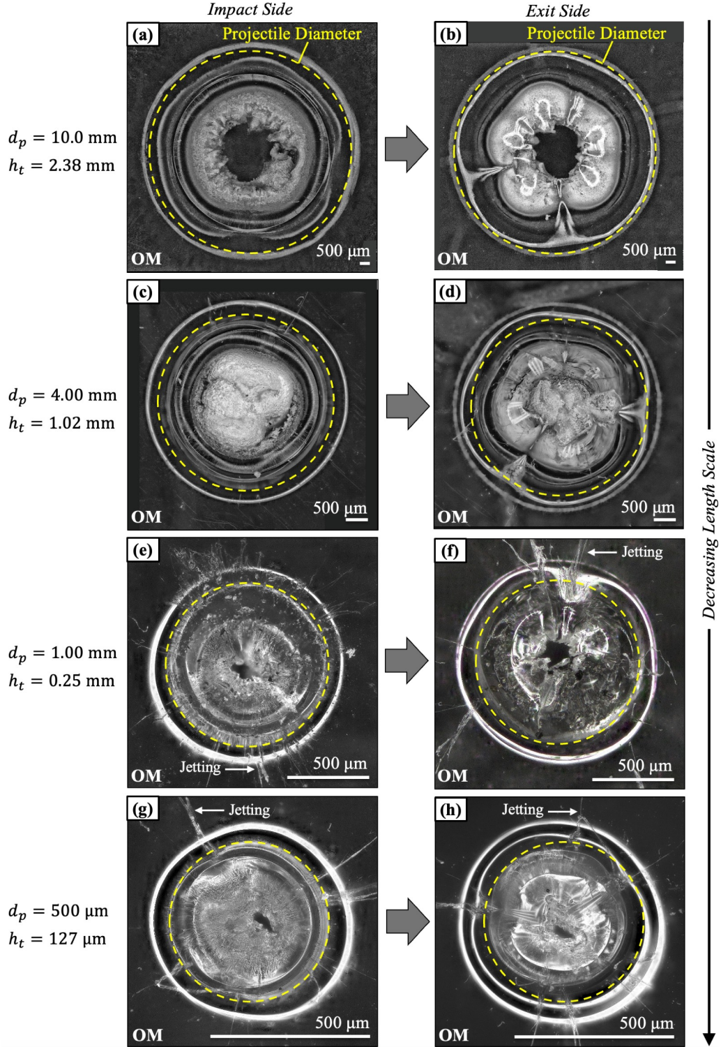
Figure 10: Orthogonal micrographs (along impact axis) display perforations in the PC targets caused by impacts from alumina spheres with diameters of (a, b) d_p = 10 \text{ mm} , (c, d) d_p = 4 \text{ mm} , (e, f) d_p = 1 \text{ mm} , and (g, h) d_p = 0.5 \text{ mm} . Within the array of images, the left column (a, c, e, g) represents the impact face of the target, whereas the right column (b, d, f, h) depicts the exit face. On each micrograph, a 2D projection of the projectile is overlaid, indicated by a dashed yellow line, to serve as a point of reference. The microscopy technique is provided in the bottom left of each image.
