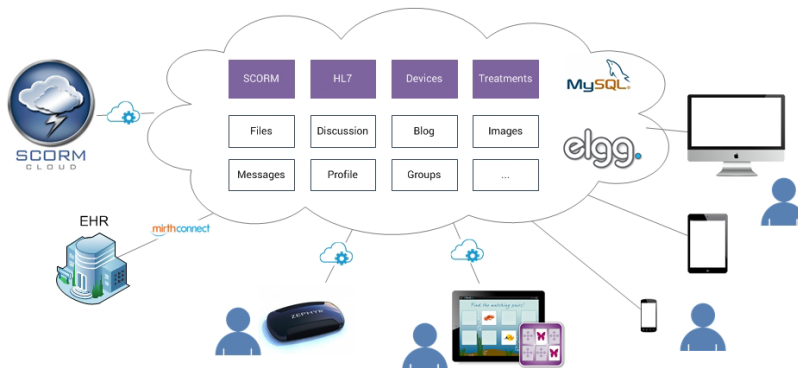
Figure 1. uHSN platform architecture.
