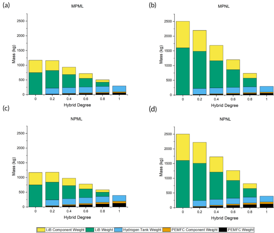
Figure 7: Power system mass distributions for a heavy-goods FCHEV and FCEV scenario under different cell operating powers. (a) MPML (b) MPNL (c) NPML (d) NPNL
