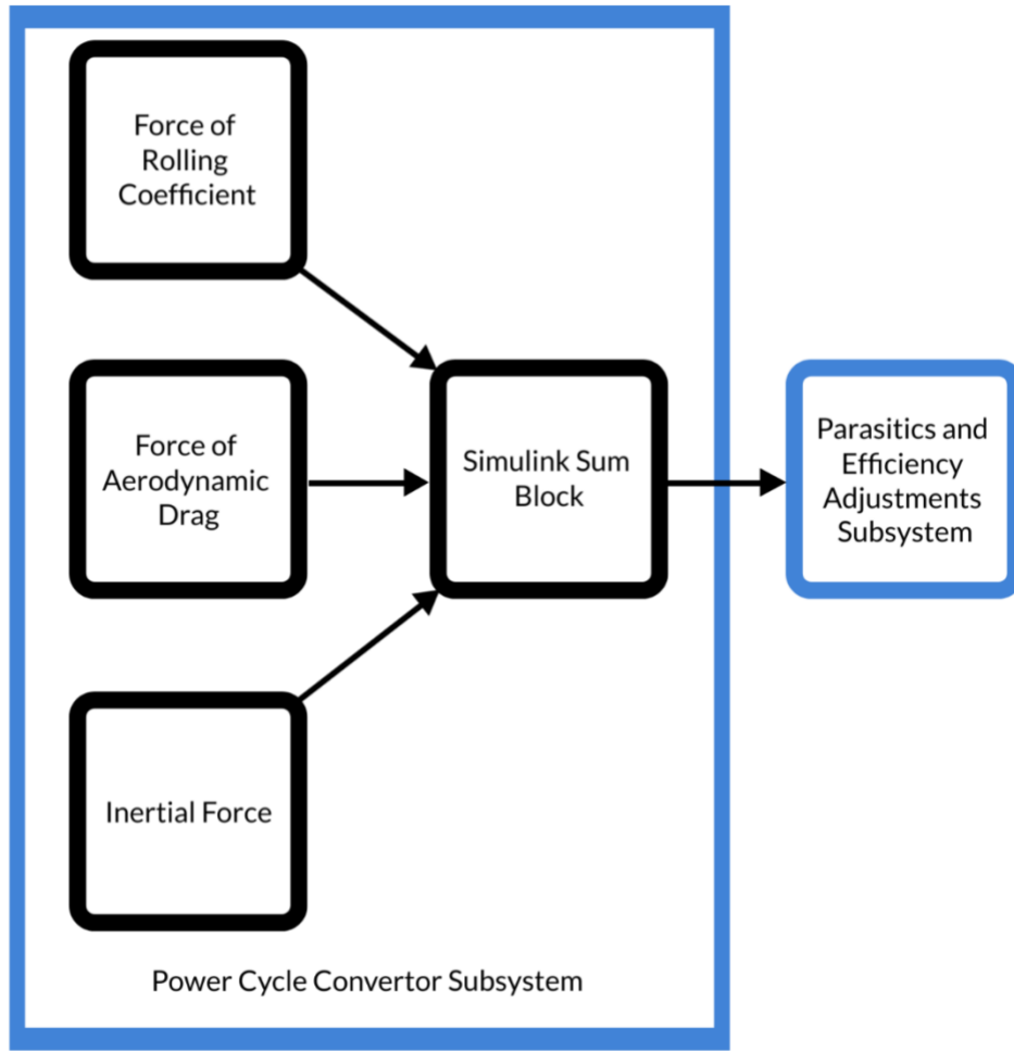
Figure 3: Model overview of power cycle convertor subsystem. This subsystem converts a drive cycle to a power cycle to determine the maximum required power of the proposed vehicle.
