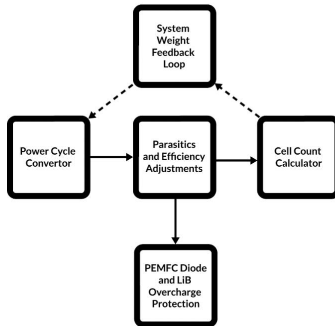
Figure 1: HybeMass model, general overview of subsystems.
