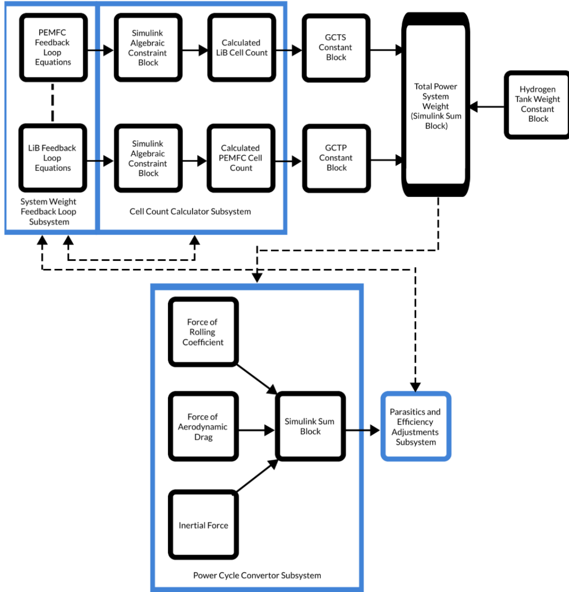
Figure 4: Detailed block layout of system mass feedback loop subsystem.
