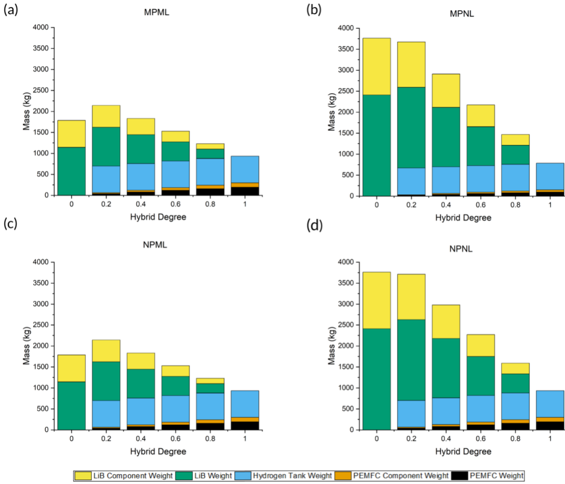
Figure 6: Power system mass distributions for a heavy-goods FCHEV and FCEV scenario under different cell operating powers. (a) MPML (b) MPNL (c) NPML (d) NPNL
