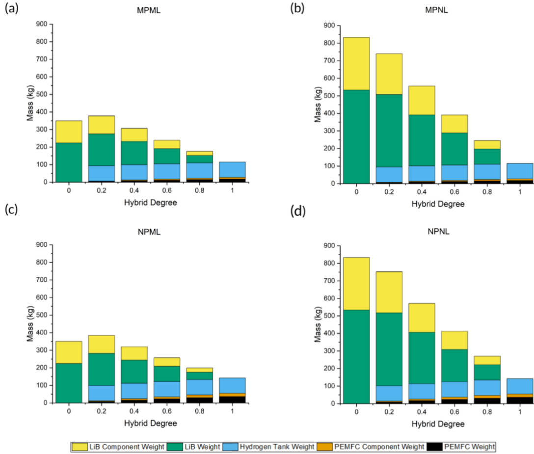
Figure 5: Power system mass distributions for a LDV FCHEV and FCEV scenario under different cell operating powers. (a) MPML (b) MPNL (c) NPML (d) NPNL
