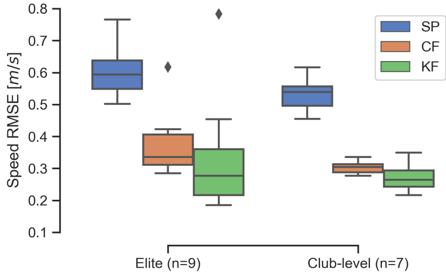
Fig 14. Summary of the speed estimate error for all trials. Comparisons of the distributions of RMSE_v of the speed estimates from the three methods for each full length trial.
