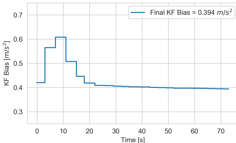
Fig 8. Convergence of the Kalman filter bias state over a single trial (elite 16NW). The filter bias state typically takes about 20 seconds to converge to a relatively constant value.
