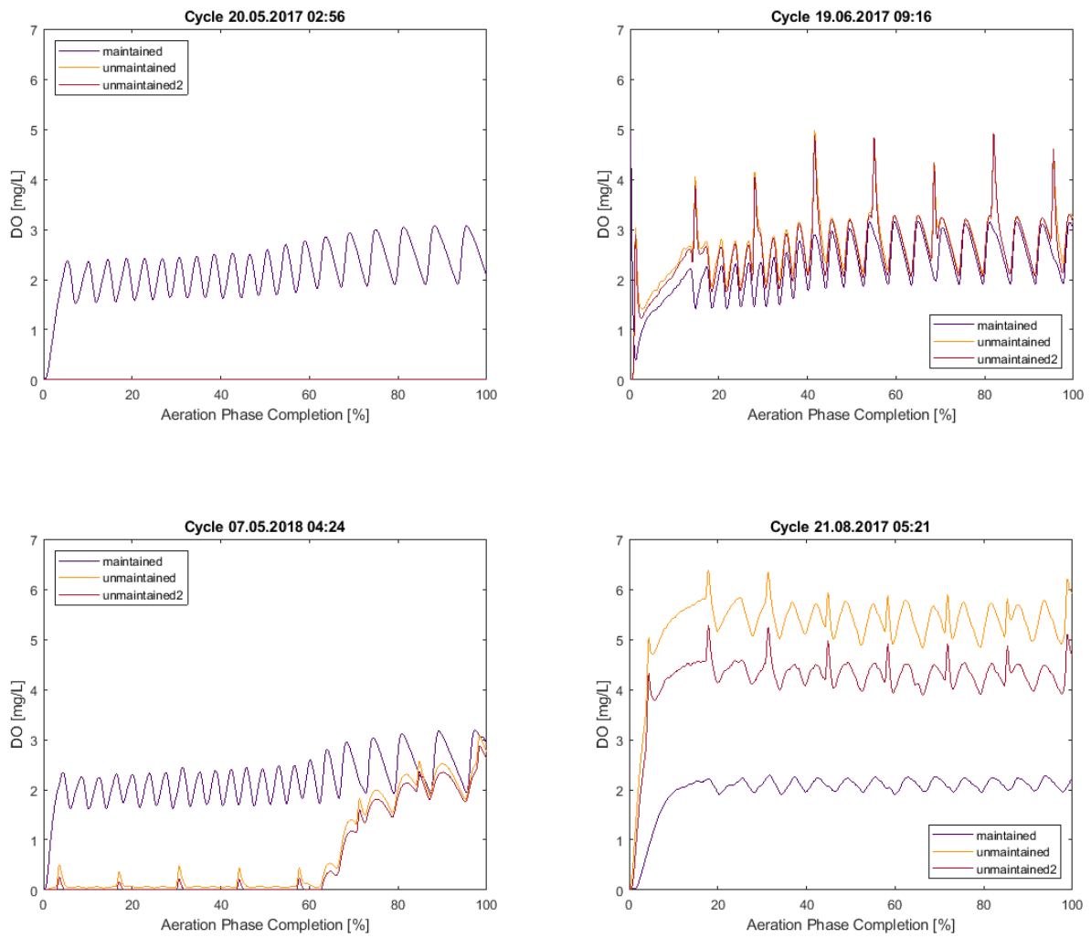
Figure A.3: Behaviour of the unmaintained DO signals represented by four cycles during the experimental period which showed non-linear deterioration effects
