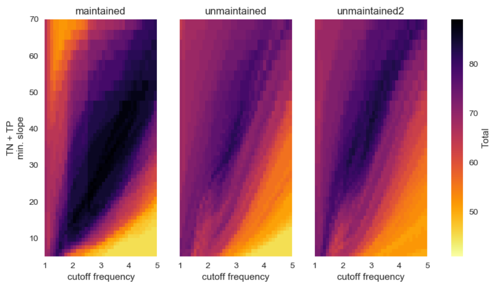
Figure 5: The total of all true predictions for the DO soft sensor's parameters, which are minimal slope and cut-off frequency. The maintained sensor is compared to the unmaintained sensor.
