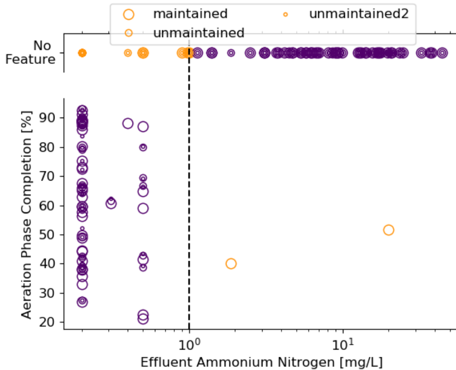
Figure 7: Aeration ramp (DO soft sensor) – Measured effluent ammonium nitrogen concentration against the feature detection time during the aeration phase. The feature is a steep slope in the DO signal. The upper plot shows the concentrations for cycles in which no feature was detected. The presence of the feature should correspond to a concentration below the threshold, here shown with a vertical line (1 mg/L). The analysis from the maintained sensor is shown by a large circle, the unmaintained sensors by smaller circles with decreasing diameters. The colours of the markers indicate whether the classification was true (purple/darker) or false (orange/lighter).
