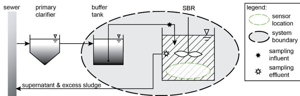
Figure 1: Schematic representation of the pilot-scale SBR setup. Sensor location is the level where the sensors are installed in the SBR. The system boundaries indicate which
