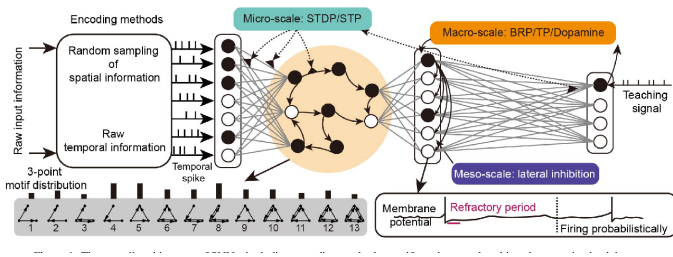
Fig. 3. The SNNs motif topology, multi-scale synaptic plasticity, etc [16]
