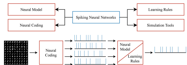
Fig. 1. Spiking Neural Networks (SNN) [14]
