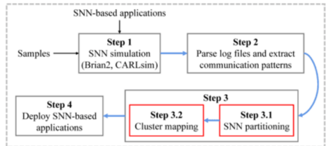
Fig. 4. SNN based Software working process [17]
