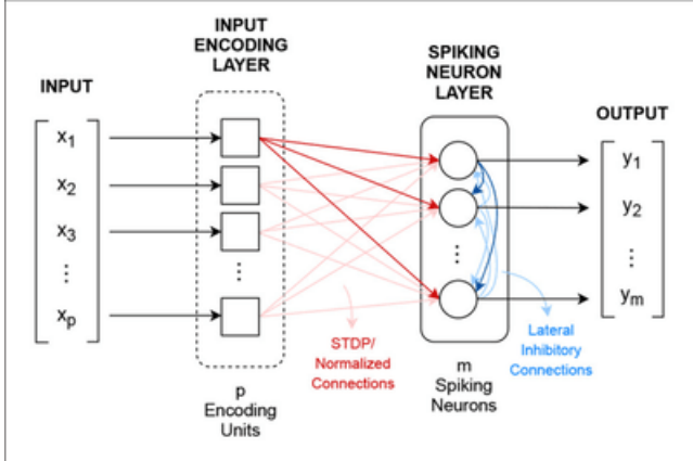
Fig. 2. Spiking neurons [15]
