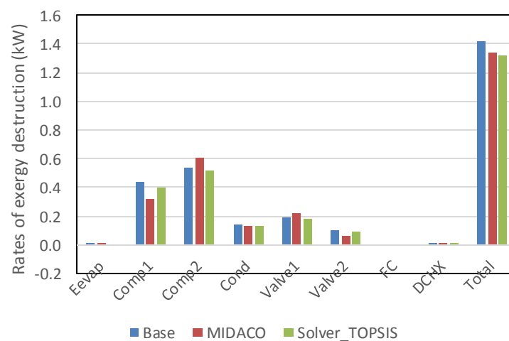
Figure 15. Comparison of the rates of exergy destruction in the system
