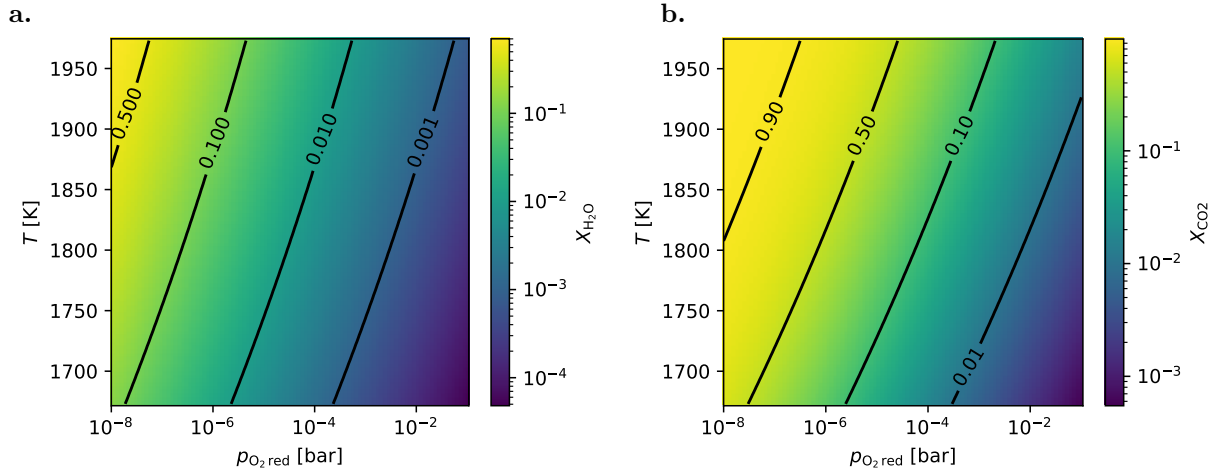
Figure 4: The feedstock conversion limits of an isothermal cycle plotted against the reduction partial pressure and the reduction temperature for a. \text{H}_2\text{O} thermolysis and b. \text{CO}_2 thermolysis.
