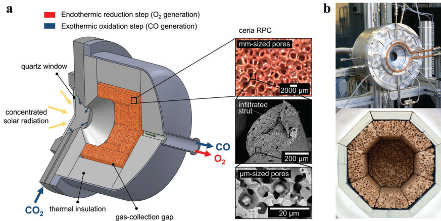
Figure 2: A schematic of the directly irradiated cavity reactor tested by Marxer et al. , copied from [34]. This type of reactor design has proven very popular for its relative simplicity with the same general design used in many other demonstrations [10, 11, 12, 22, 28].
