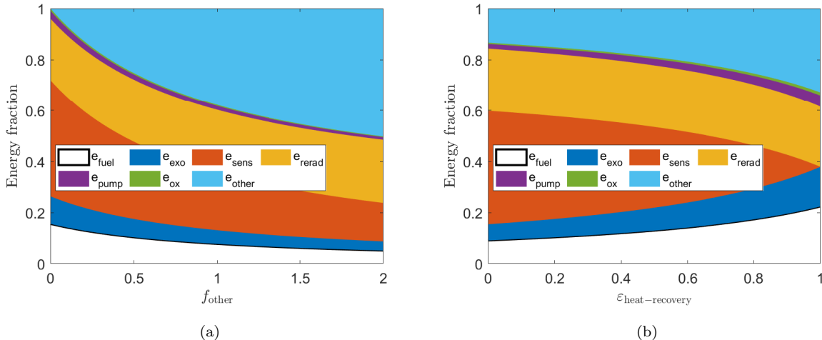
Figure 8: Reactor efficiency \eta and energy breakdown for a vacuum operated reactor as a function of (a) f_{\text{other}} , and (b) \epsilon_{\text{HR}} . The analysis performed for the baseline cycle (Table 3).
