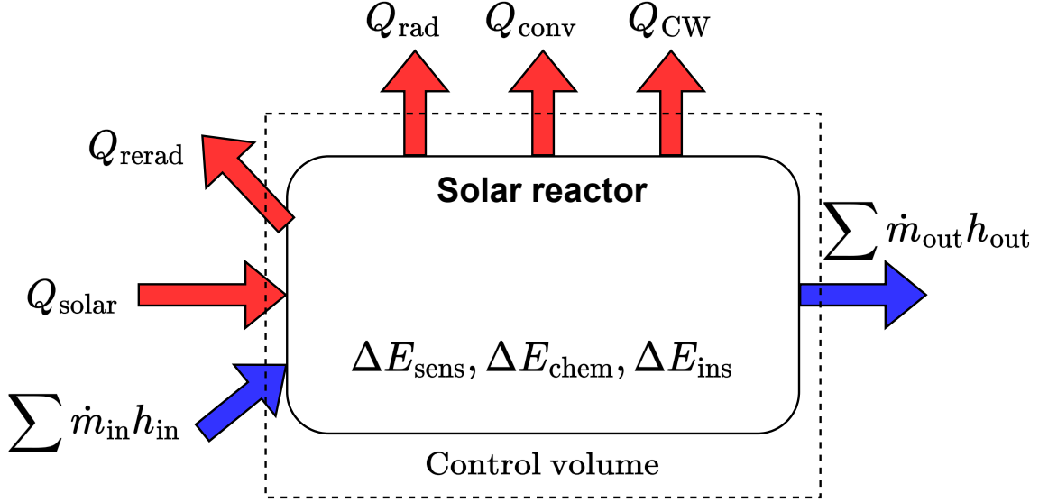
Figure 5: Control volume of the solar reactor including all the energy terms.
