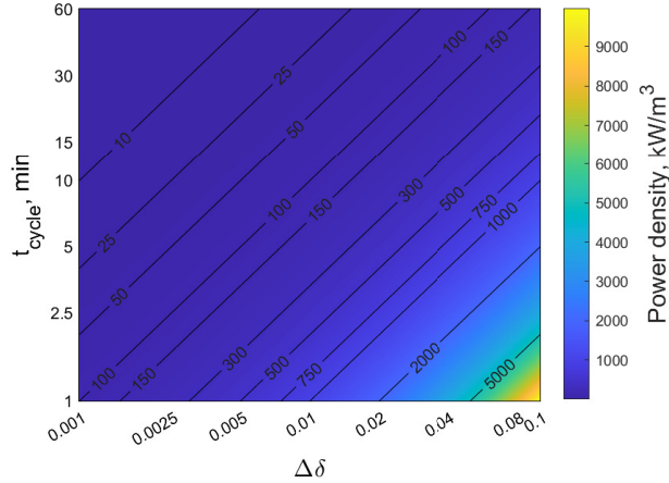
Figure 13: Power density as a function of \Delta\delta and t_{\text{cycle}} for \text{CeO}_2 with \varepsilon_{\text{void}} = 0.5 .
