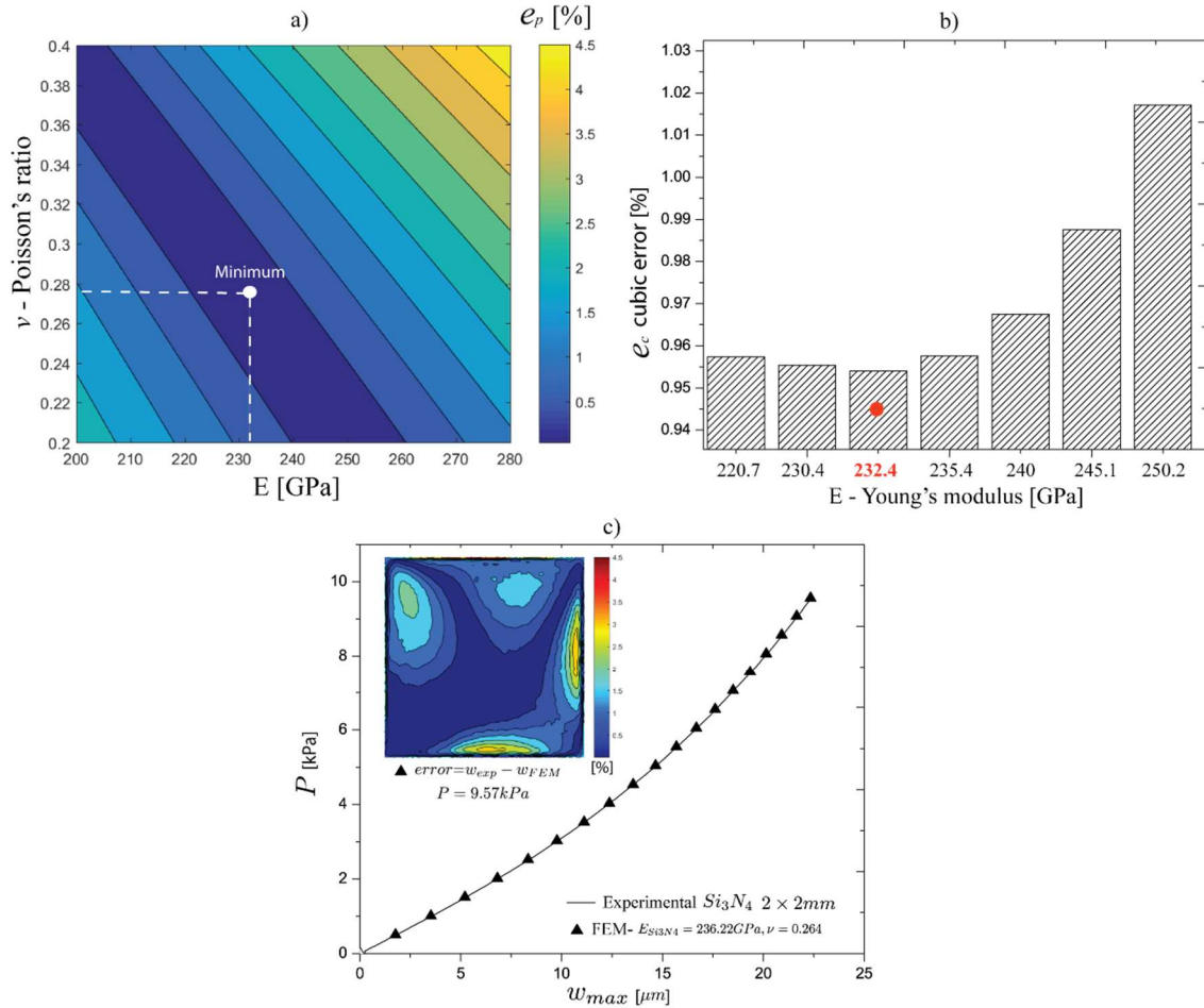
Figure 3: a. e_p(E, \nu) error function. b. RMS cubic error scheme of the experimental setup. c. Load-deflection curve comparisons.
