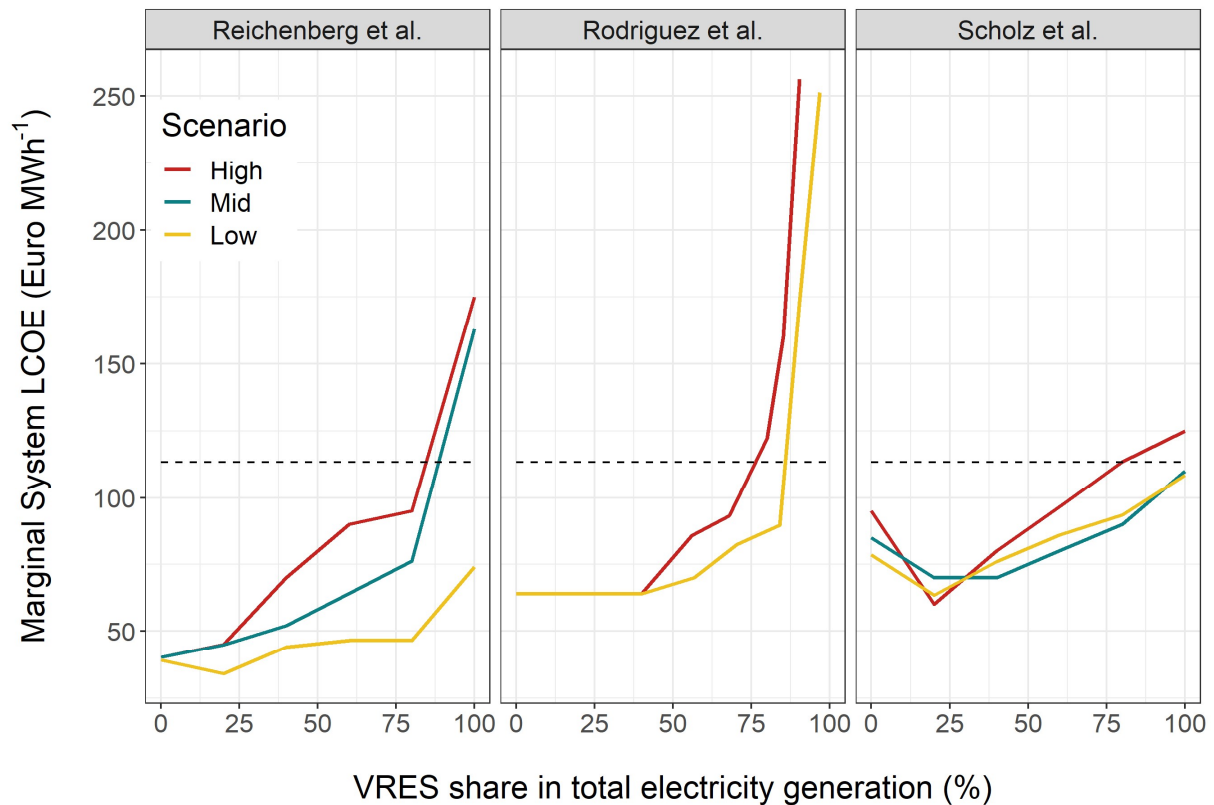
Figure 3: Marginal system levelized costs of electricity (LCOE) for varying levels of VRES in total generation for different scenarios in three different modelling studies 39–41 (coloured lines) compared to lower bound for costs of generating electricity from WWS diesel 16 (black dashed line). Scenarios are derived for the period 2035–2050. Marginal System LCOE are calculated according to Reichenberg et al. 41 . See appendix for details.
