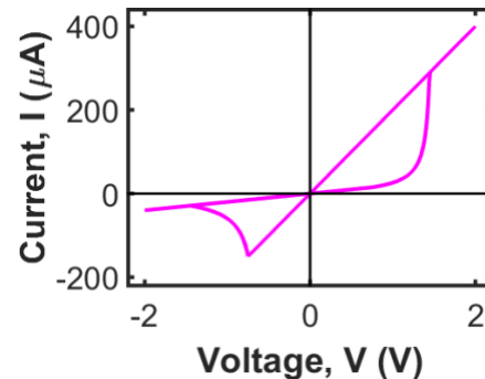
Figure 2: I-V characteristics of memristor model.
