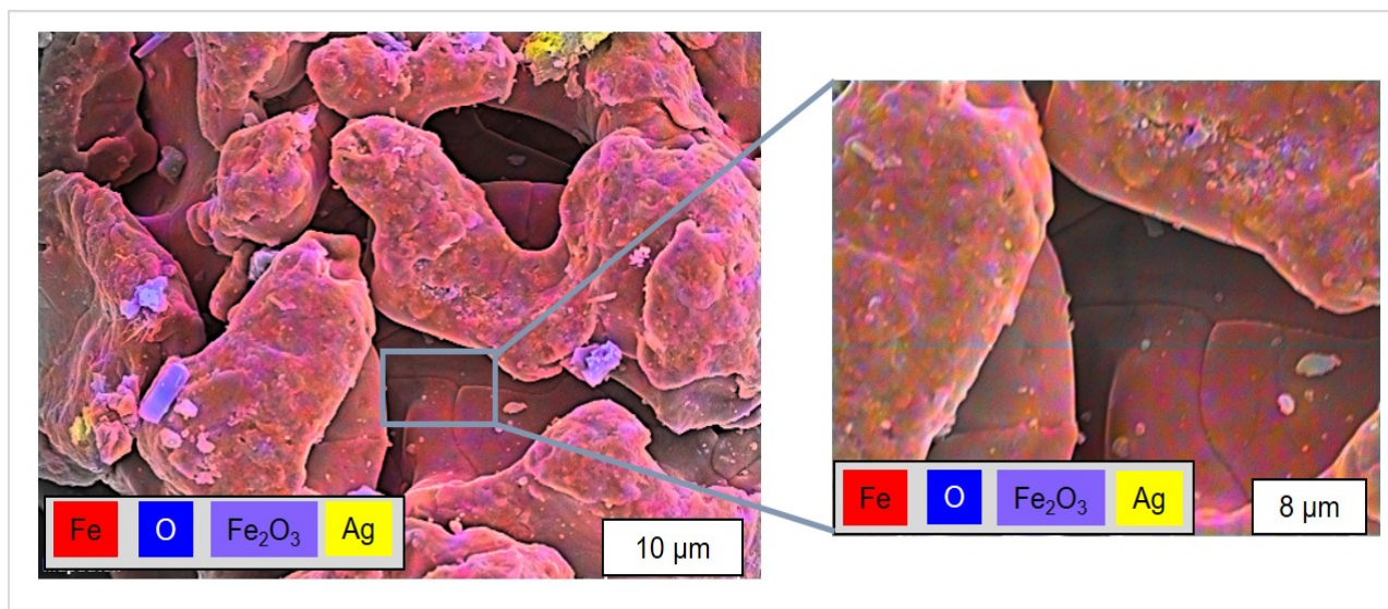
Fig. S-6: Elemental map data of a reduced bio-hematite after 20 h of electrolysis at -1.4 V vs. Ag/AgCl in 10 M NaOH at 363 K shows areas where Fe is inclusively present. Note that silver appears as a binder during pelletizing and that the presence of oxygen stains from the ambient atmosphere in the SEM chamber is unavoidable.
