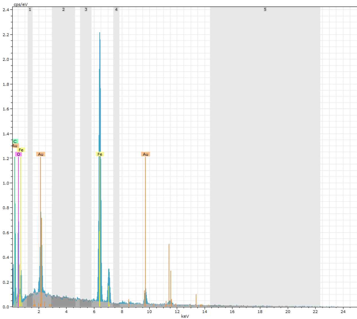
Fig. S-7: EDX analysis reveals traces of carbon in the bio-magnetite, probably from dead microorganisms or the partial formation of siderite ( \text{FeCO}_3 ).
