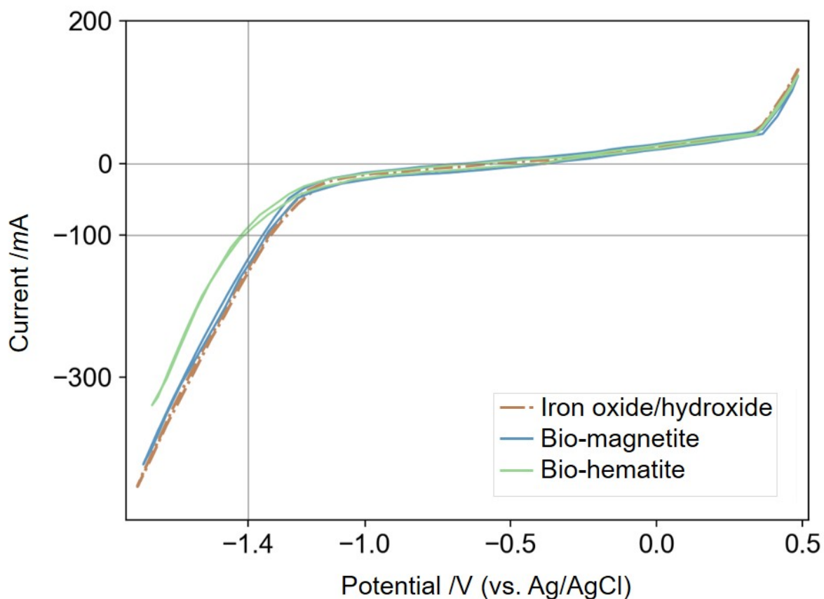
Fig. S-4: The first cycle of cyclic voltammetry test in 10 M NaOH for iron oxide/hydroxide as starting material, the biologically produced magnetite (bio-magnetite), and after heat treatment (bio-hematite) at 363 K and the obtained iron yields. No redox peaks appear as the materials are not yet electrochemically activated.
