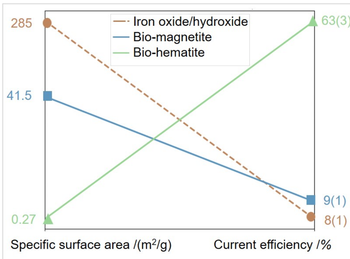
Fig. S-5: Visualization of the inverse relationship between specific surface area (logarithmic scale) and current efficiencies for iron oxide/hydroxide as starting material, the biologically produced magnetite, and after heat treatment (bio-hematite) after conducting 20 h chronoamperometry at -1.4 V vs. Ag/AgCl in 10 M NaOH at 363 K. The numbers in brackets are the estimated standard deviations of the obtained values in the last digit.
