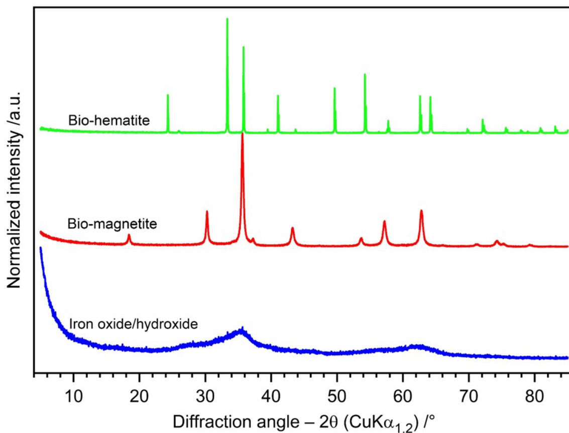
Fig. S-2: X-ray powder data Rietveld (XRPD) plots of iron oxide/hydroxide as the starting material, the biologically produced magnetite (bio-magnetite), and that after calcining (bio-hematite). XRPD data confirms that bio-mining has successfully converted a quantum-crystalline ferrihydrite with an average crystallite size (ACS) of 2.7(1) nm into a micro-crystalline bio-magnetite (ACS = 16.2(2) nm). Heat treatment increased the ACS further to 238(6) nm for bio-hematite.
