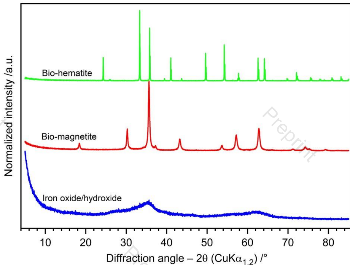
Figure S2. X-ray powder data Rietveld (XRPD) plots of iron oxide/hydroxide as the starting material, the biologically produced magnetite (bio-magnetite), and that after calcining (bio-hematite). XRPD data confirms that bio-mining has successfully converted a quantum-crystalline ferrihydrite with an average crystallite size (ACS) of 2.7(1) nm into a micro-crystalline bio-magnetite (ACS = 16.2(2) nm). Heat treatment increased the ACS further to 238(6) nm for bio-hematite.
