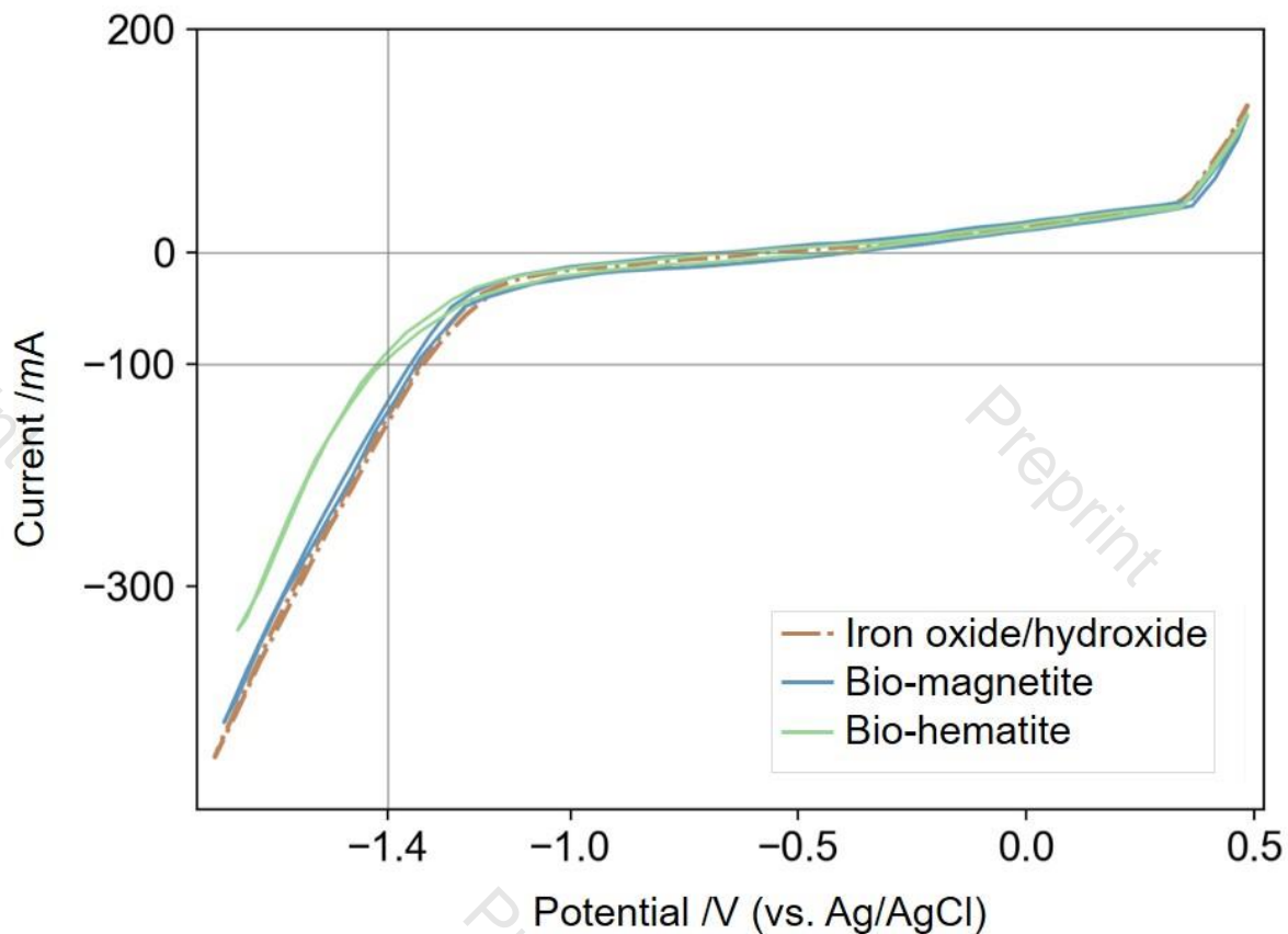
Figure S4. The first cycle of cyclic voltammetry test in 10 M NaOH for iron oxide/hydroxide as starting material, the biologically produced magnetite (bio-magnetite), and after heat treatment (bio-hematite) at 363 K and the obtained iron yields. No redox peaks appear as the materials are not yet electrochemically activated.
