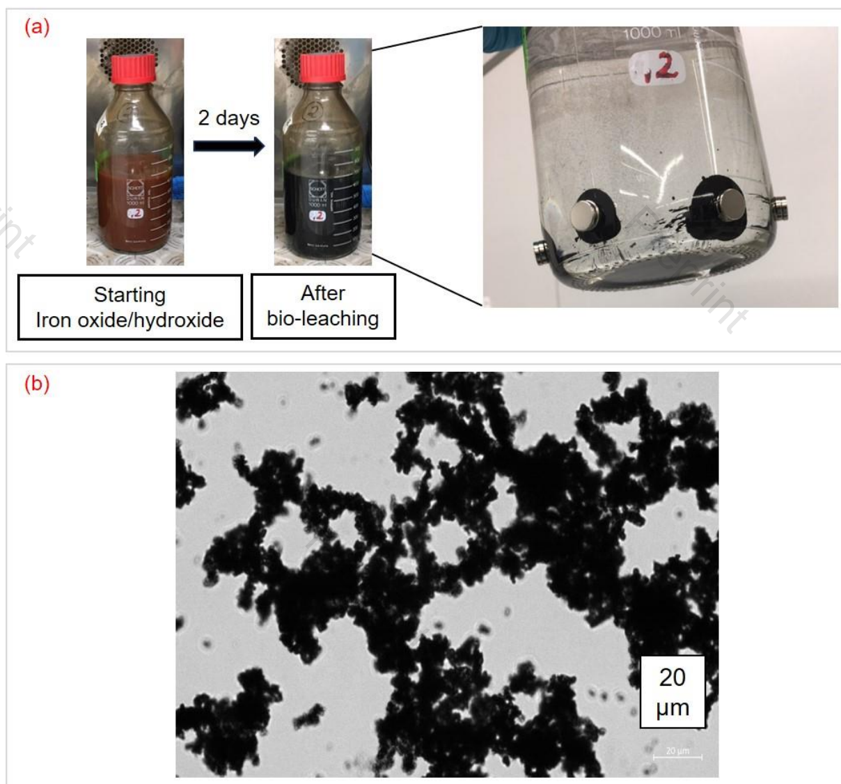
Figure S1. The iron-reducing bacterium was C. ferrireducens as a terminal electron acceptor for anaerobic respiration. (a) A full magnetic response was observed after two days of iron oxide/hydroxide bio-mining. (b) Black magnetic particles from C. ferrireducens cultures (2 days) were observed with transmitted white light, revealing the presence of microbial cells all over the particles.
