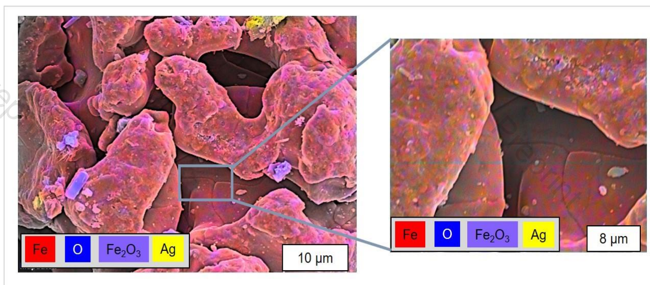
Figure S6. Elemental map data of a reduced bio-hematite after 20 h of electrolysis at -1.4 V vs. Ag/AgCl in 10 M NaOH at 363 K shows areas where Fe is inclusively present. Note that silver appears as a binder during pelletizing and that the presence of oxygen stains from the ambient atmosphere in the SEM chamber is unavoidable.
