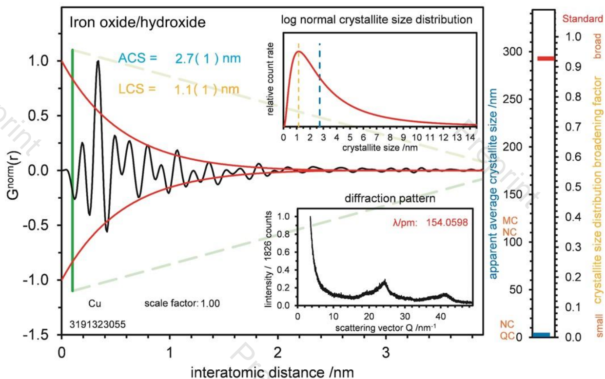
Figure S3. The PDF EnvACS method to determine the ACS of iron oxide/hydroxide.
