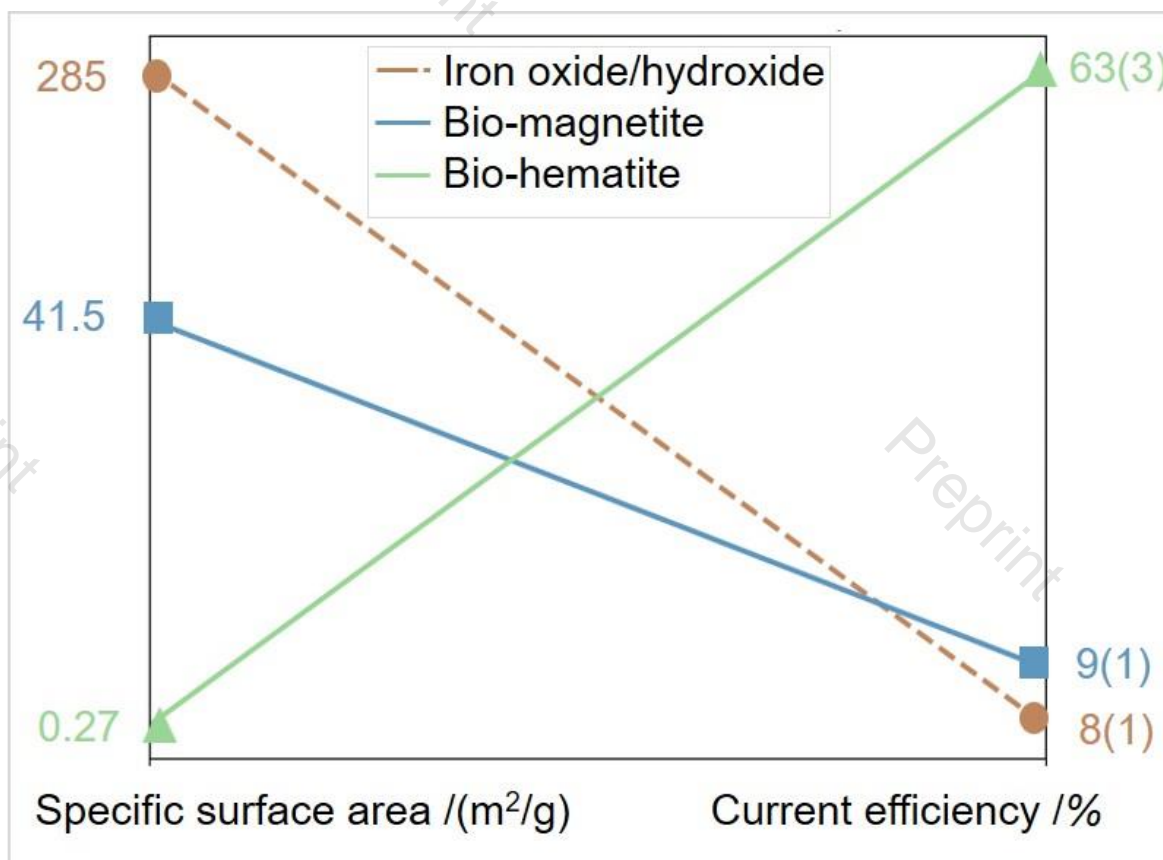
Figure S5. Visualization of the inverse relationship between specific surface area (logarithmic scale) and current efficiencies for iron oxide/hydroxide as starting material, the biologically produced magnetite, and after heat treatment (bio-hematite) after conducting 20 h chronoamperometry at -1.4 V vs. Ag/AgCl in 10 M NaOH at 363 K. The numbers in brackets are the estimated standard deviations of the obtained values in the last digit.
