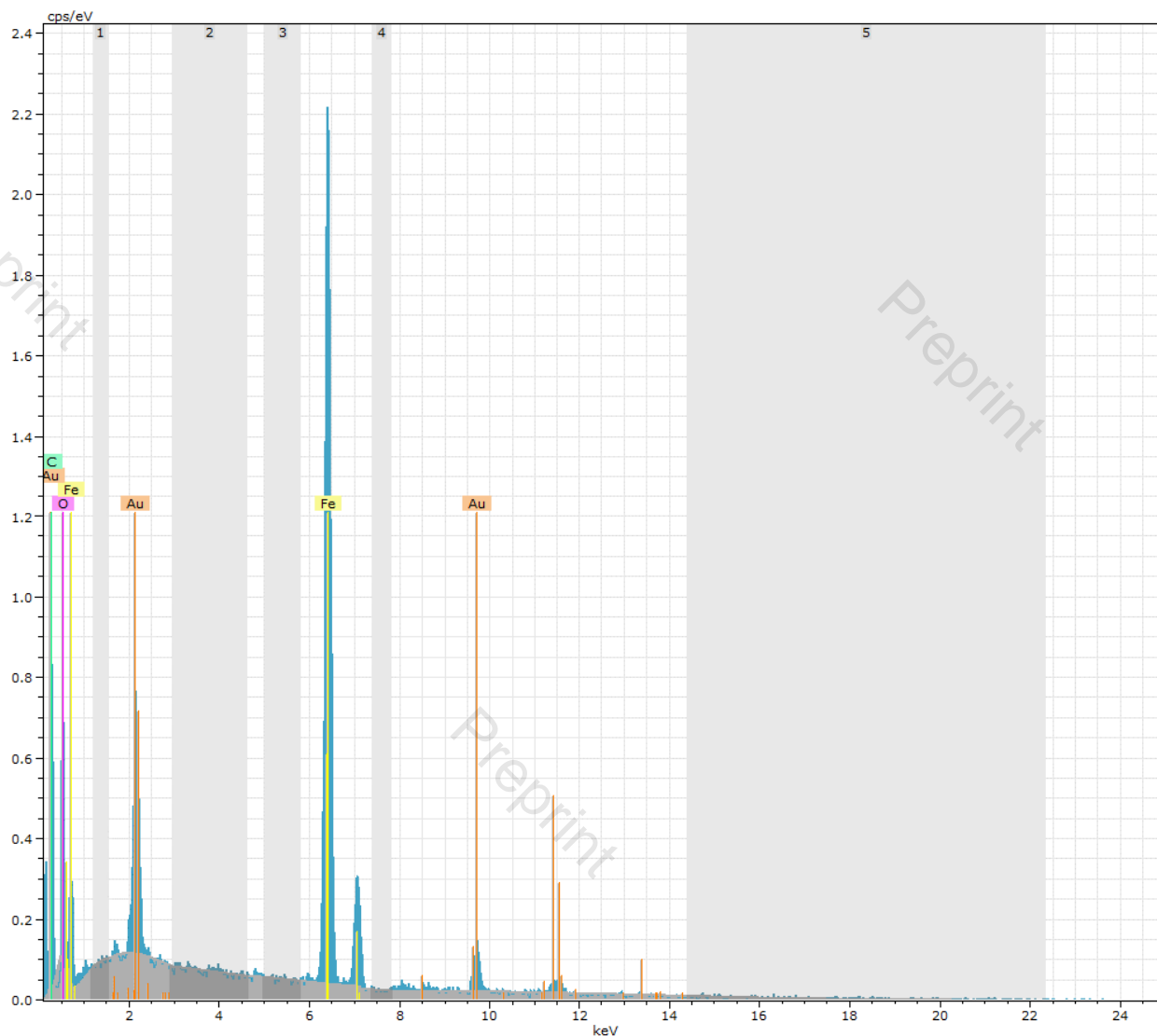
Figure S7. EDX analysis reveals traces of carbon in the bio-magnetite, probably from dead microorganisms or the partial formation of siderite ( \text{FeCO}_3 ).
