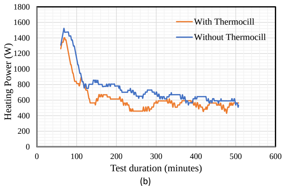
Figure 5: The variation of (a) heating power and (b) 60 minutes average heating power in terms of time for the case of with Thermocill compared with no Thermocill case
