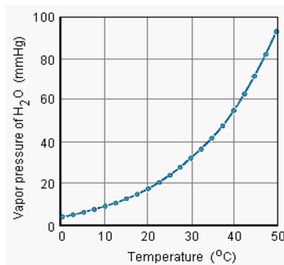
Figure 1: Vapour pressure in terms of temperature for water (taken from [2])
