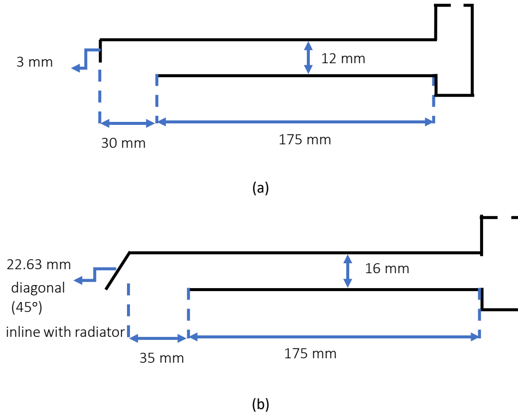
Figure 4: The schematic of the (a) original Thermocill design and (b) optimised Thermocill design, along with based dimensions.
