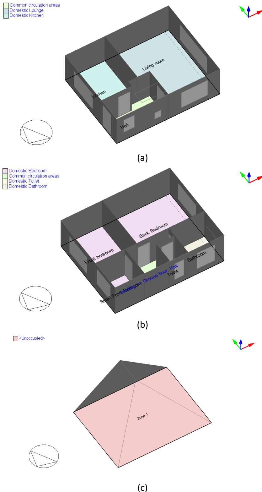
Figure 7: The sketch of different floor plans (a) ground floor, (b) first floor, (c) roof space
