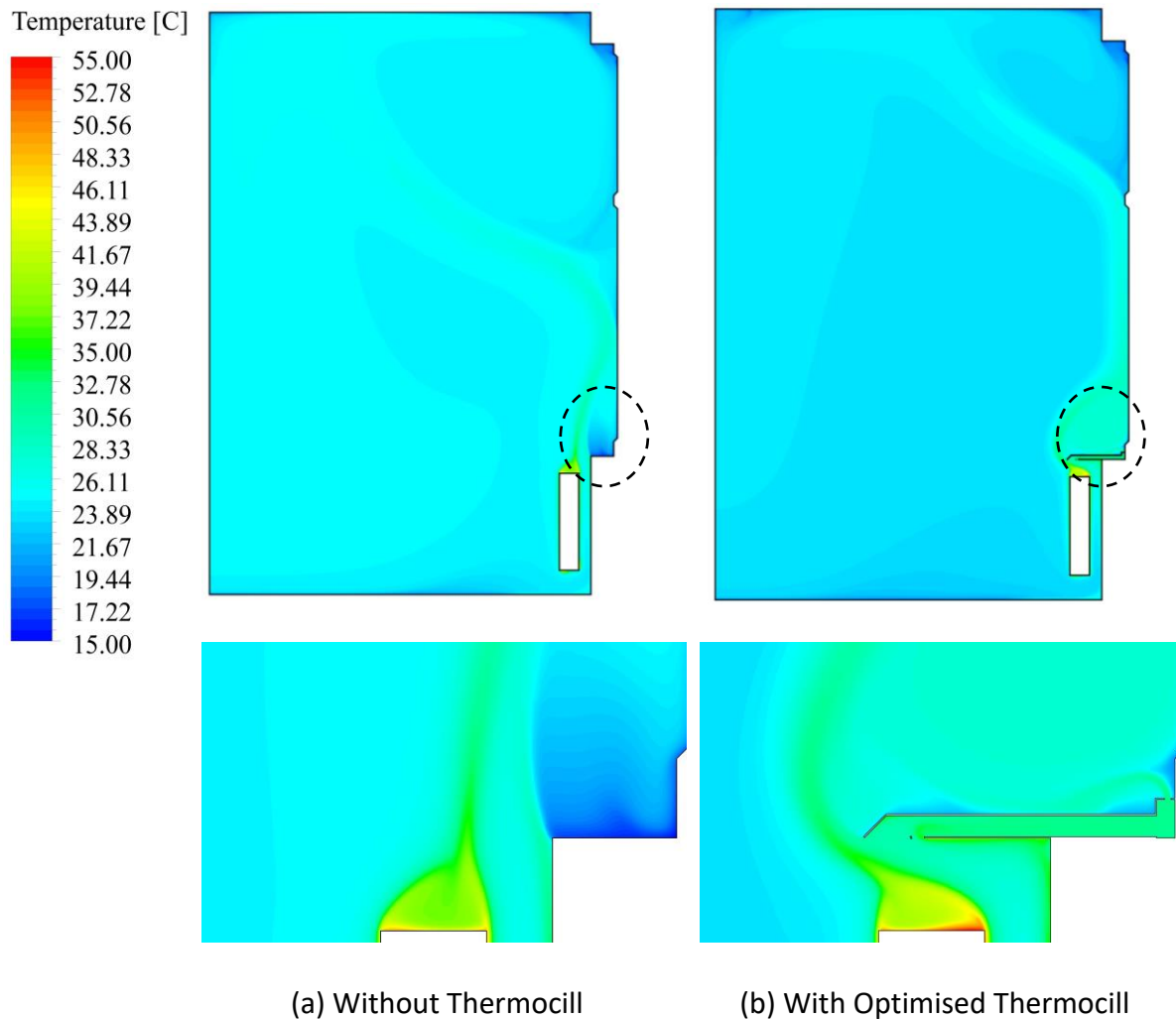
Figure 3: The contour plots of temperature distribution for the cases of (a) No Thermocill and (b) With optimised Thermocill, obtained by CFD.
