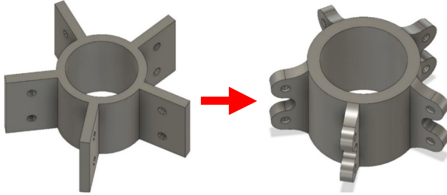
Figure 5: “POLO-1” Splice Node Connection before and after design modifications.
