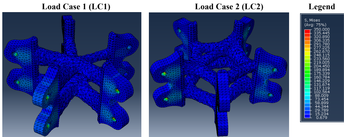
Figure 7: Optimised design against LC1.
