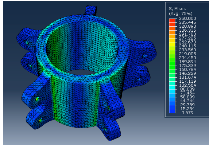
Figure 12: FEA Structural testing of the traditional node-connection against Load Case 1.
