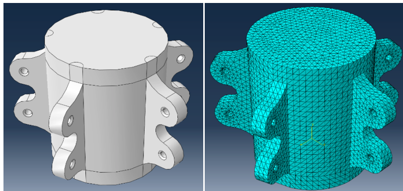
Figure 6: Meshing of “Connection A” for the optimisation.
