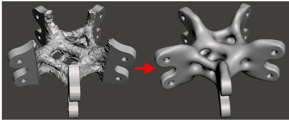
Figure 15: An optimised node connection before and after post-processing.
