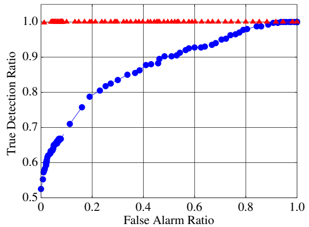
Figure 10. Receiver Operating Characteristics (ROC) curve. ● represents the linear index and ▲ represents the nonlinear index.
