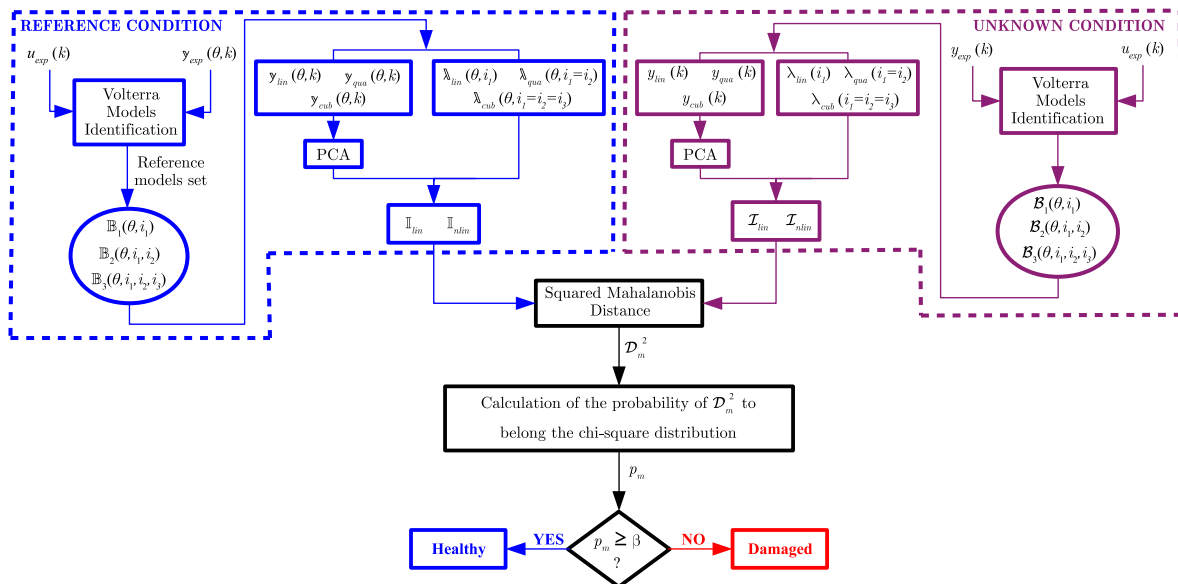
Figure 1. Flowchart of the damage detection methodology proposed.
