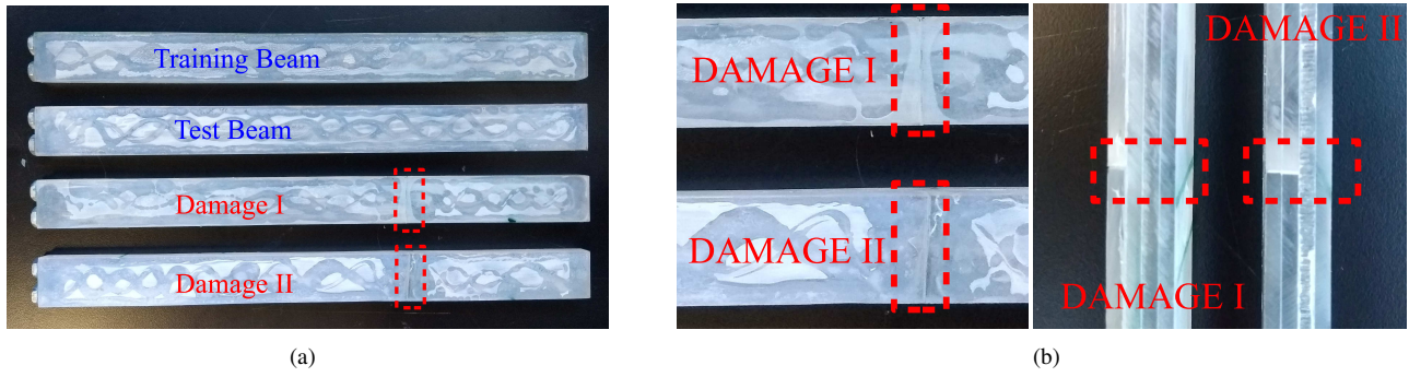
Figure 4. Structural conditions considered; (a) all beams constructed and (b) damaged beams (zoom).
