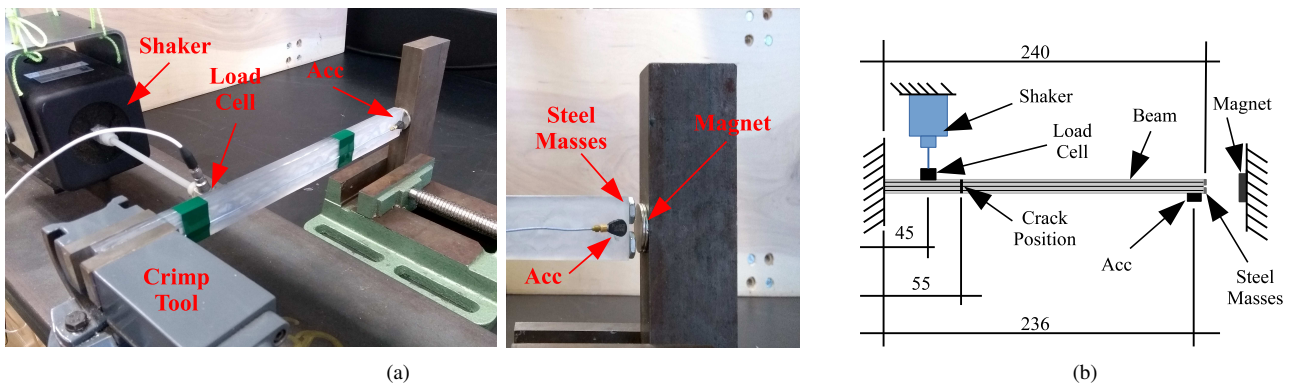
Figure 2. Experimental apparatus; (a) photos and (b) scheme (dimensions in [mm]).
