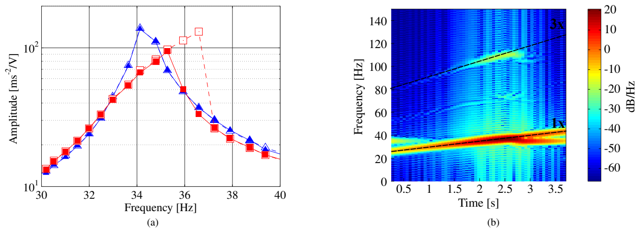
Figure 3. Intrinsic nonlinear behavior of the system. (a) Stepped sine test, where -\triangle- , -\blacktriangle- , -\square- and -\blacksquare- represent, respectively, frequency up and frequency down considering low level of input, and frequency up and frequency down considering high level of input. (b) Time-frequency diagram of the system response.
