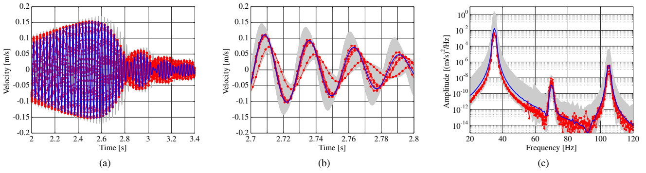
Figure 7. Verification and validation of the reference model. (a) Model response in the time domain considering a chirp excitation. (b) Model response in the time domain considering a chirp excitation (zoom). (c) Model response in the frequency domain considering a sine excitation. ■ represents the 99% model response confidence bands, — represents the model response mean and -●- represents five realizations of the experimental data.
