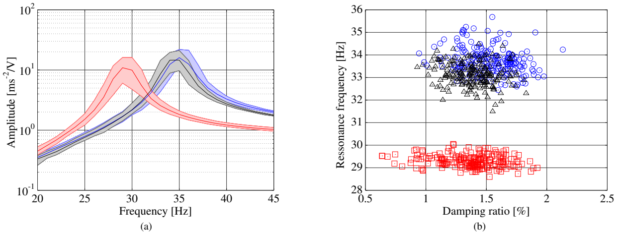
Figure 6. Variation of the data measured. (a) Frequency Response Function, where the continuous lines represent the mean values and the color zones the curves obtained with 99% of confidence, ■ - reference, ■ - damage I and ■ - damage II. (b) Variation of linear modal parameters, where ○ represents the reference condition, △ damage I and □ damage II.
