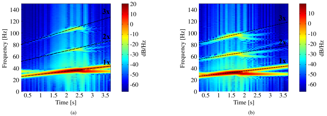
Figure 5. Time-frequency diagram of the system response obtained in damaged conditions; (a) damage I and (b) damage II.
