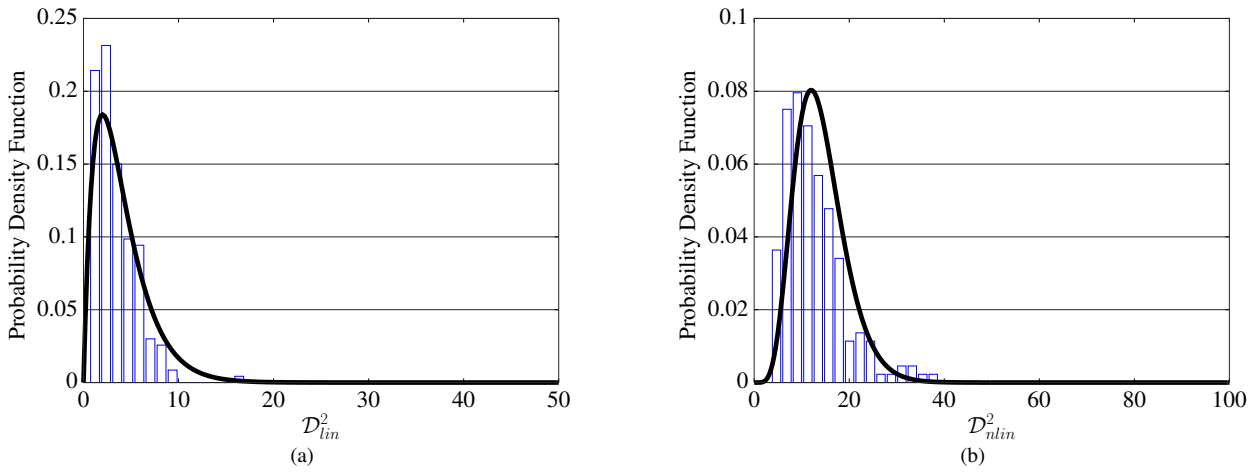
Figure 8. Comparison between the theoretical and experimental distributions. (a) Distance calculated based on the linear index in the reference condition. (b) Distance calculated based on the nonlinear index in the reference condition. The histogram represents the experimental data and the black line represents the theoretical chi-square distribution.
