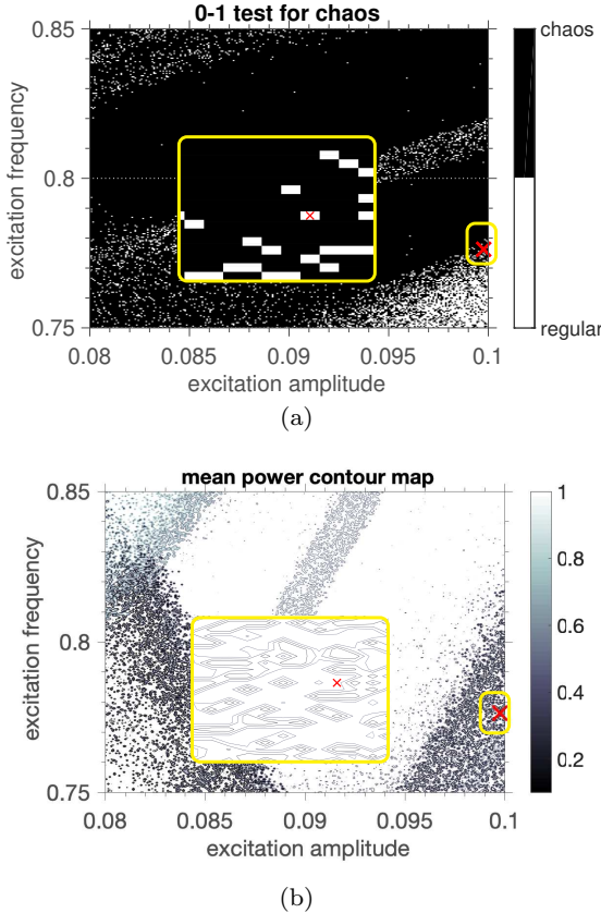
Figure 7 Noisy case contour maps: (a) constraint function defined by the 0-1 test for chaos, and (b) noisy objective function defined by the mean output power.
