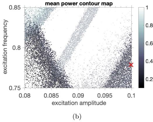
Figure 4 Bi-dimensional case contour maps: (a) constraint function defined by the 0-1 test for chaos, and (b) normalized objective function, defined by the mean output power.
