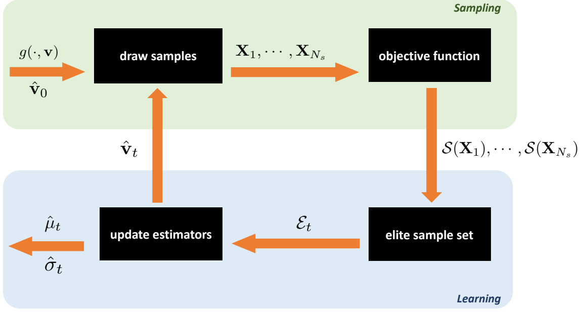
Figure 3 Schematic representation of the CE algorithm for optimization.
