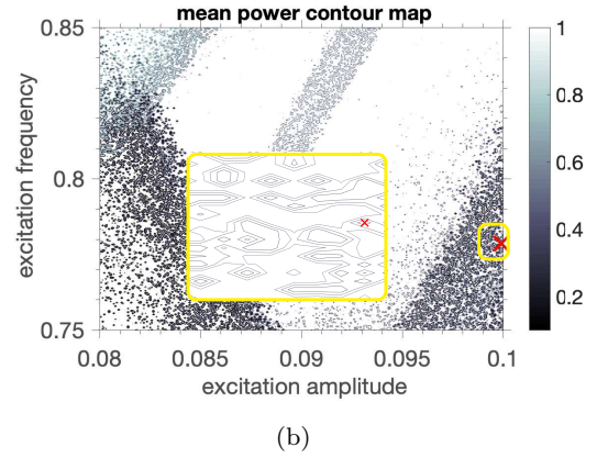
Figure 5 Magnification of the contour maps in bi-dimensional case: (a) constraint function defined by the 0-1 test for chaos, and (b) normalized objective function, defined by the mean output power.
