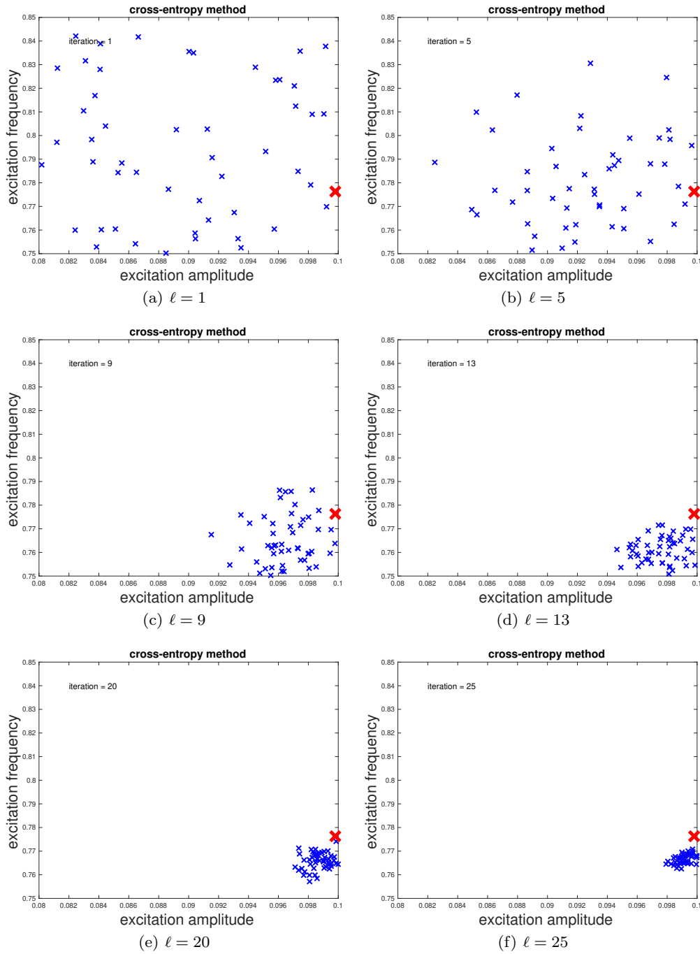
Figure 8 Illustration of CE method in the noisy case, using N^s = 50 samples, at different levels (iterations) of the algorithm. The noisy version of reference solution is indicated with a red cross.
