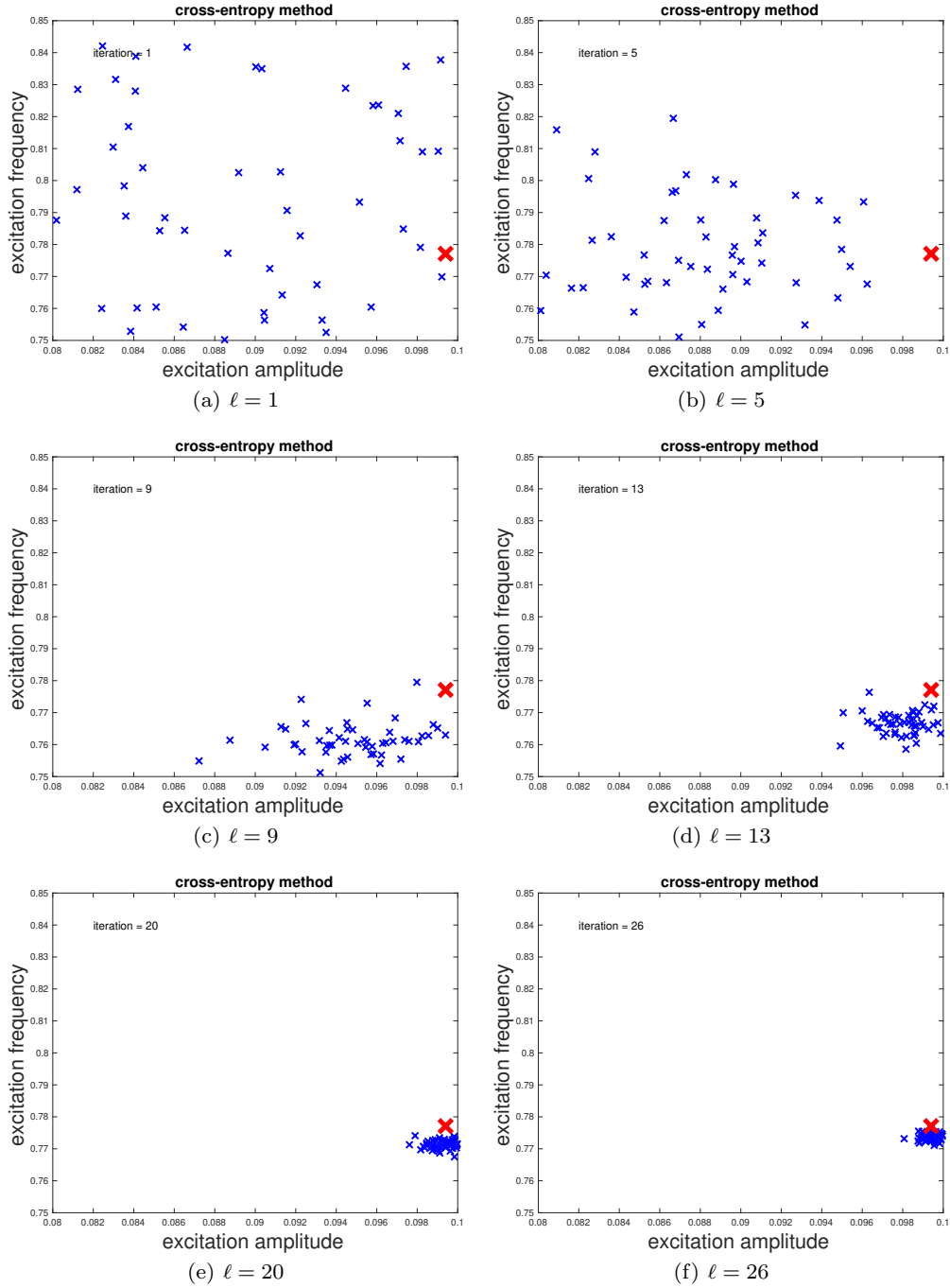
Figure 6 Illustration of CE method in the bi-dimensional case, using N^s = 50 samples, at different levels (iterations) of the algorithm. The reference solution is indicated with a red cross.
