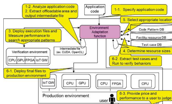
Fig. 1. Processing flow of environment-adaptive software.
