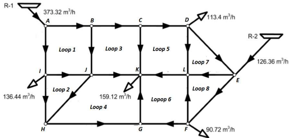
Figure 2. A pipe-network with 8 loops (adapted from Brkic [15])
