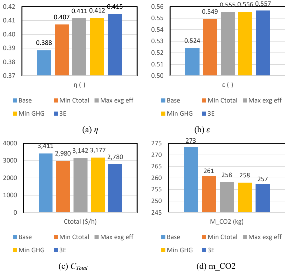
Figure 10. Comparison of the Solver-TOPSIS optimised solution and Solver's three single-objective solutions to the base-design values
