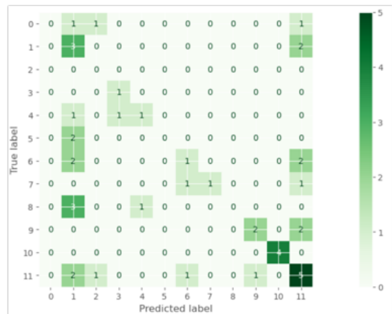
Figure 10: Confusion Matrix of Decision Tree
