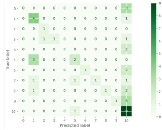
Figure 9: Confusion Matrix of Random Forest Classifier
