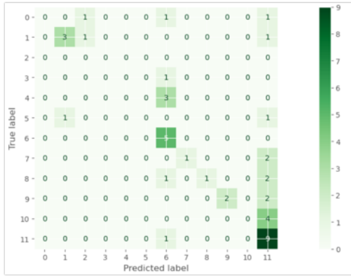
Figure 7: Confusion Matrix of Logistic Regression
