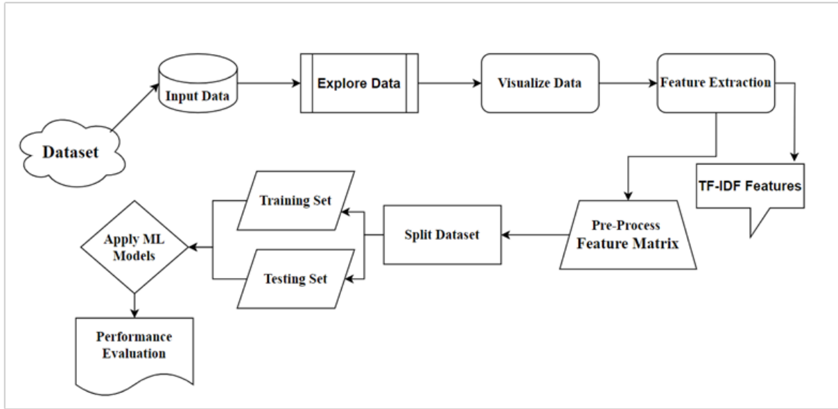
Figure 1: Proposed methodology illustration with step-by-step process of taxonomy classification
