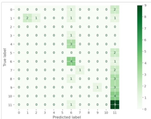
Figure 8: Confusion Matrix of Support Vector Machine
